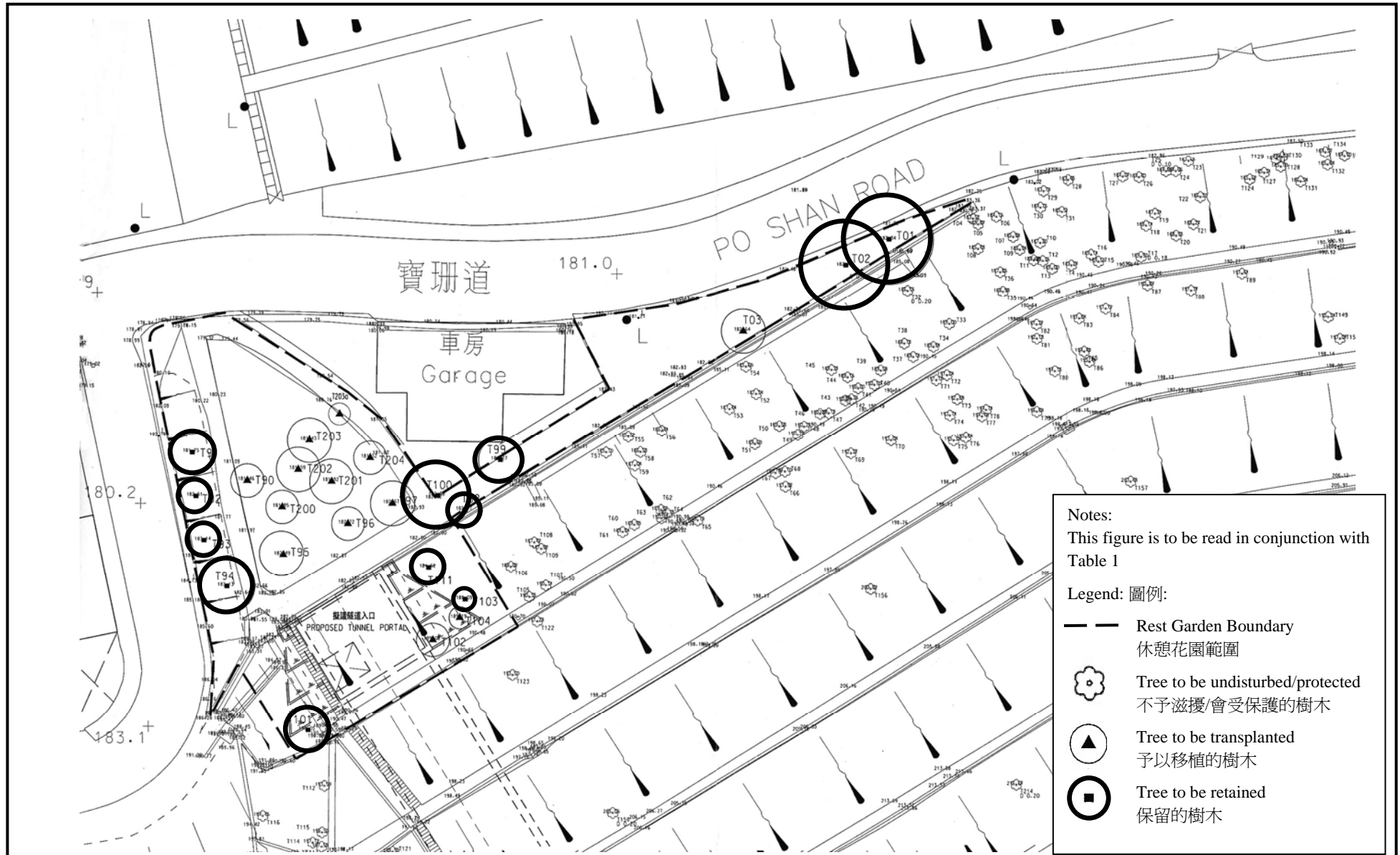
Figure 4: Indicative Tree Transplantation Plan for Rest garden 圖 4: 休憩花園樹木移植示意圖
