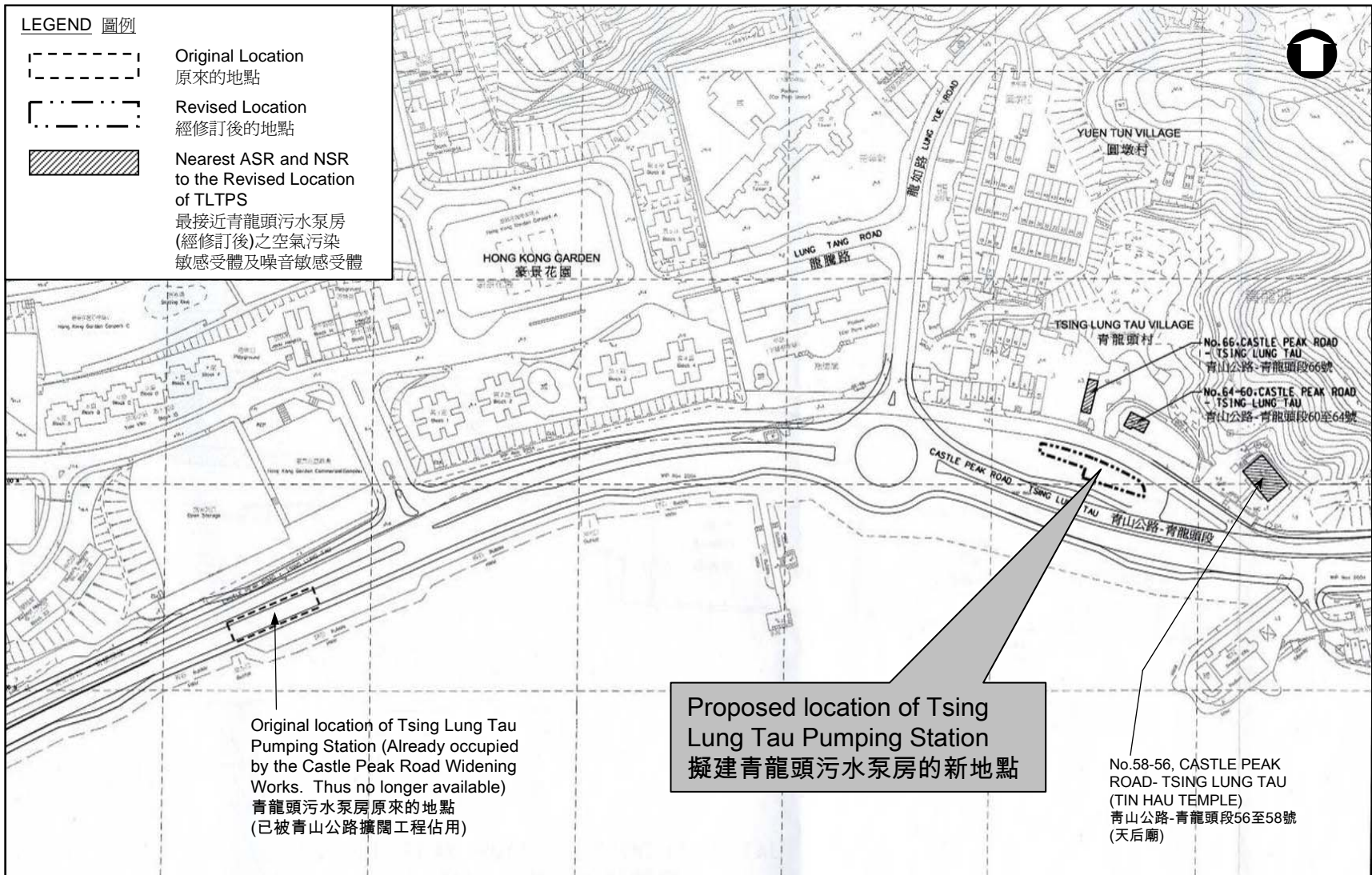
Figure 1 : Location Plan of the Proposed Tsing Lung Tau Pumping Station 圖 1: 擬建青龍頭污水泵房位置圖
