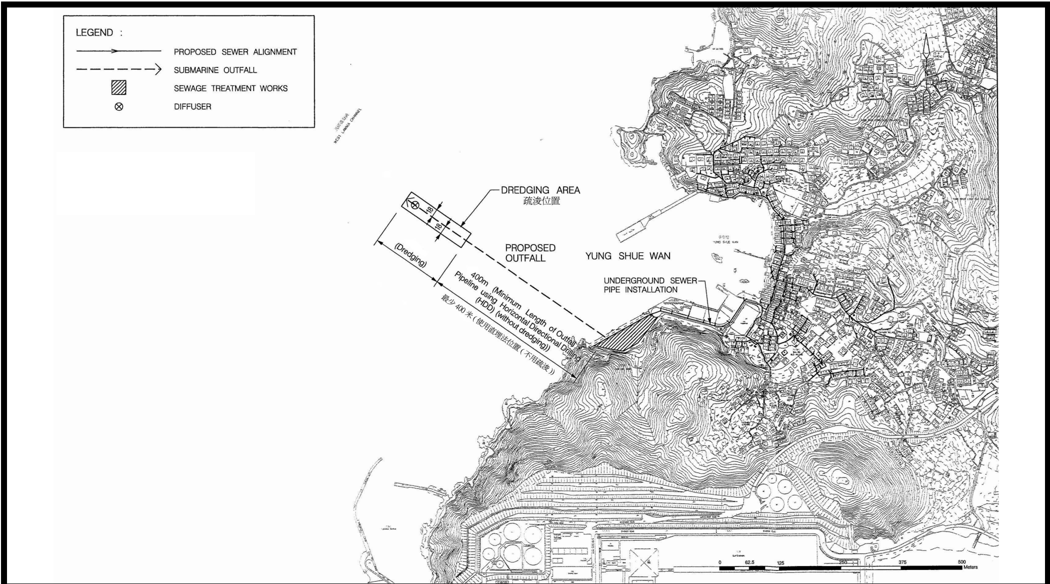
Figure 2: Locations of Horizontal Directional Drilling and Dredging
