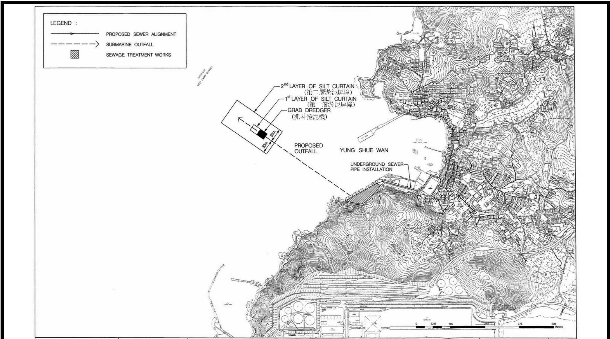
Figure. 4: Arrangement of Silt Curtain during Construction
