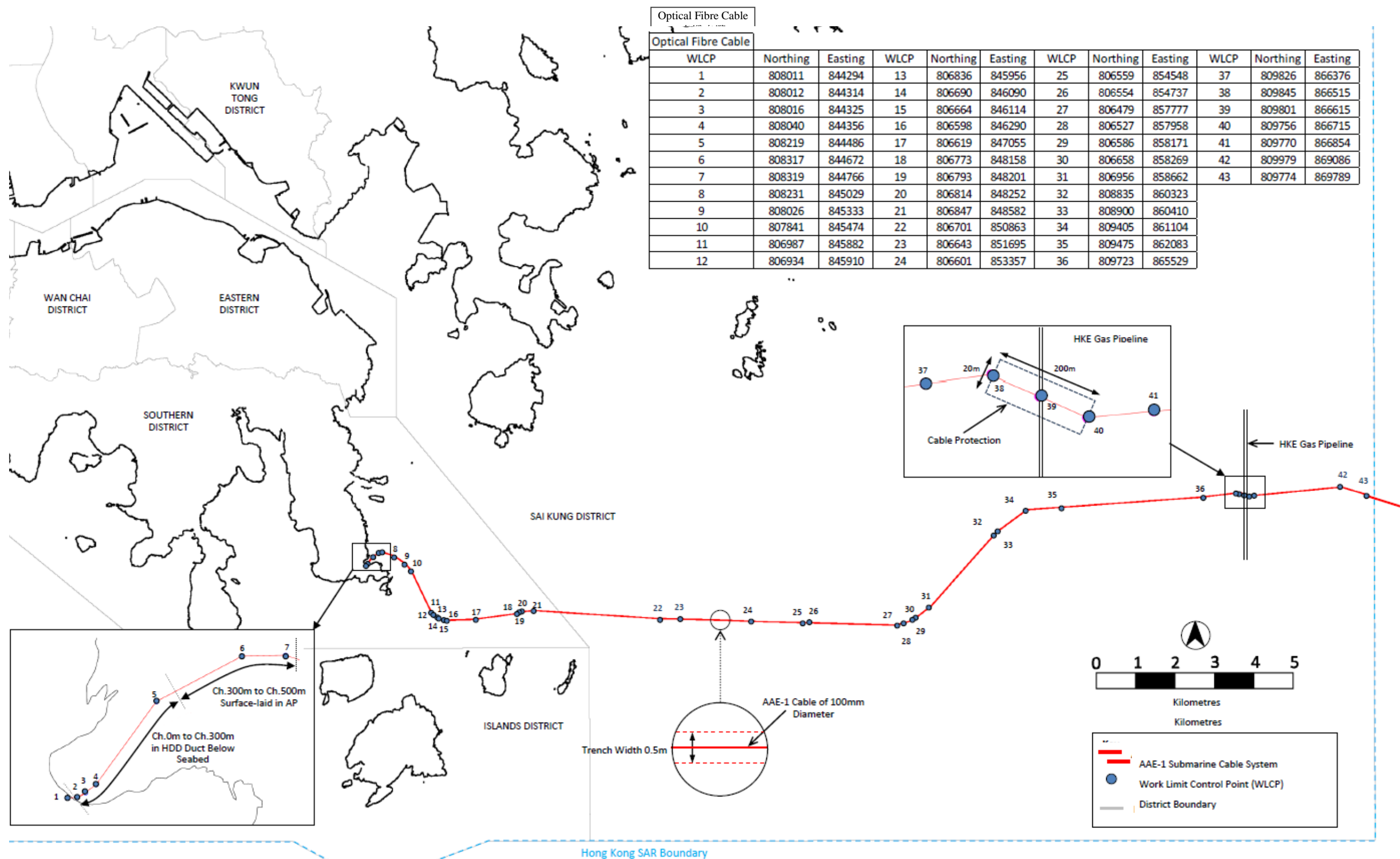
Figure 1: The landing site and the route alignment of the cable 圖 1: 光纜系統登岸地點及海上路線
