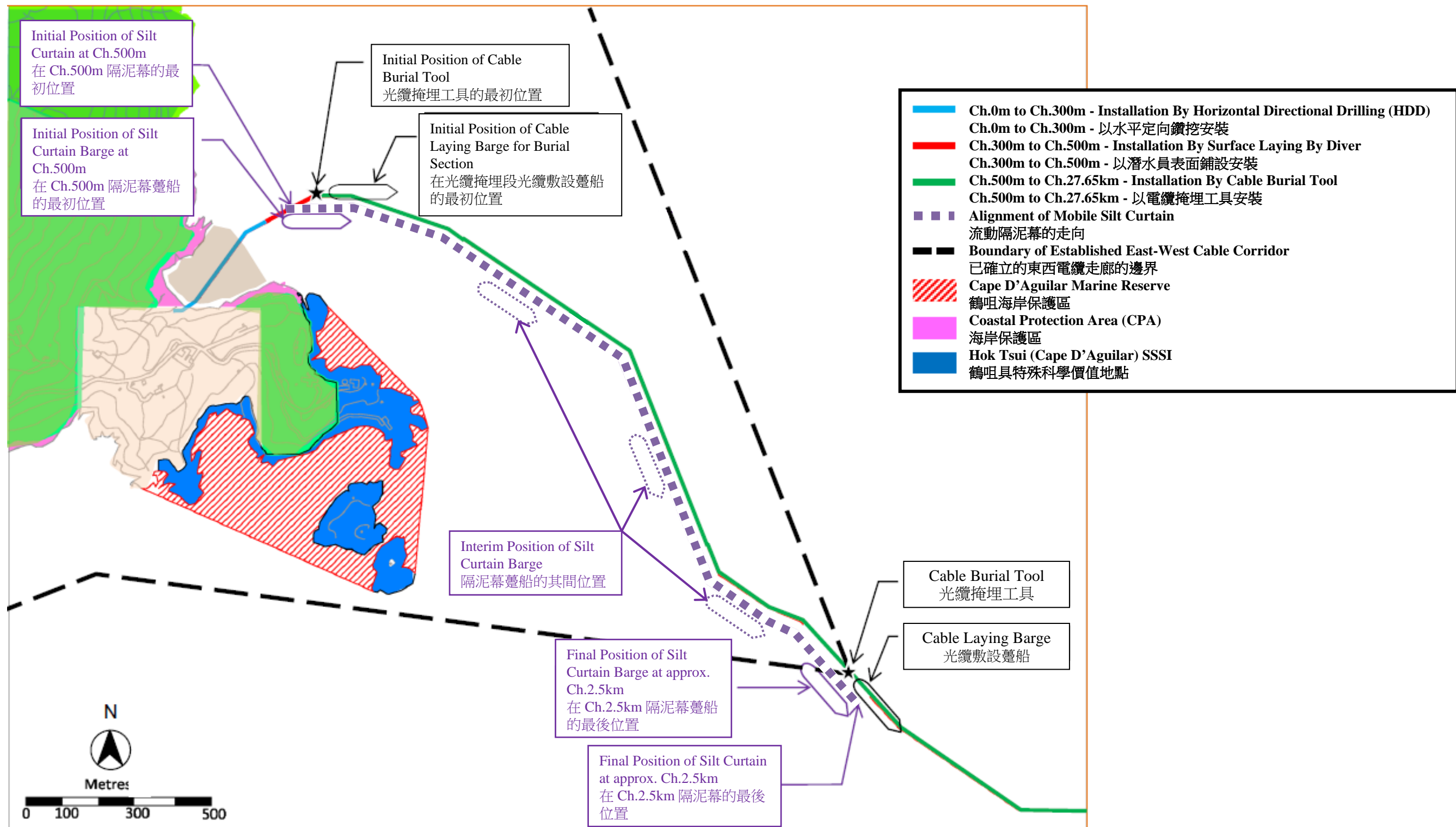
Figure 2: Installation method and the indicative location of the silt curtain 圖 2: 光纜系統的安裝方法及隔泥幕位置指示圖
