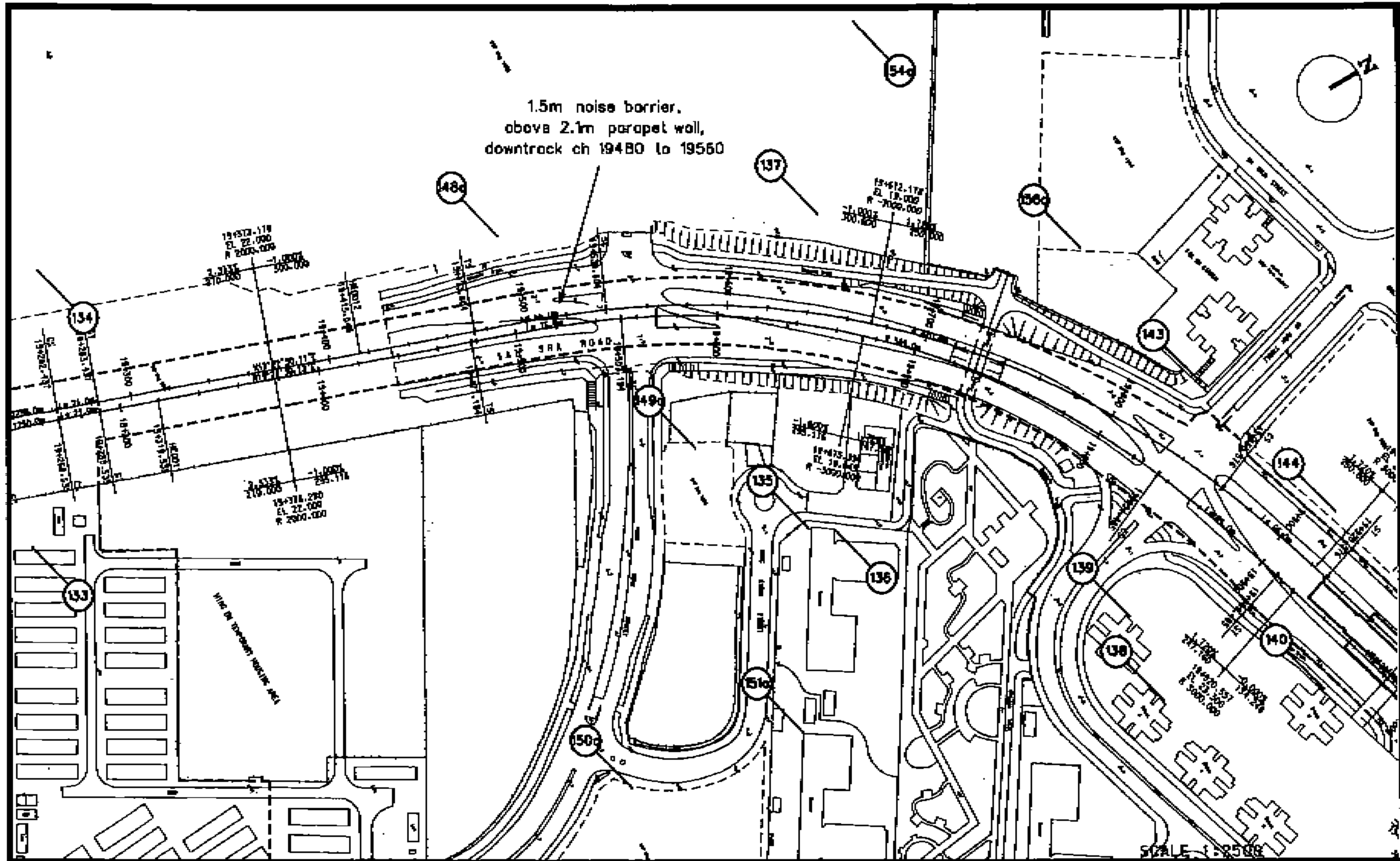
Figure 9 Noise Barriers and Enclosures (Extracted from Technical Annex F1 of the EIA Report)
