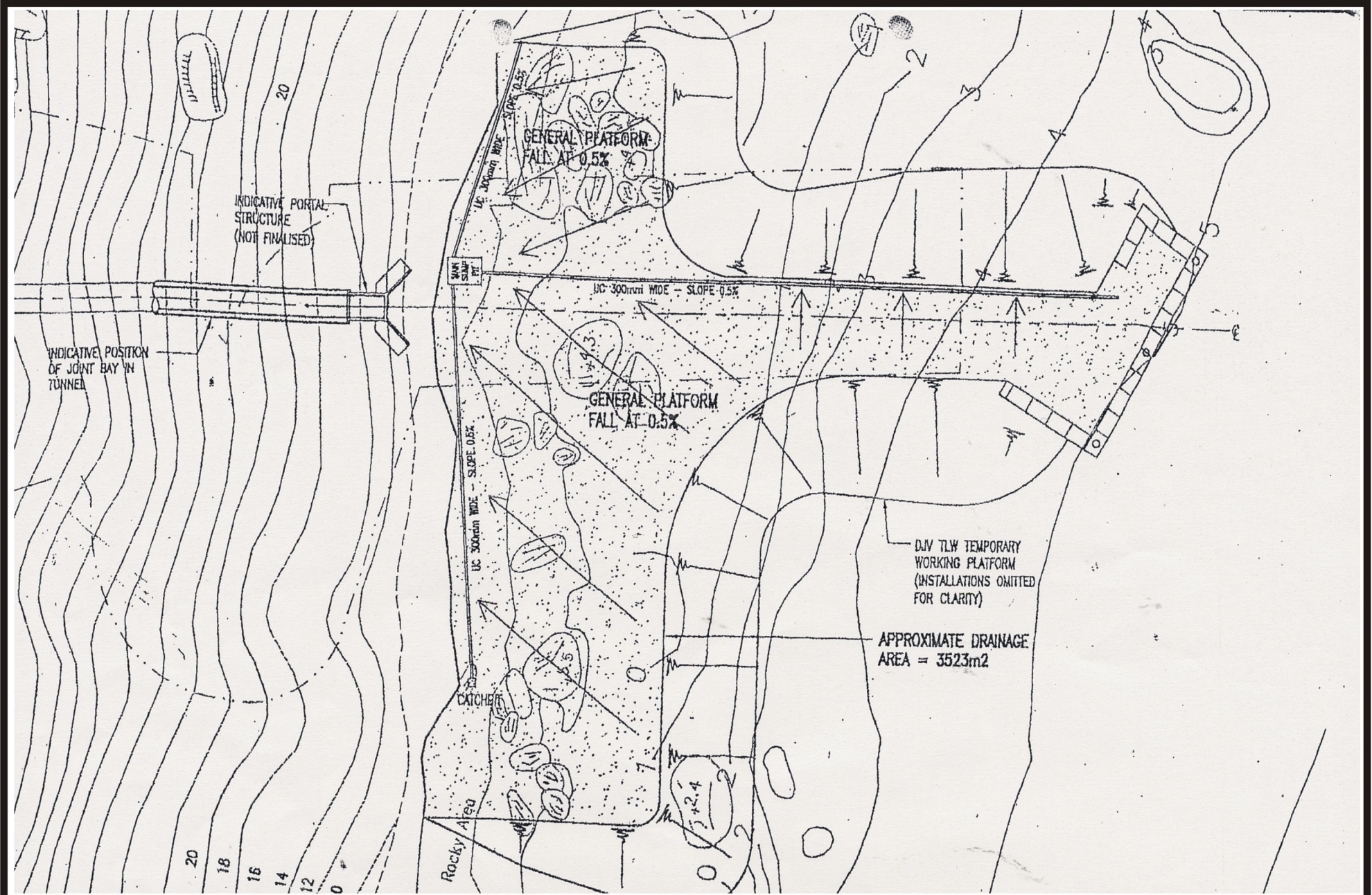
Schematic Layout of Construction Site Drainage System at Tai Long Wan
