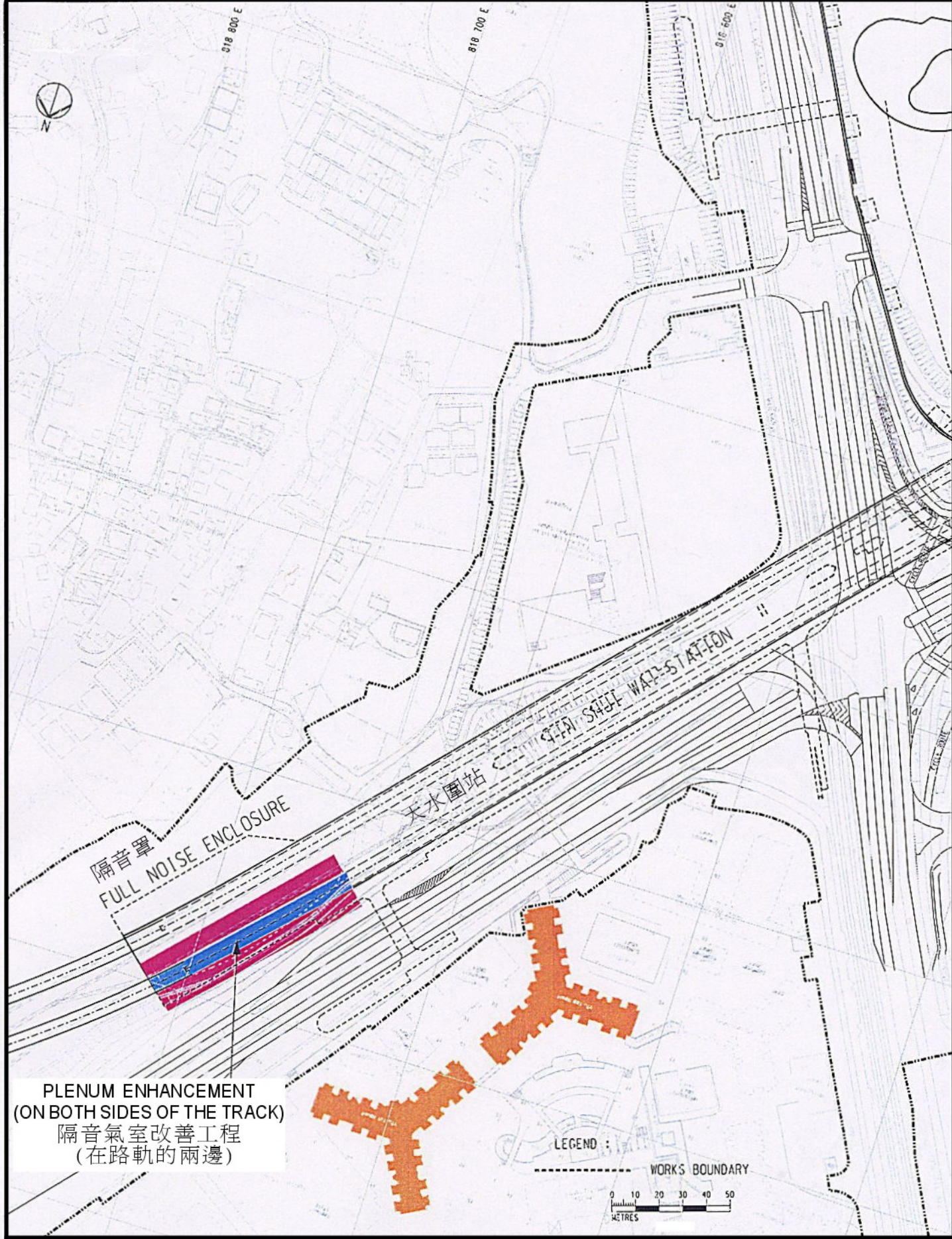
Figure 10 - Track Enclosure and Plenum Enhancement at the Tin Shui Wai Station
