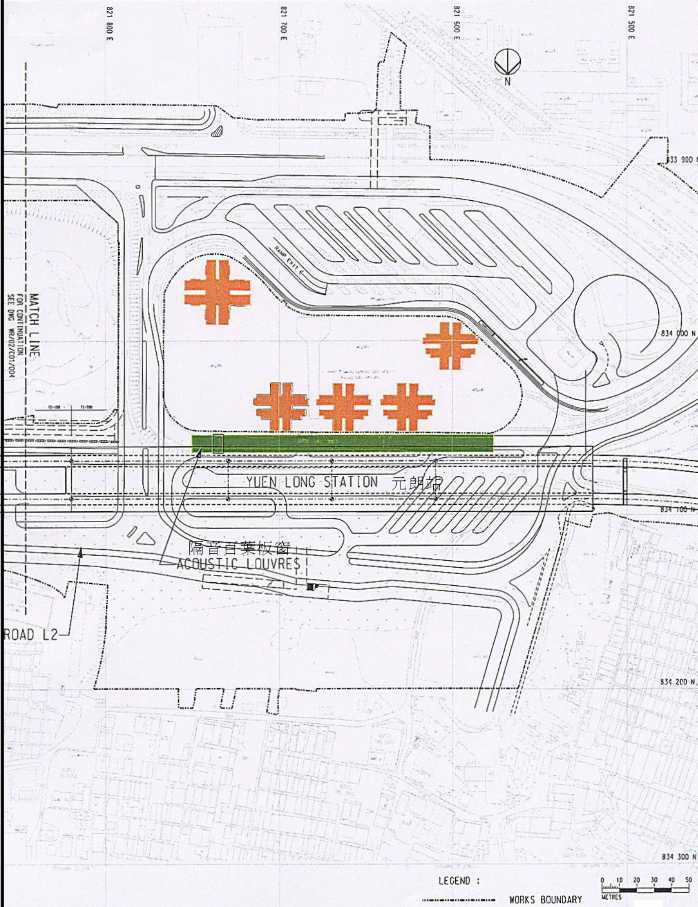
Figure 6 - Acoustic Louvers at the Yuen Long Station
