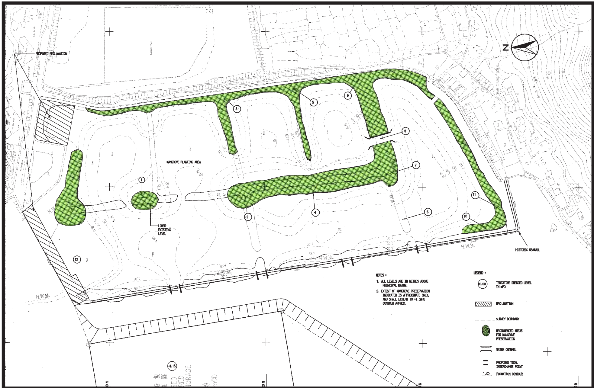
Figure 3 Mangrove Formation Plan
