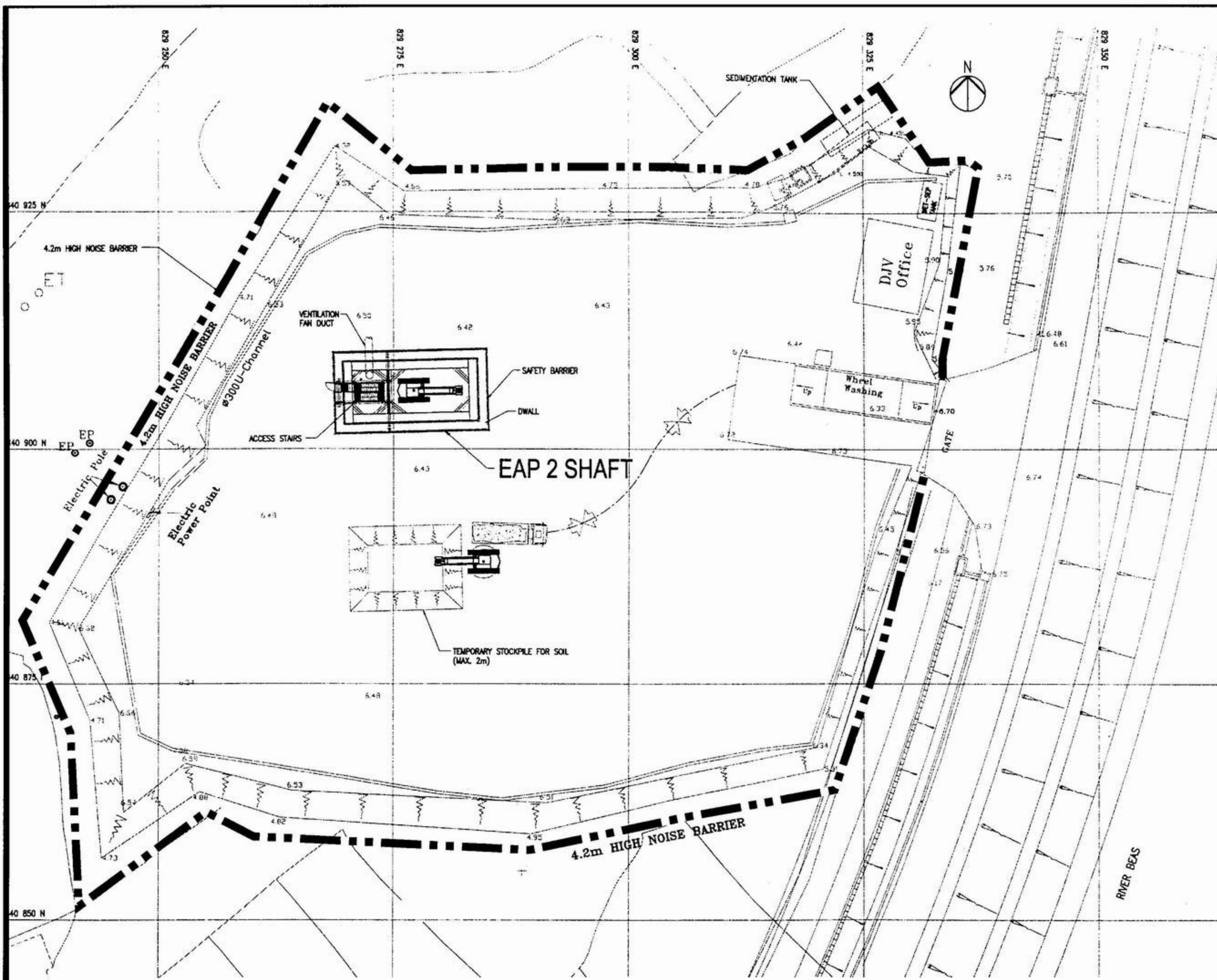
Figure 7b - Locations of Construction Phase Noise Barriers as described in Condition 3.17 of the Permit 圖七乙 - 條例3.17所指消除建築工程噪音之隔音屏障位置 Reproduced from Drawing No. LDB-201/001/92/C83/003 as submitted in Application No. VEP-130/2004 摘自申請書編號VEP-130/2004圖LDB-201/001/92/C83/003
