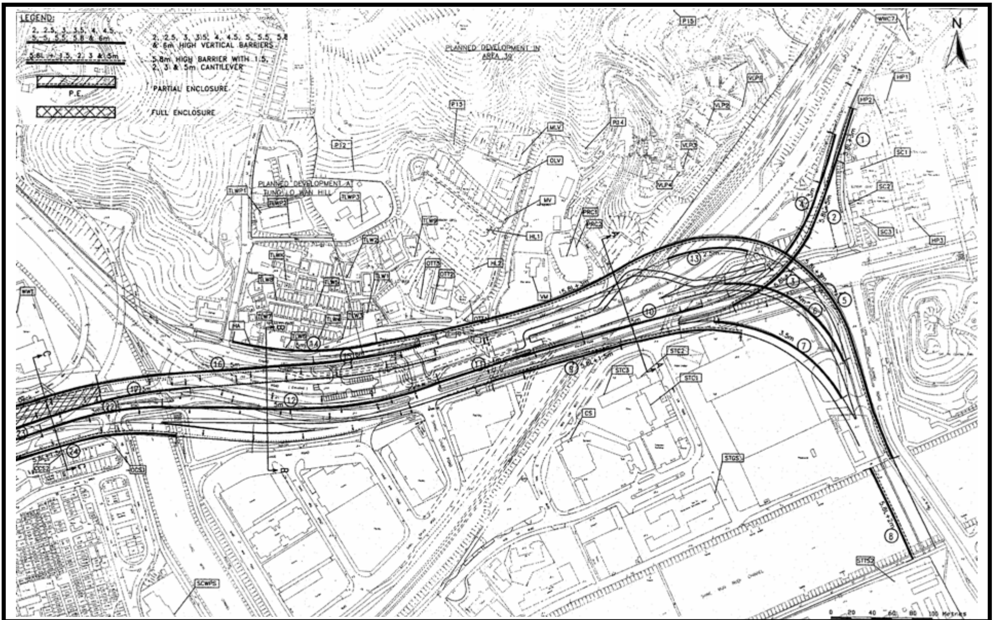
Figure 3 – Location of the Noise Barriers and Enclosures
