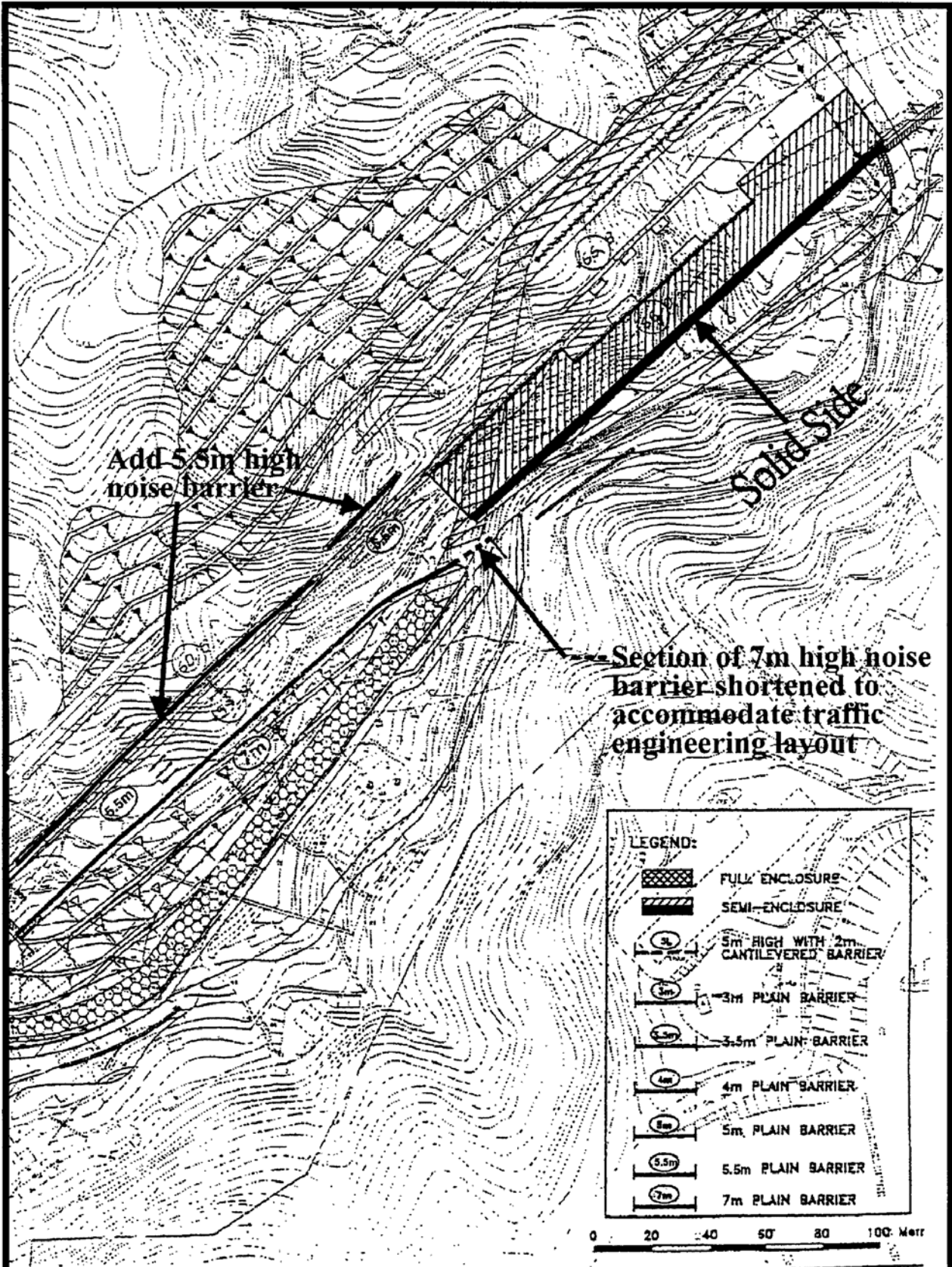
Figure 5 Noise Barriers and Enclosures (Extracted from the Application VEP-180/2005)
