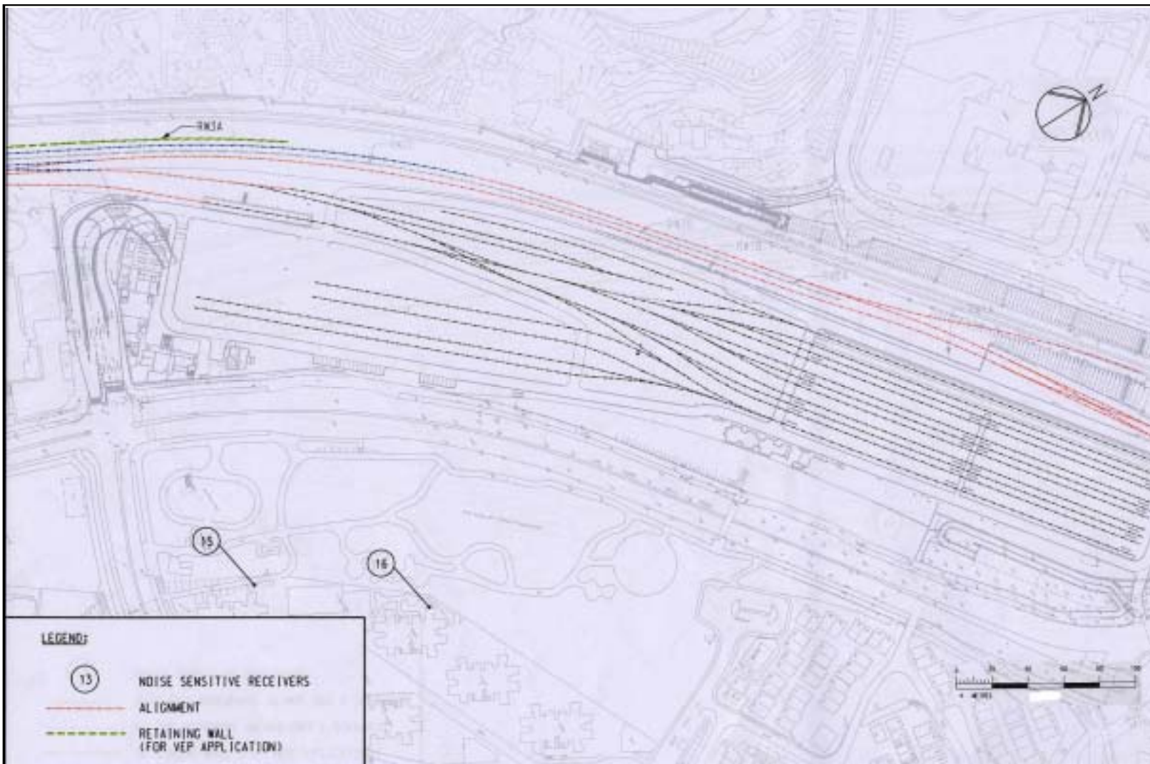
Figure 2 Retaining Walls (Extracted from the Application VEP-157/2004)
