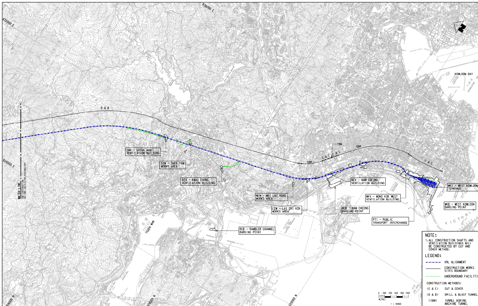
Figure 2: Overall View of Alignment & Works Sites (This figure was prepared based on Figure No. C8016/C/XRL/ENS/M50/002 of the Report submitted under Application No. VEP-346/2011)
