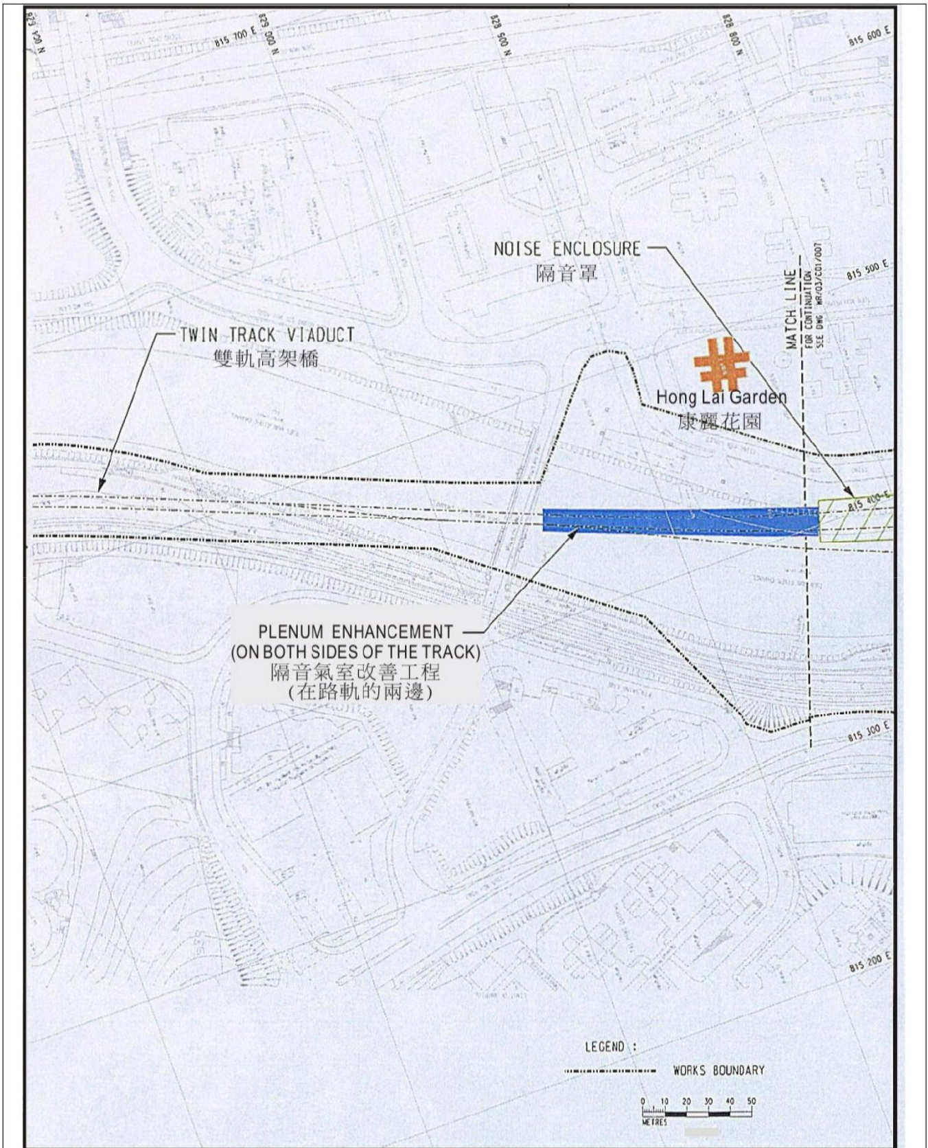
Figure 12– The Location of Plenum Enhancement along the Up and Down Tracks of the Viaduct near Hong Lai Garden
