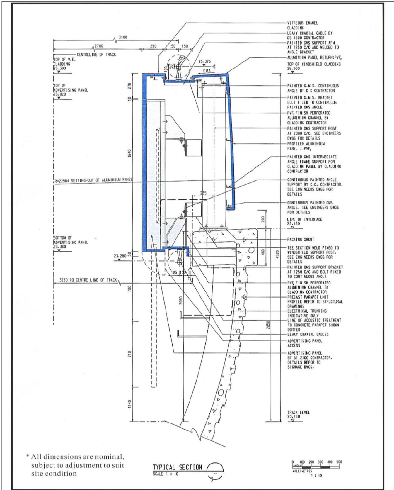
Figure 4 – Trackside Panels and Windshields at the Kam Sheung Road Station, Long Ping Station and Tin Shui Wai Station
