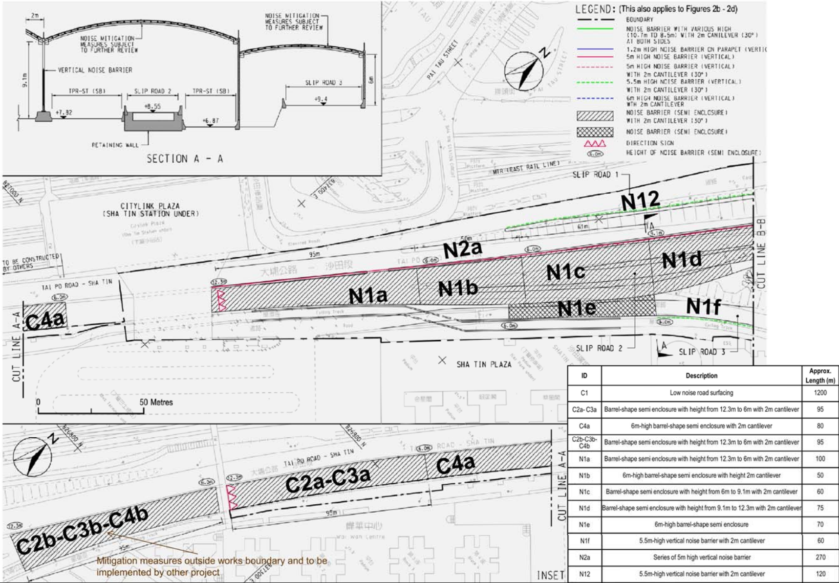
Figure 2a: Location of Noise Mitigation Measures (1 of 4)
