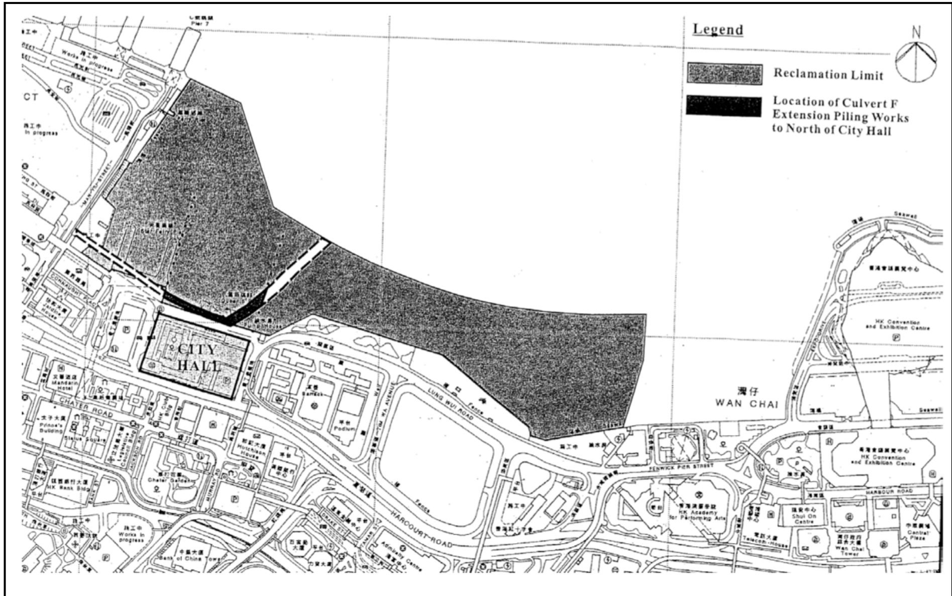
Figure 10: Locations of Culvert F Extension Piling Works to North of City Hall Note: Locations of Culvert F Extension Piling Works to North of City Hall Modified from Figure 4.2 of Volume 1 of the EIA Report
