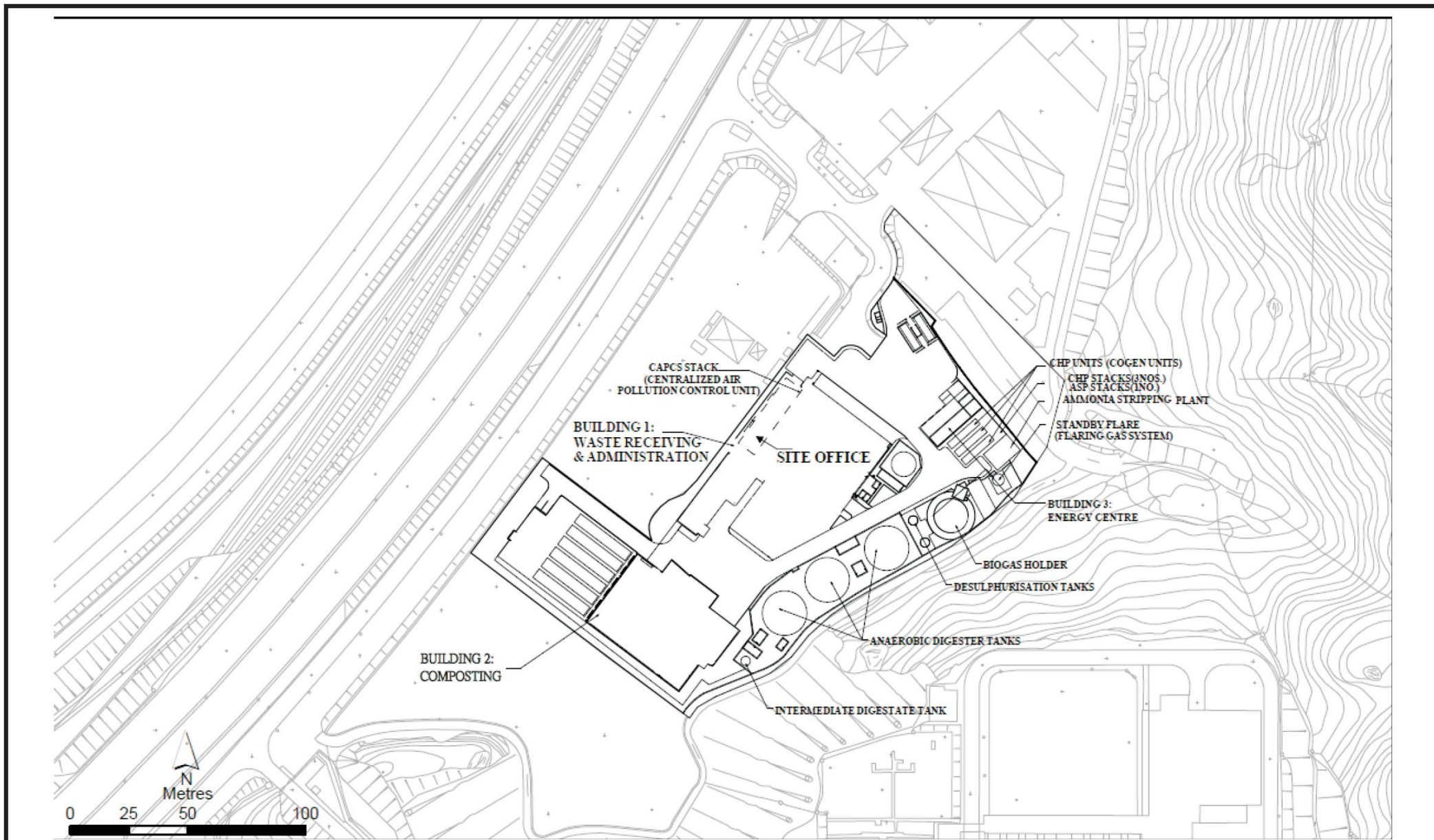
Figure 3 - Site Layout
