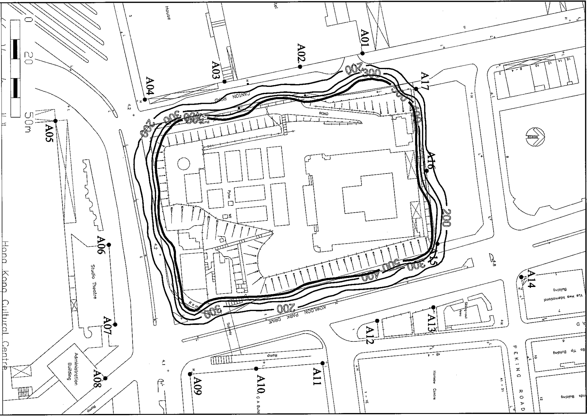
Title: Predicted Cumulative Hourly TSP Concentration Contour with Background Concentration at 5m above ground for Fugitive Dust Impact Assessment
