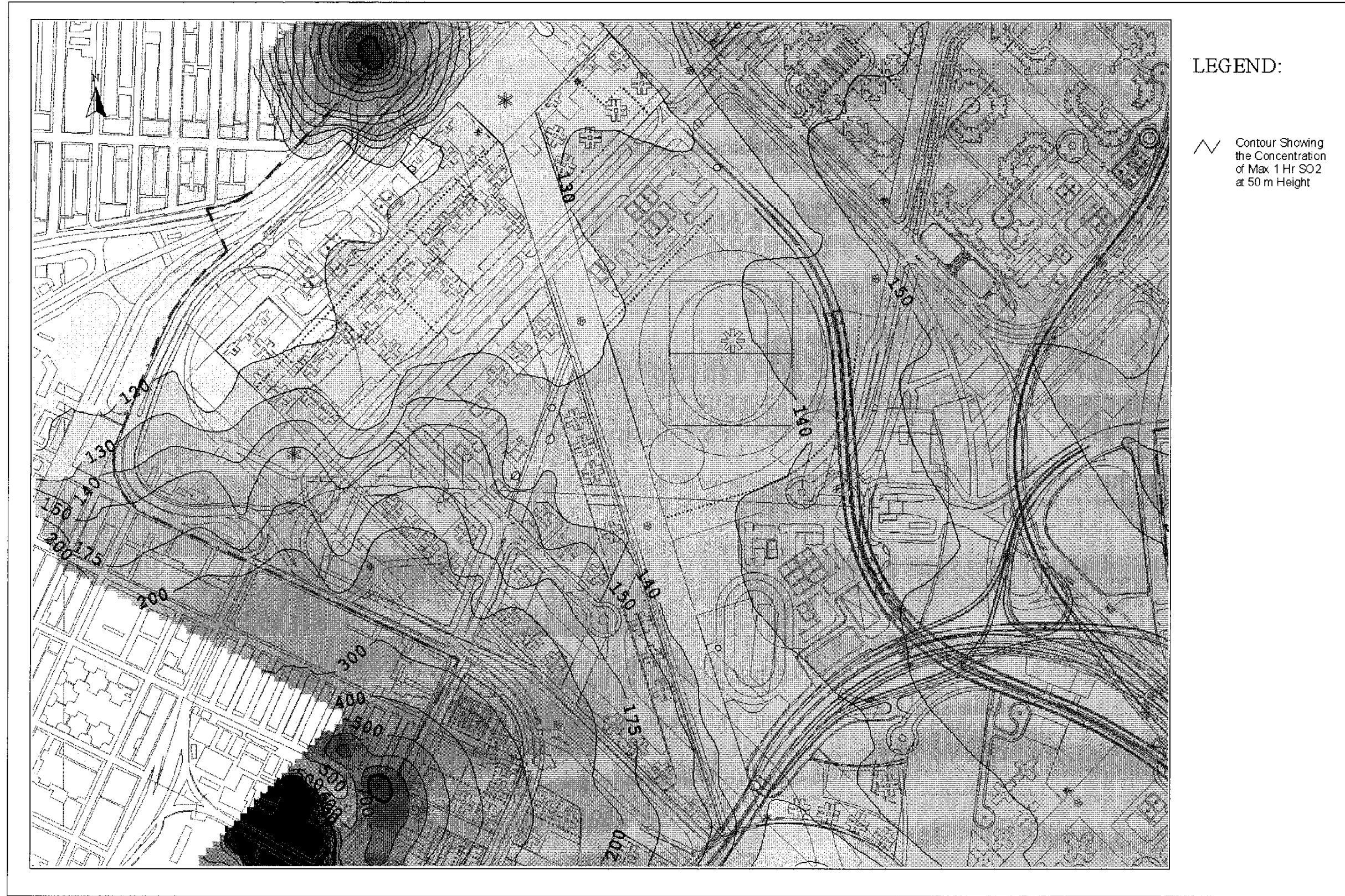
Drawing No. 22936/EN/330B Predicted Worst-case 1-hr Average SO 2 Concentration Contours at 50m Above Ground
