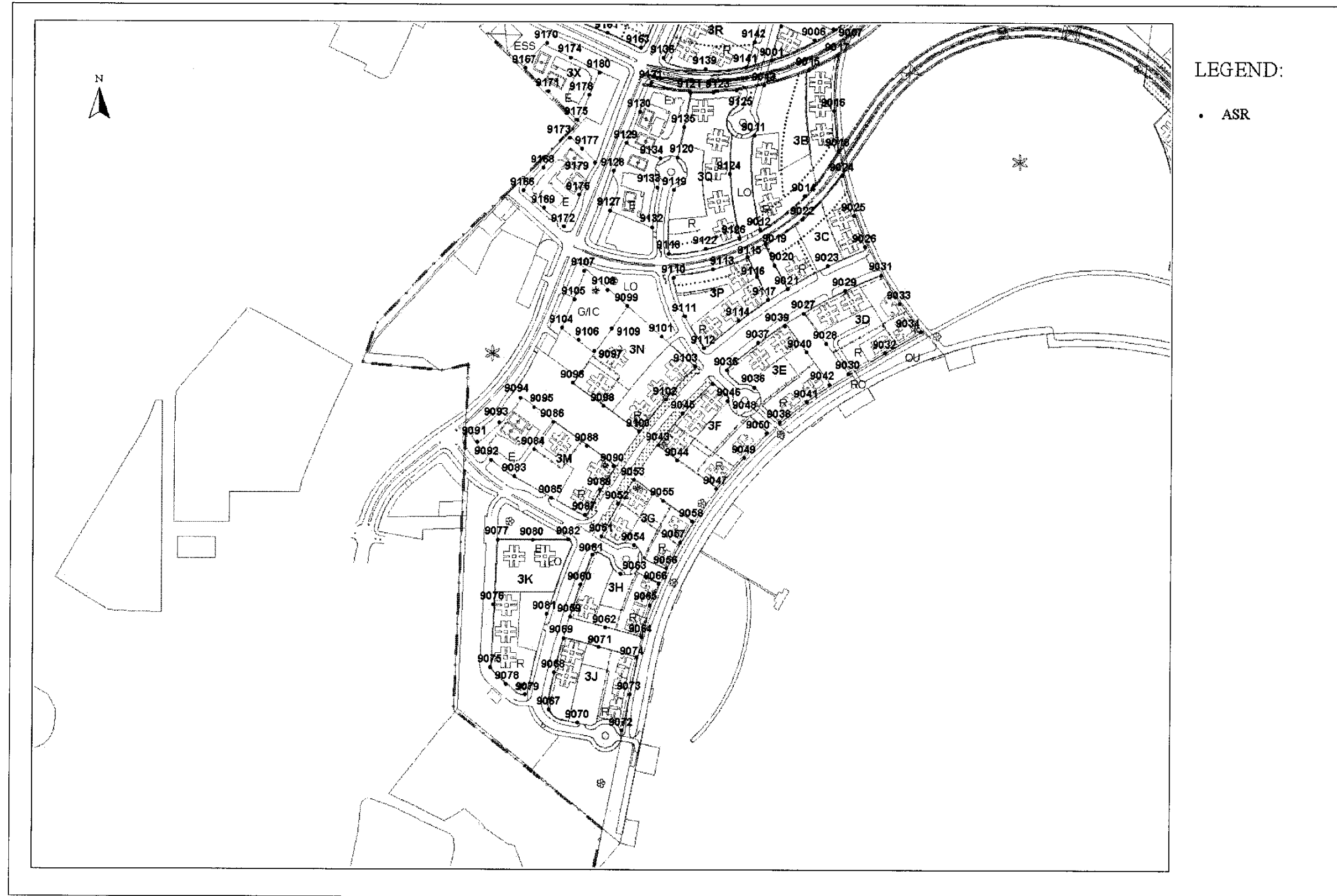
Drawing No. 22936/EN/337D Locations of Air Quality Assessment Points (Sheet 4 of 6)
