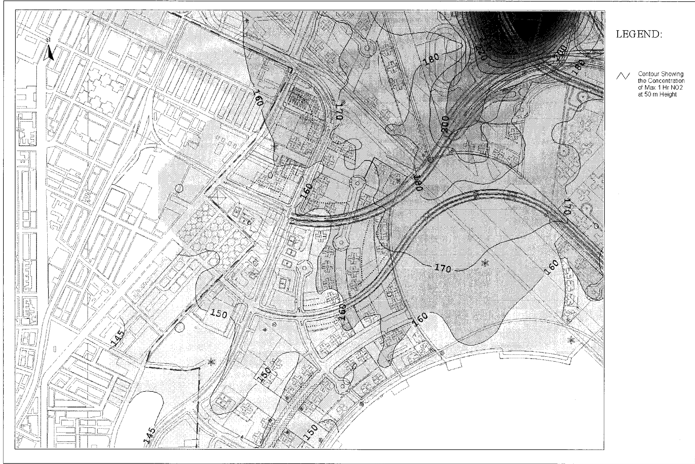
Drawing No. 22936/EN/319C Predicted Worst-case 1-hr Average NO 2 Concentration Contours at 50m Above Ground
