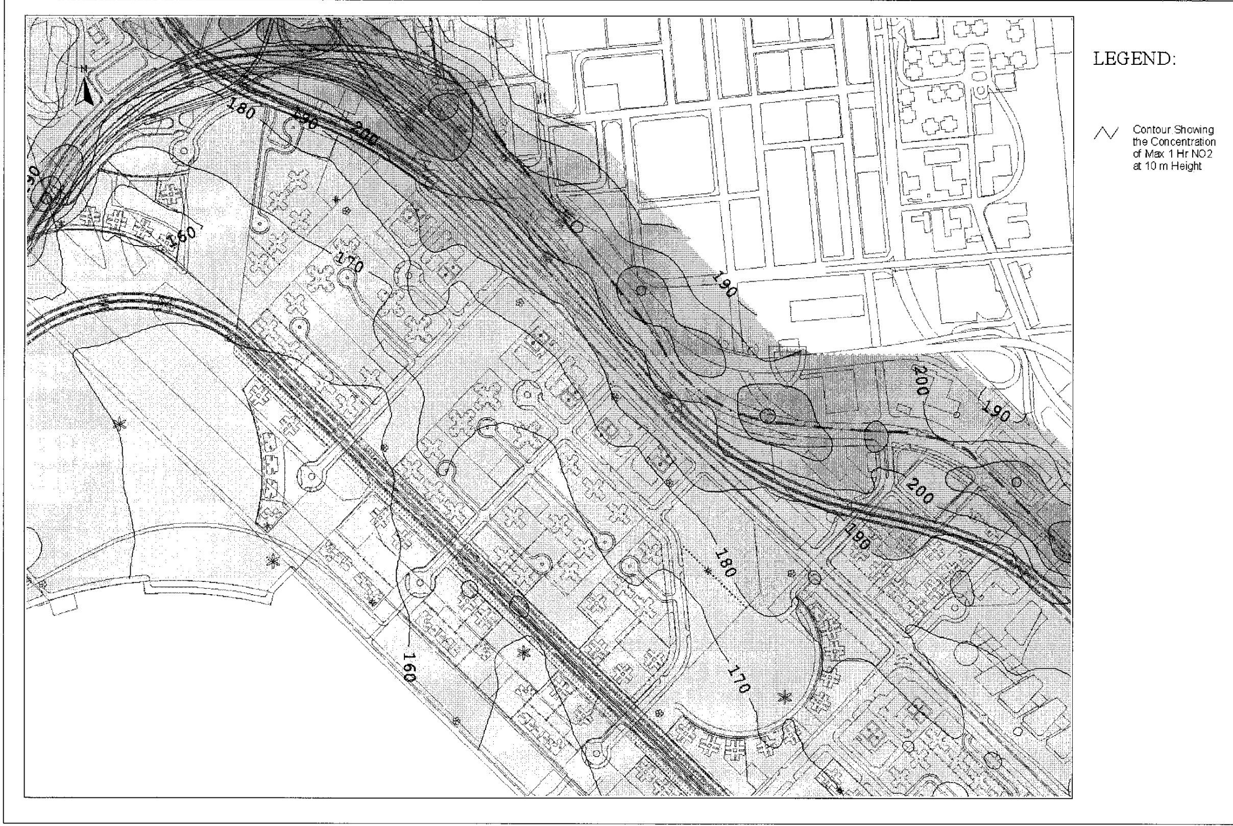
Drawing No. 22936/EN/317E Predicted Worst-case 1-hr Average NO 2 Concentration Contours at 10m Above Ground
