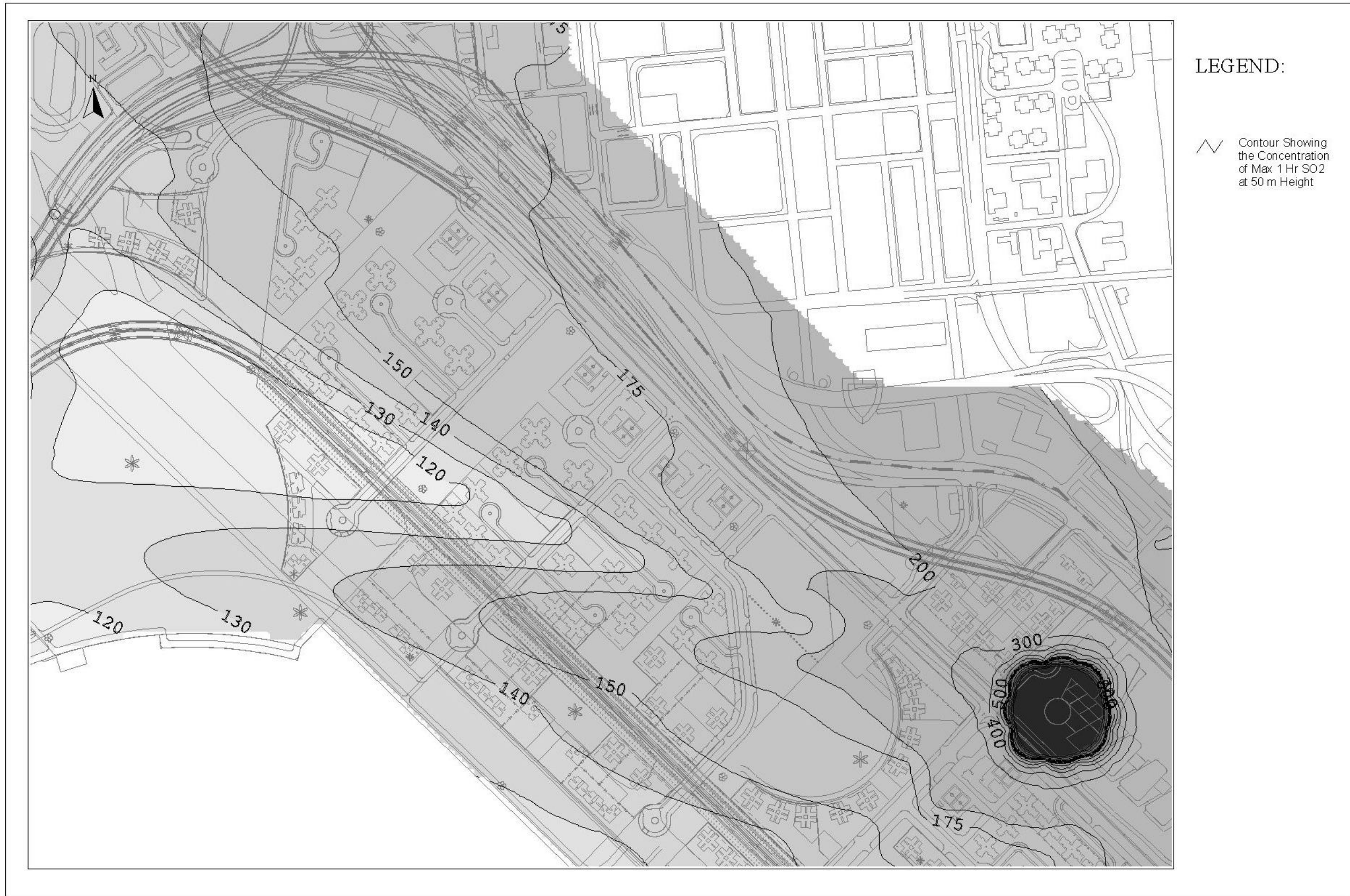
Drawing No. 22936/EN/330E Predicted Worst-case 1-hr Average SO2 Concentration Contours at 50m Above Ground
