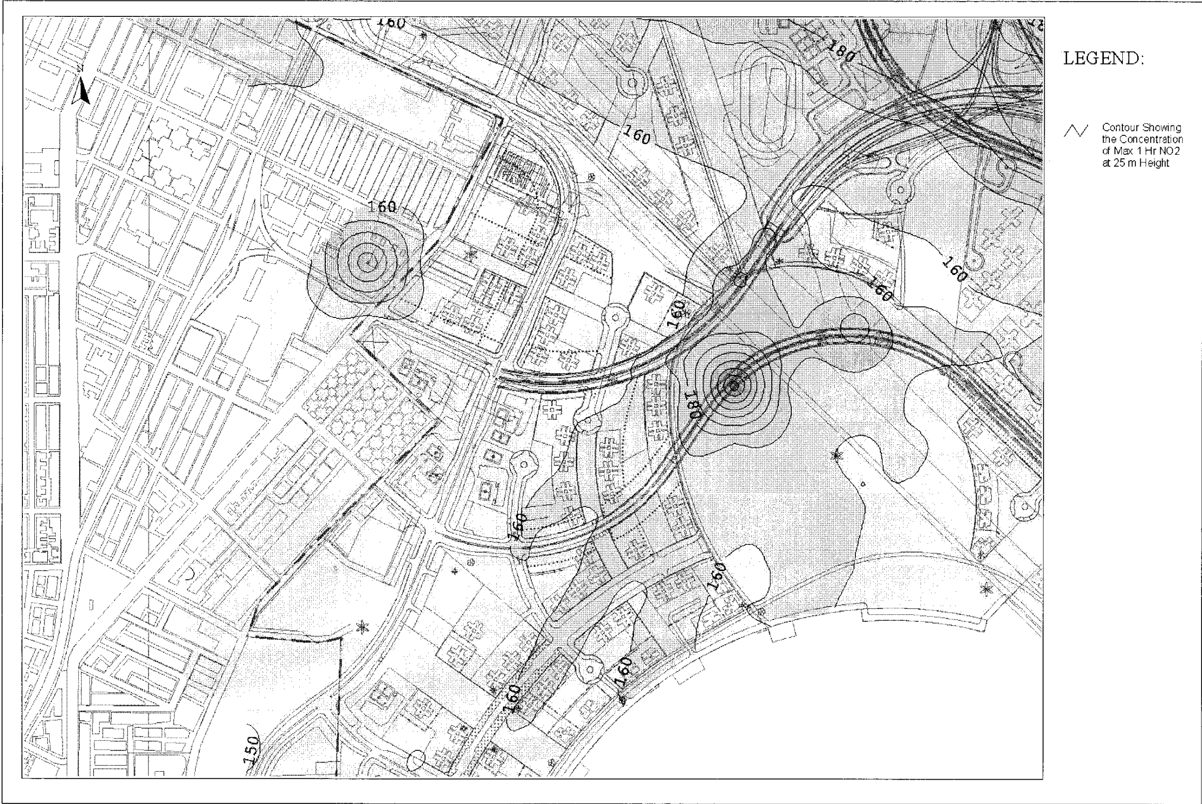
Drawing No. 22936/EN/318C Predicted Worst-case 1-hr Average NO 2 Concentration Contours at 25m Above Ground
