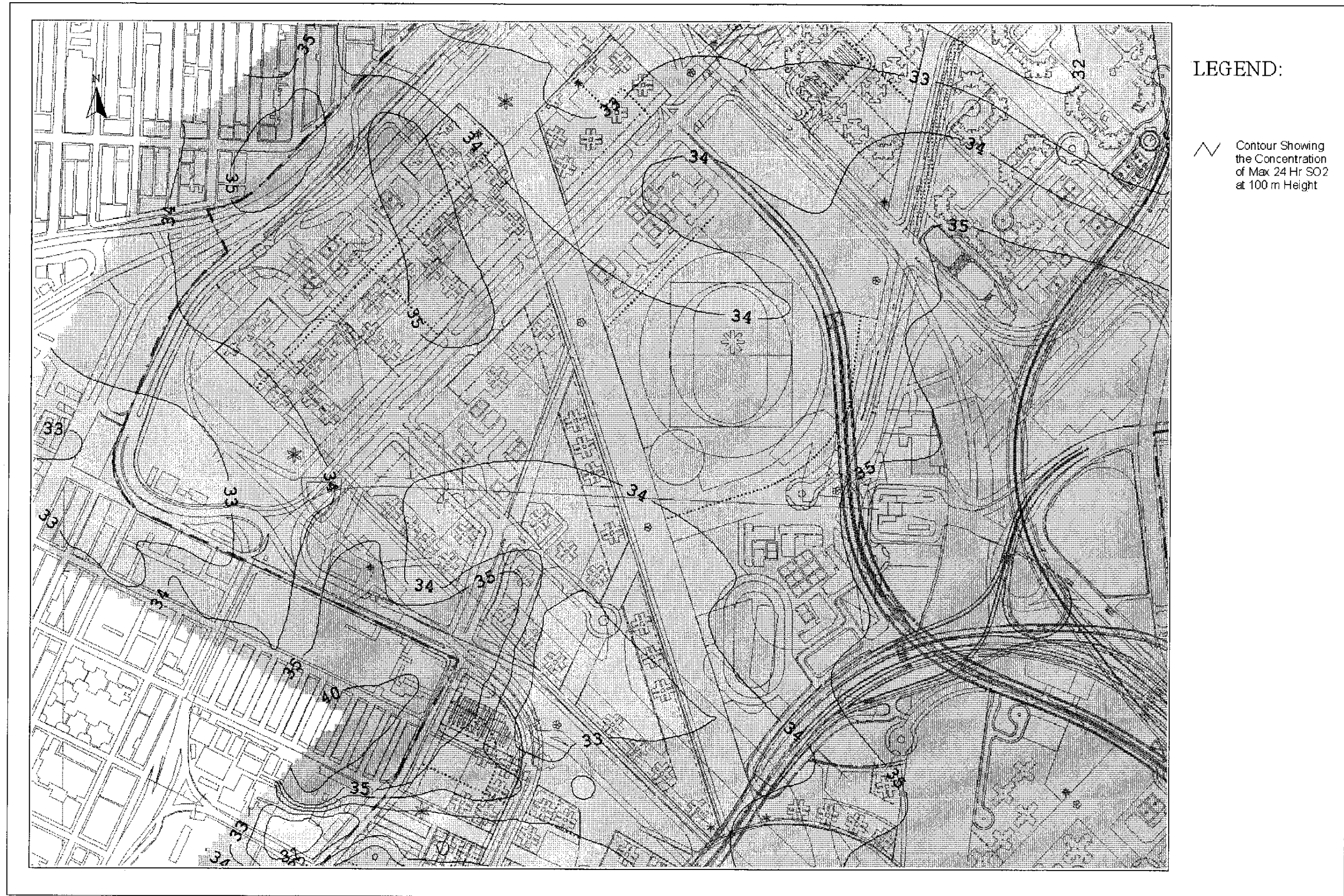
Drawing No. 22936/EN/336B Predicted Worst-case 24-hr Average SO 2 Concentration Contours at 100m Above Ground
