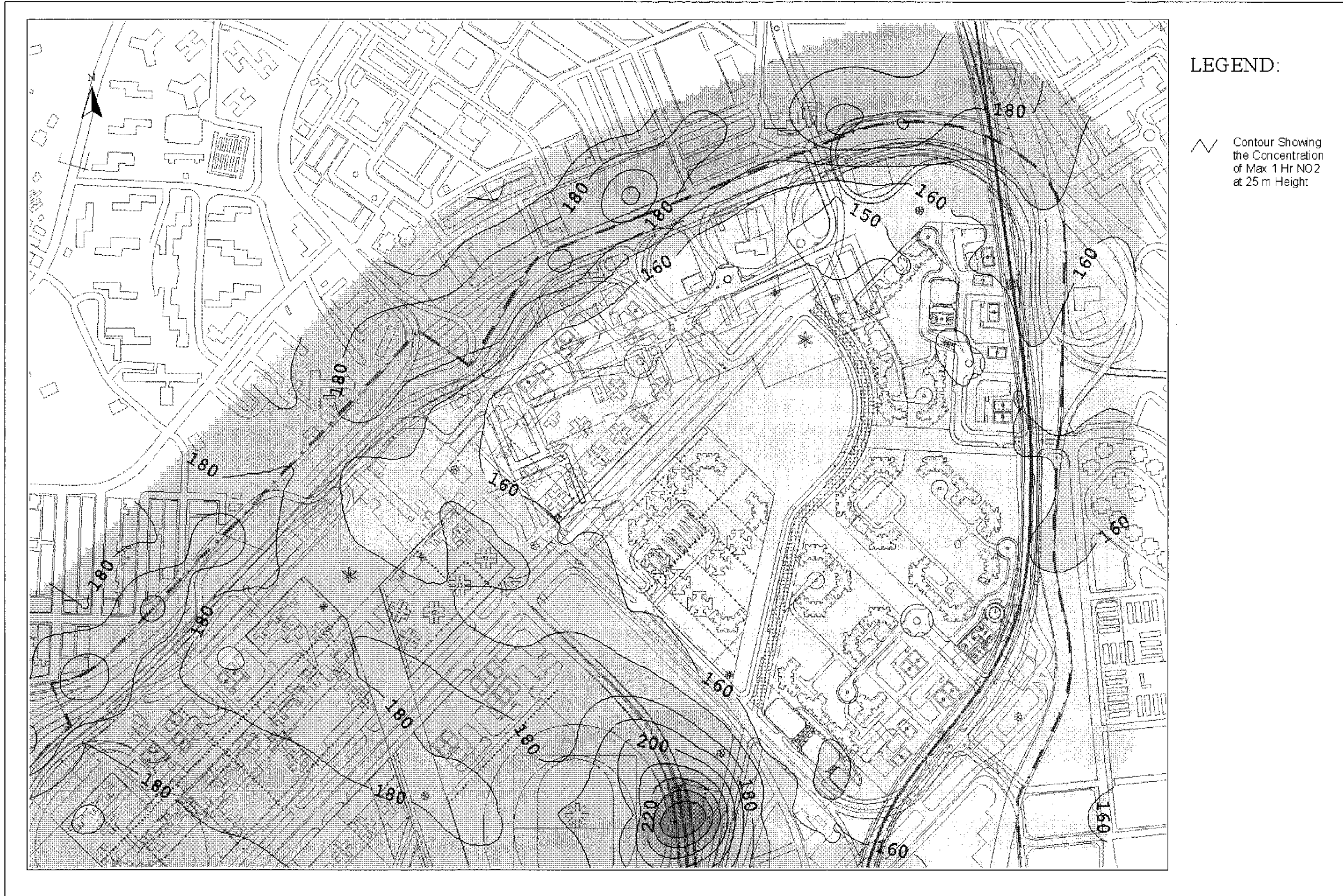
Drawing No. 22936/EN/318A Predicted Worst-case 1-hr Average NO 2 Concentration Contours at 25m Above Ground
