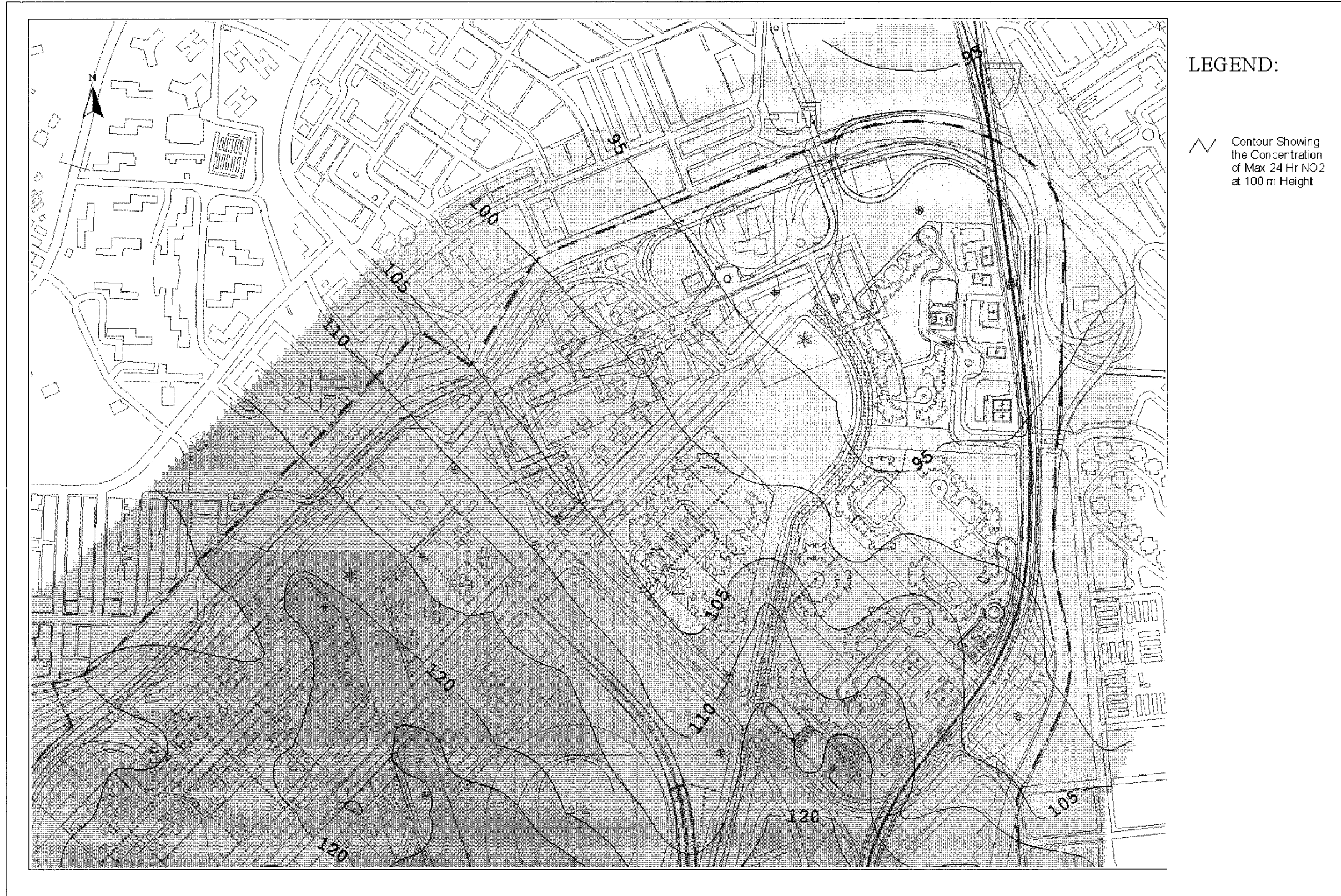
Drawing No. 22936/EN/327A Predicted Worst-case 24-hr Average NO 2 Concentration Contours at 100m Above Ground
