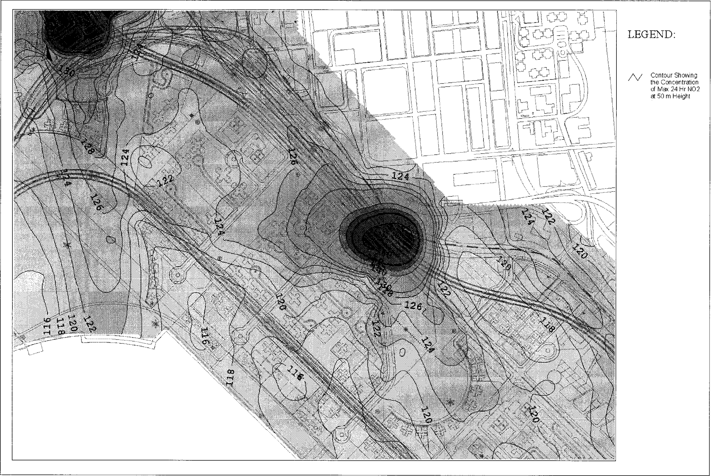
Drawing No. 22936/EN/325E Predicted Worst-case 24-hr Average NO 2 Concentration Contours at 50m Above Ground
