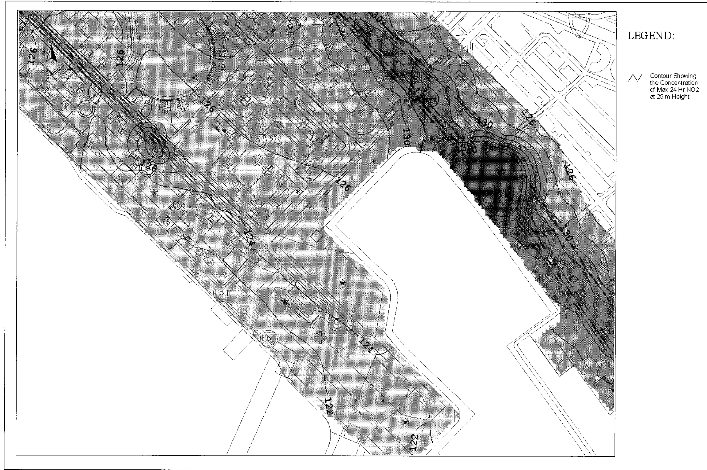
Drawing No. 22936/EN/324F Predicted Worst-case 24-hr Average NO 2 Concentration Contours at 25m Above Ground
