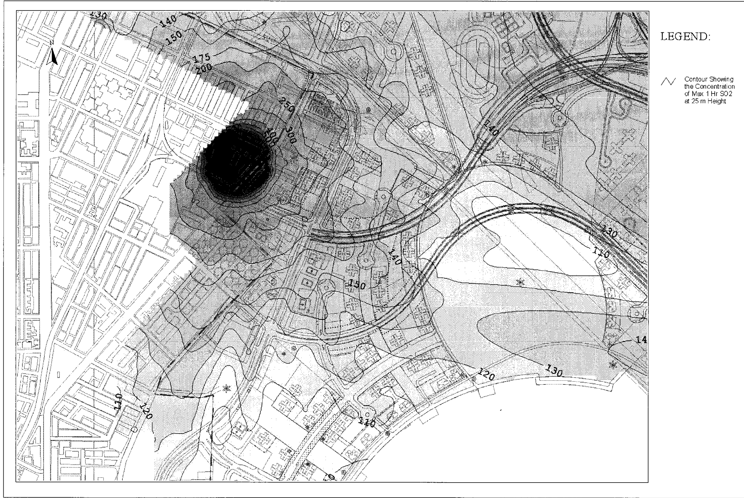
Drawing No. 22936/EN/329C Predicted Worst-case 1-hr Average SO 2 Concentration Contours at 25m Above Ground
