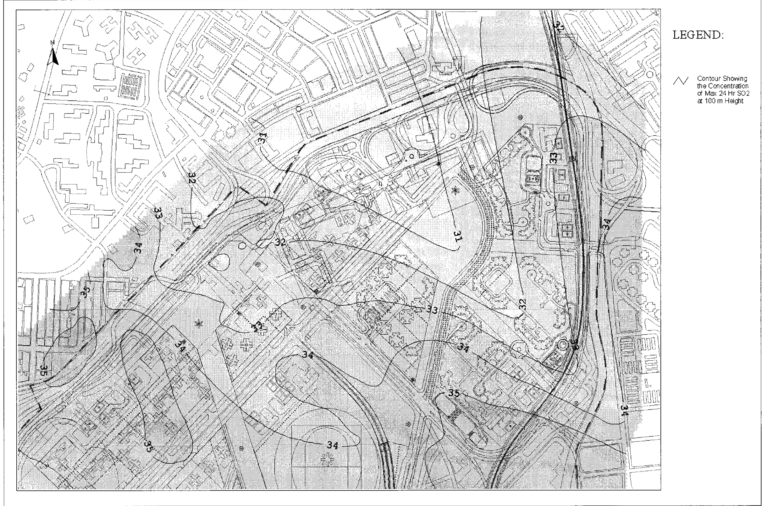
Drawing No. 22936/EN/336A Predicted Worst-case 24-hr Average SO 2 Concentration Contours at 100m Above Ground
