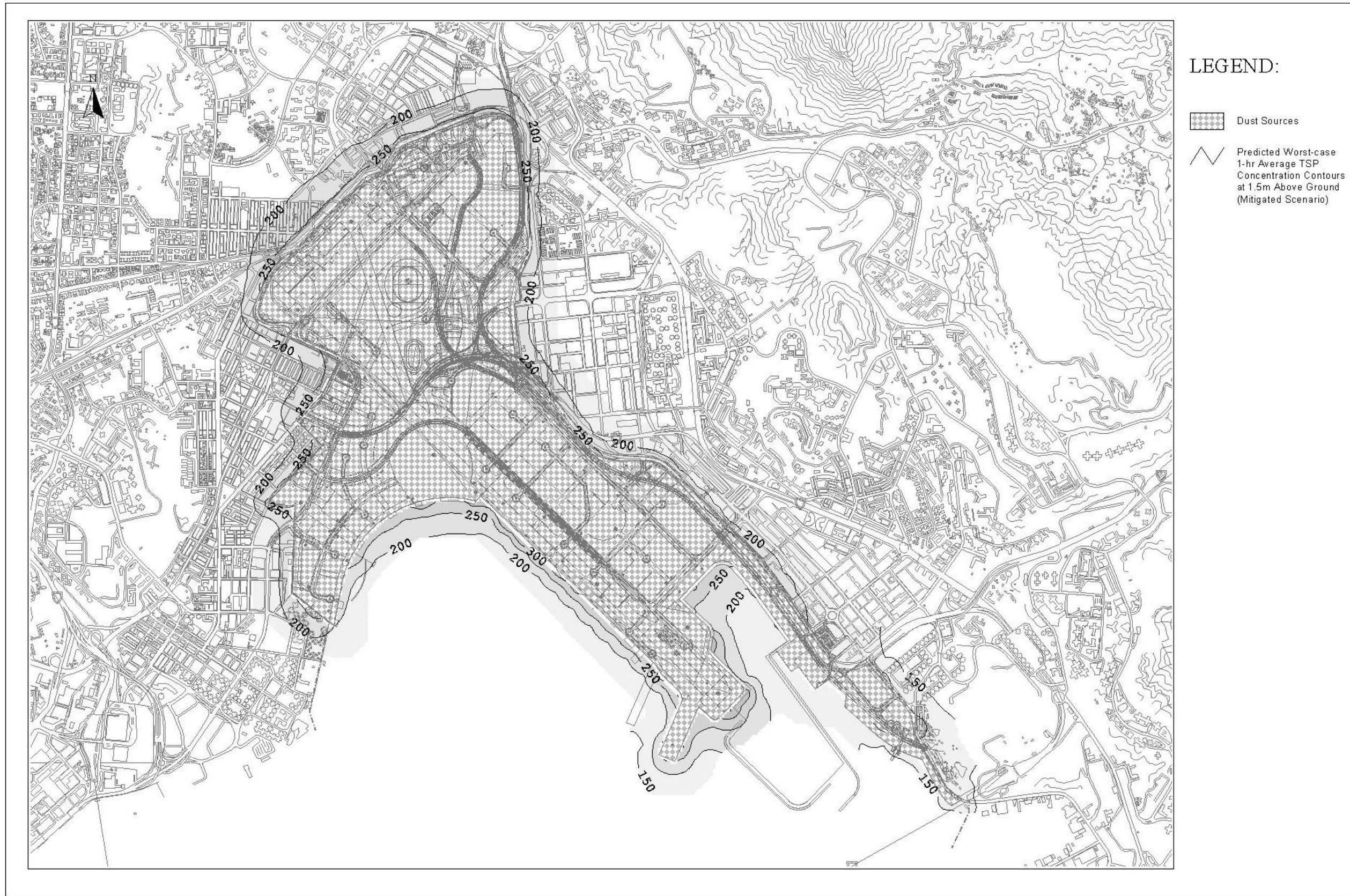
Drawing No. 22936/EN/391 Predicted Worst-case 1-hr Average TSP Concentration Contours at 1.5m Above Ground (Mitigated Scenario)
