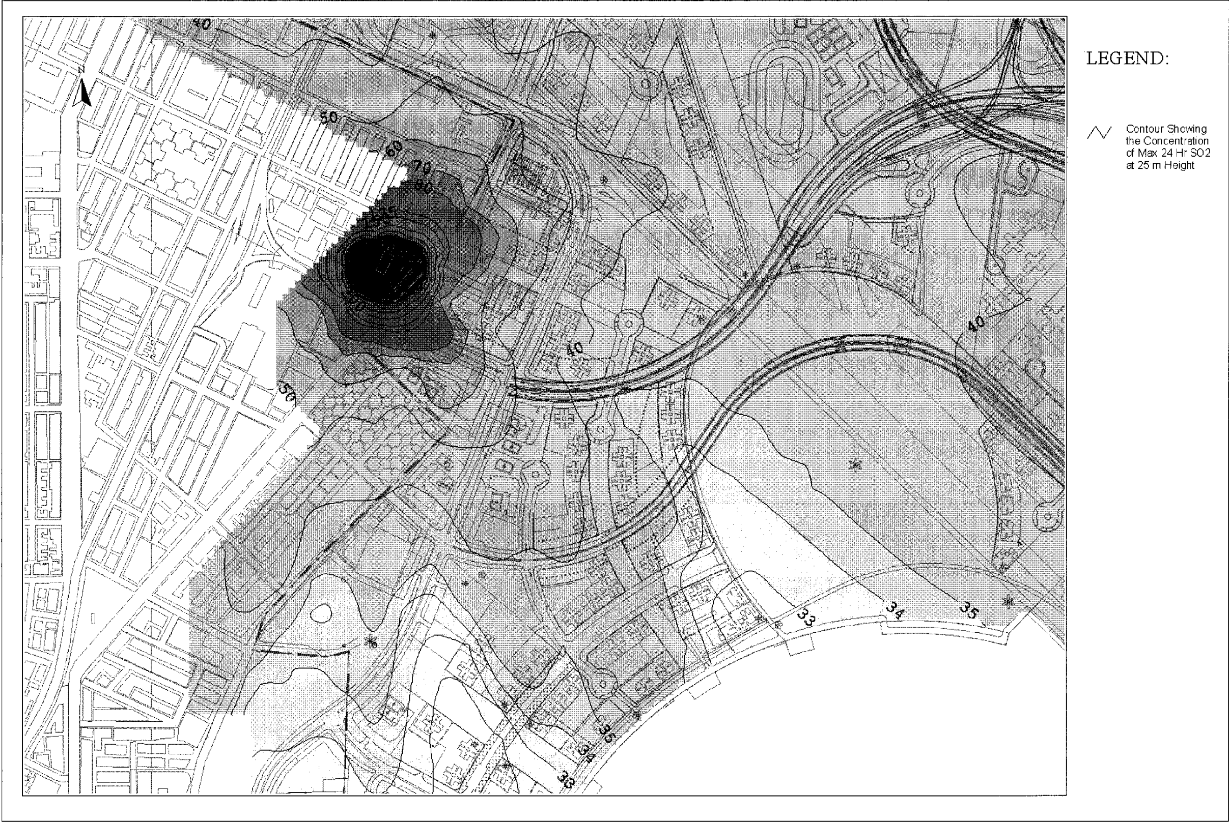
Drawing No. 22936/EN/333C Predicted Worst-case 24-hr Average SO 2 Concentration Contours at 25m Above Ground
