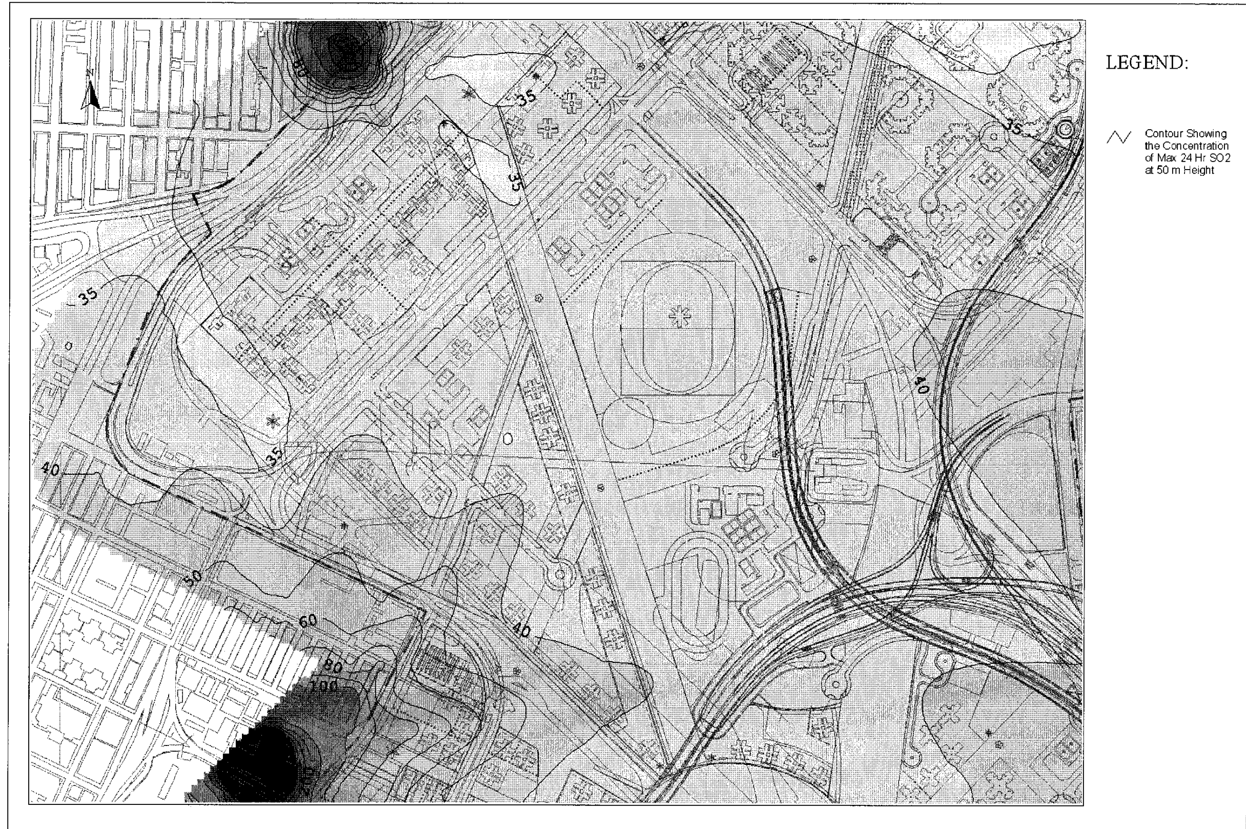
Drawing No. 22936/EN/334B Predicted Worst-case 24-hr Average SO 2 Concentration Contours at 50m Above Ground
