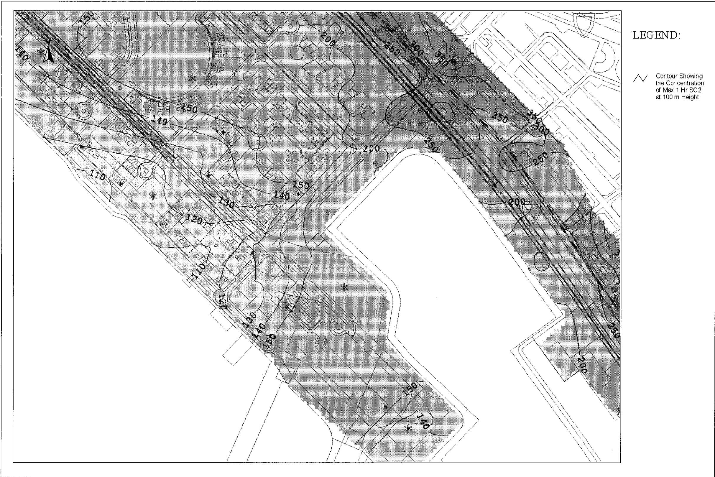
Drawing No. 22936/EN/332F Predicted Worst-case 1-hr Average SO 2 Concentration Contours at 100m Above Ground
