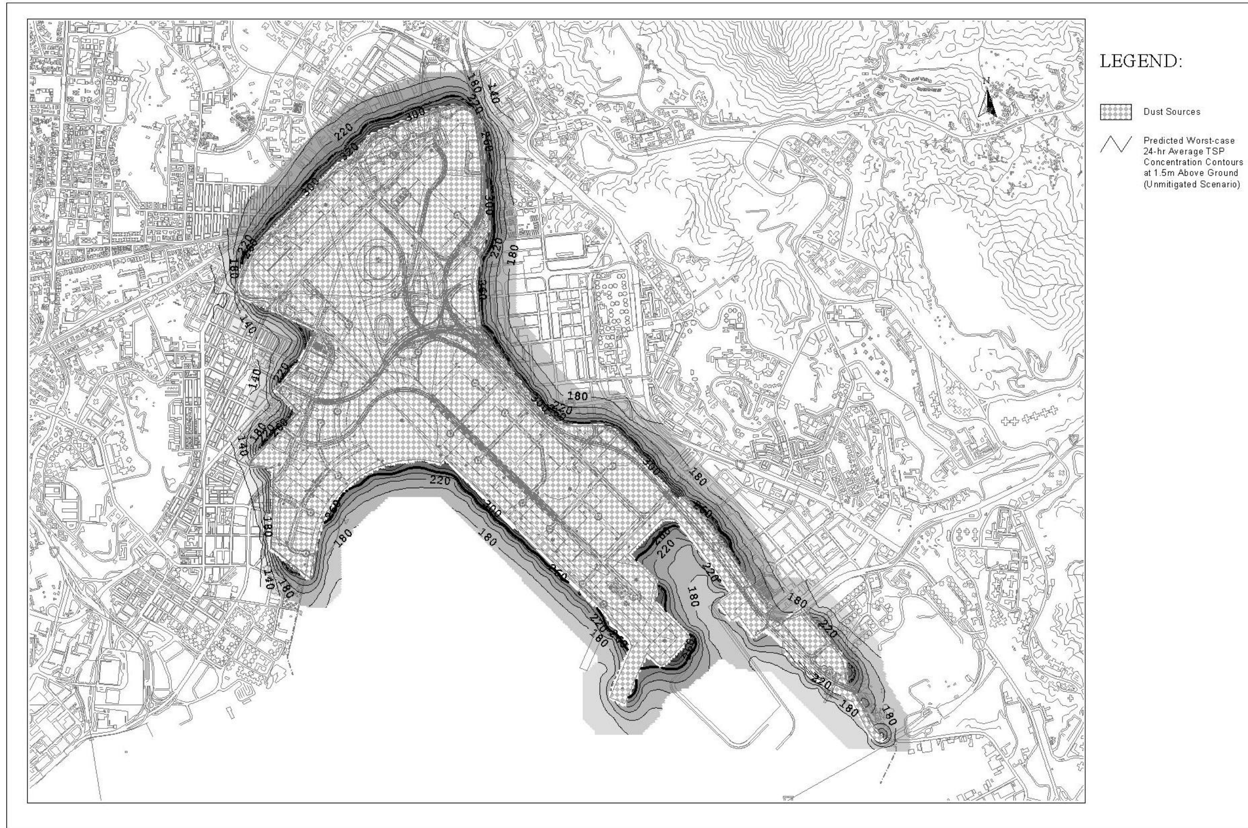
Drawing No. 22936/EN/390 Predicted Worst-case 24-hr Average TSP Concentration Contours at 1.5m Above Ground (Unmitigated Scenario)
