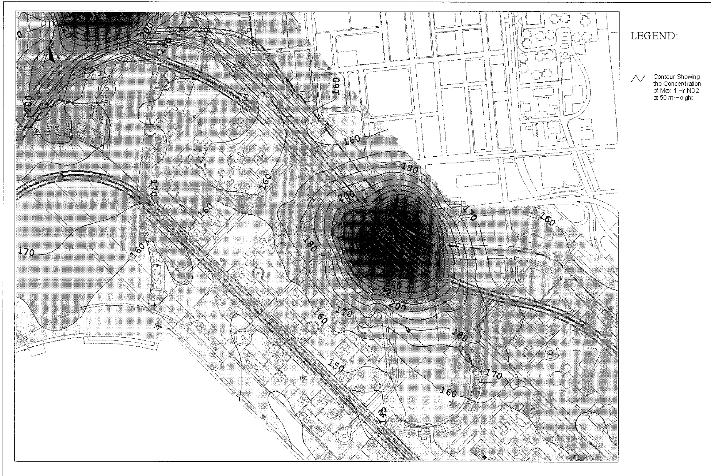
Drawing No. 22936/EN/319E Predicted Worst-case 1-hr Average NO 2 Concentration Contours at 50m Above Ground
