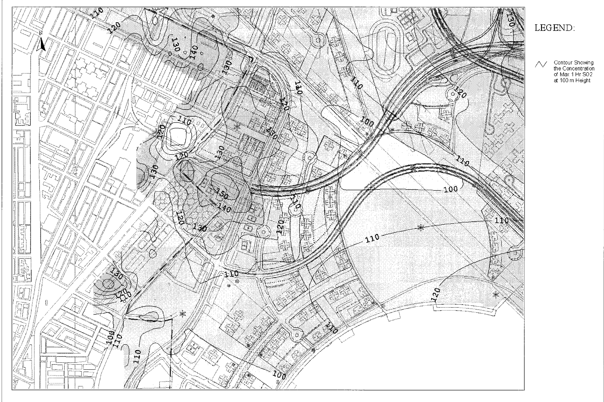
Drawing No. 22936/EN/332C Predicted Worst-case 1-hr Average SO 2 Concentration Contours at 100m Above Ground
