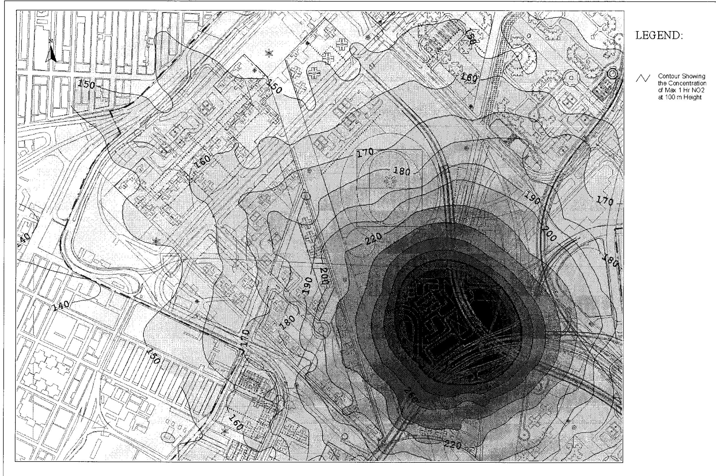
Drawing No. 22936/EN/321B Predicted Worst-case 1-hr Average NO 2 Concentration Contours at 100m Above Ground
