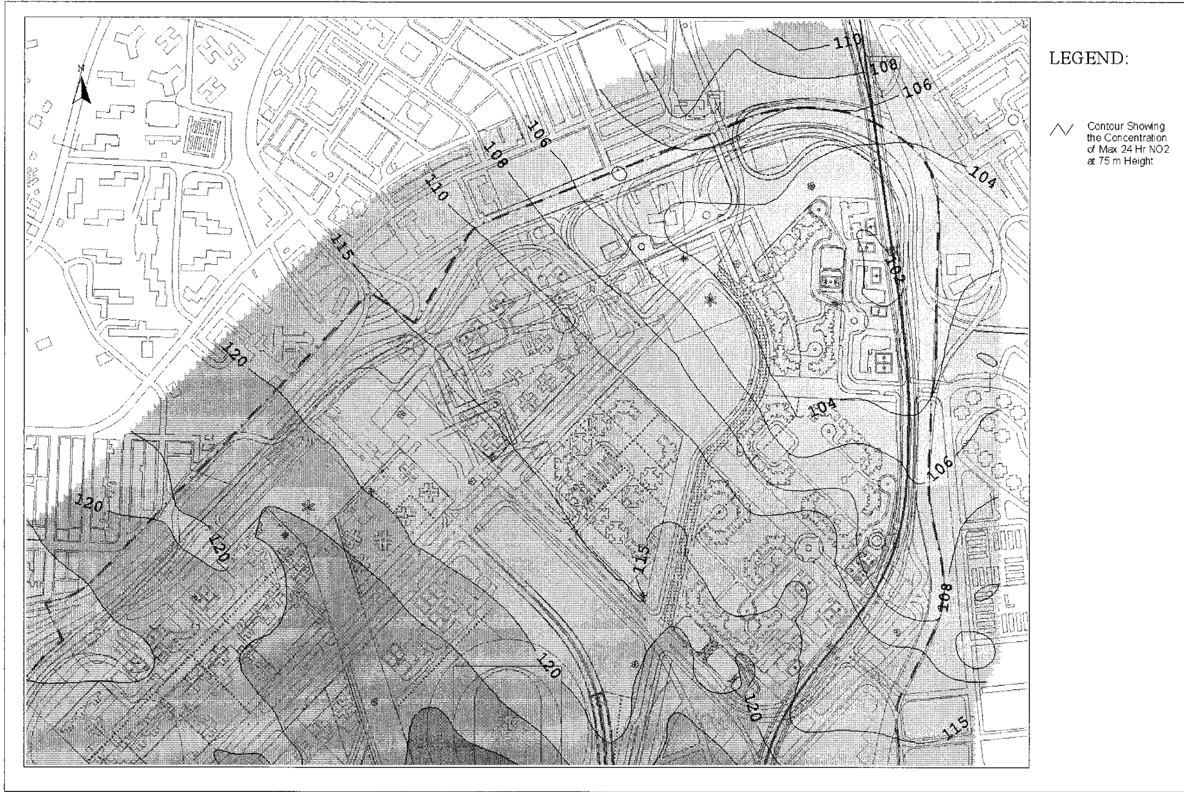
Drawing No. 22936/EN/326A Predicted Worst-case 24-hr Average NO 2 Concentration Contours at 75m Above Ground
