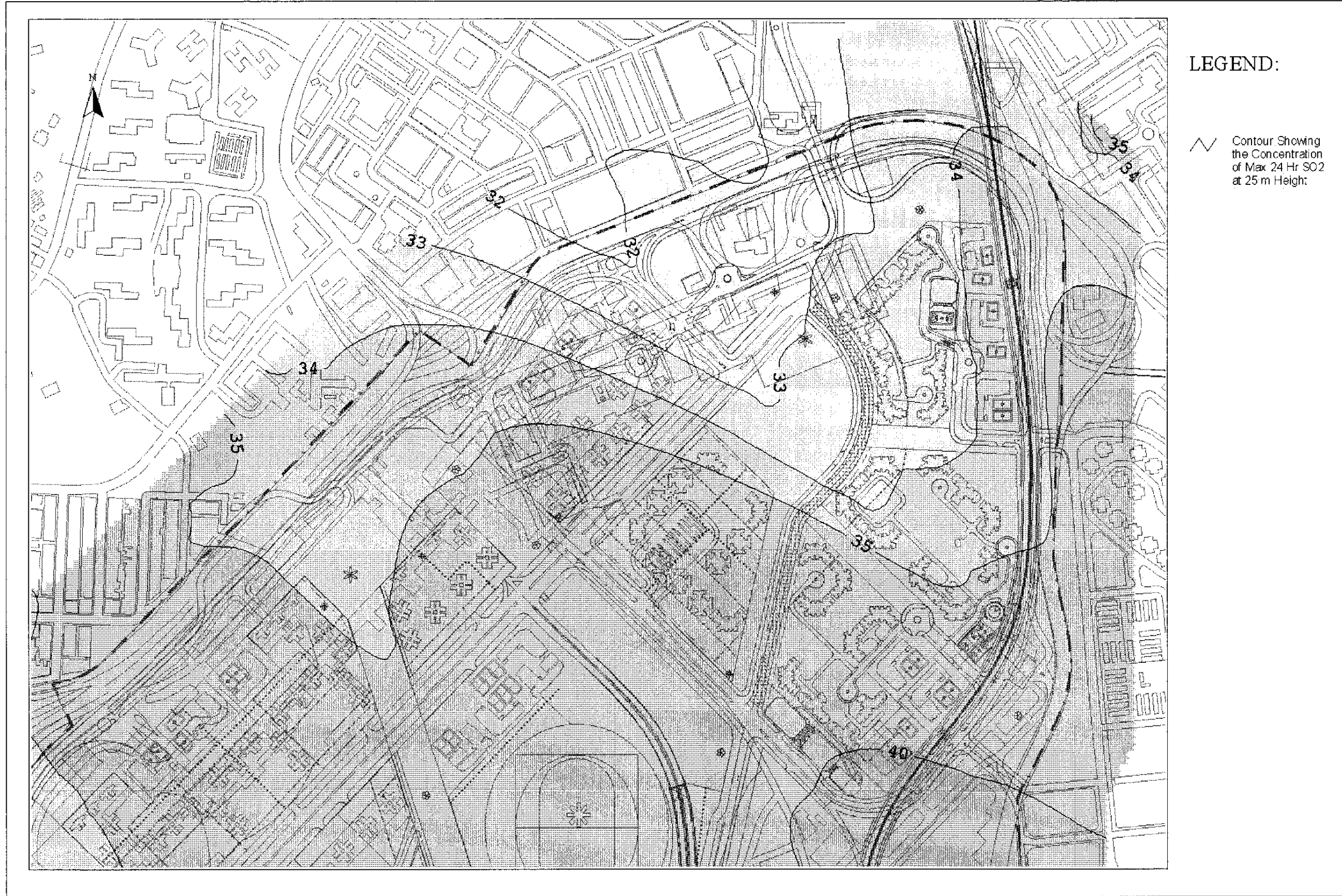
Drawing No. 22936/EN/333A Predicted Worst-case 24-hr Average SO 2 Concentration Contours at 25m Above Ground
