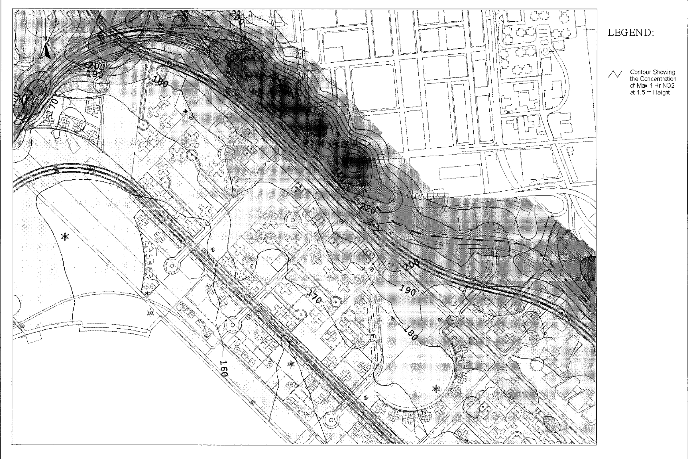
Drawing No. 22936/EN/316E Predicted Worst-case 1-hr Average NO 2 Concentration Contours at 1.5m Above Ground
