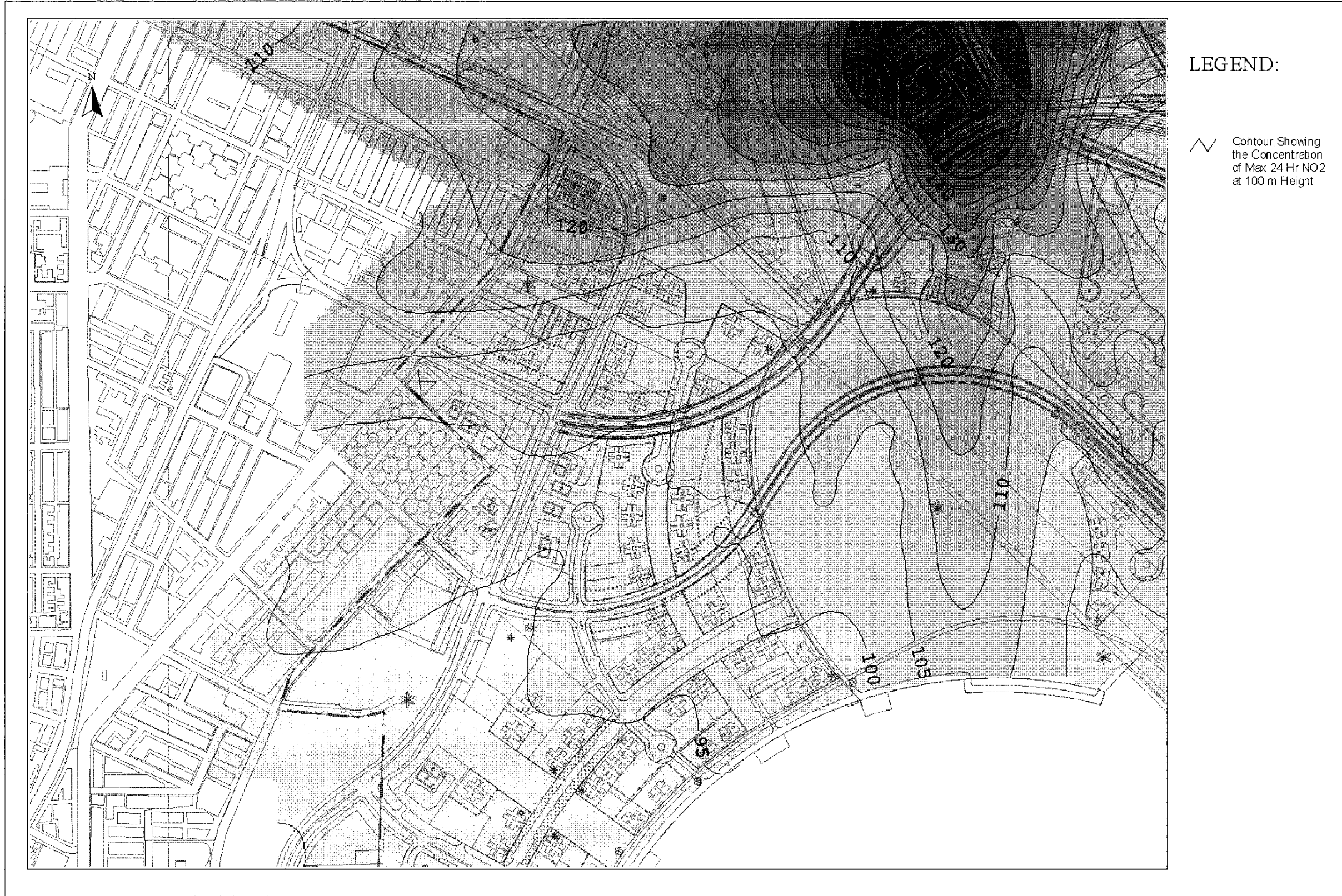
Drawing No. 22936/EN/327C Predicted Worst-case 24-hr Average NO 2 Concentration Contours at 100m Above Ground
