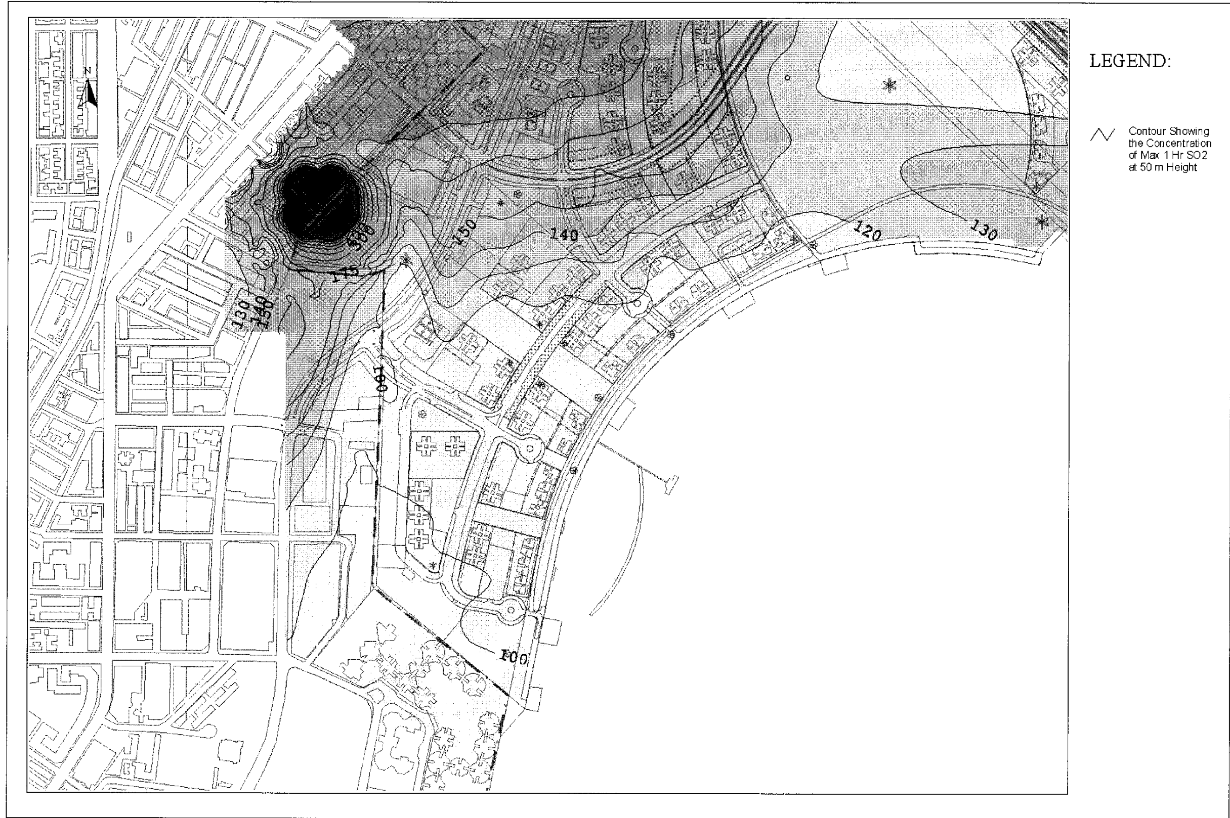
Drawing No. 22936/EN/330D Predicted Worst-case 1-hr Average SO 2 Concentration Contours at 50m Above Ground
