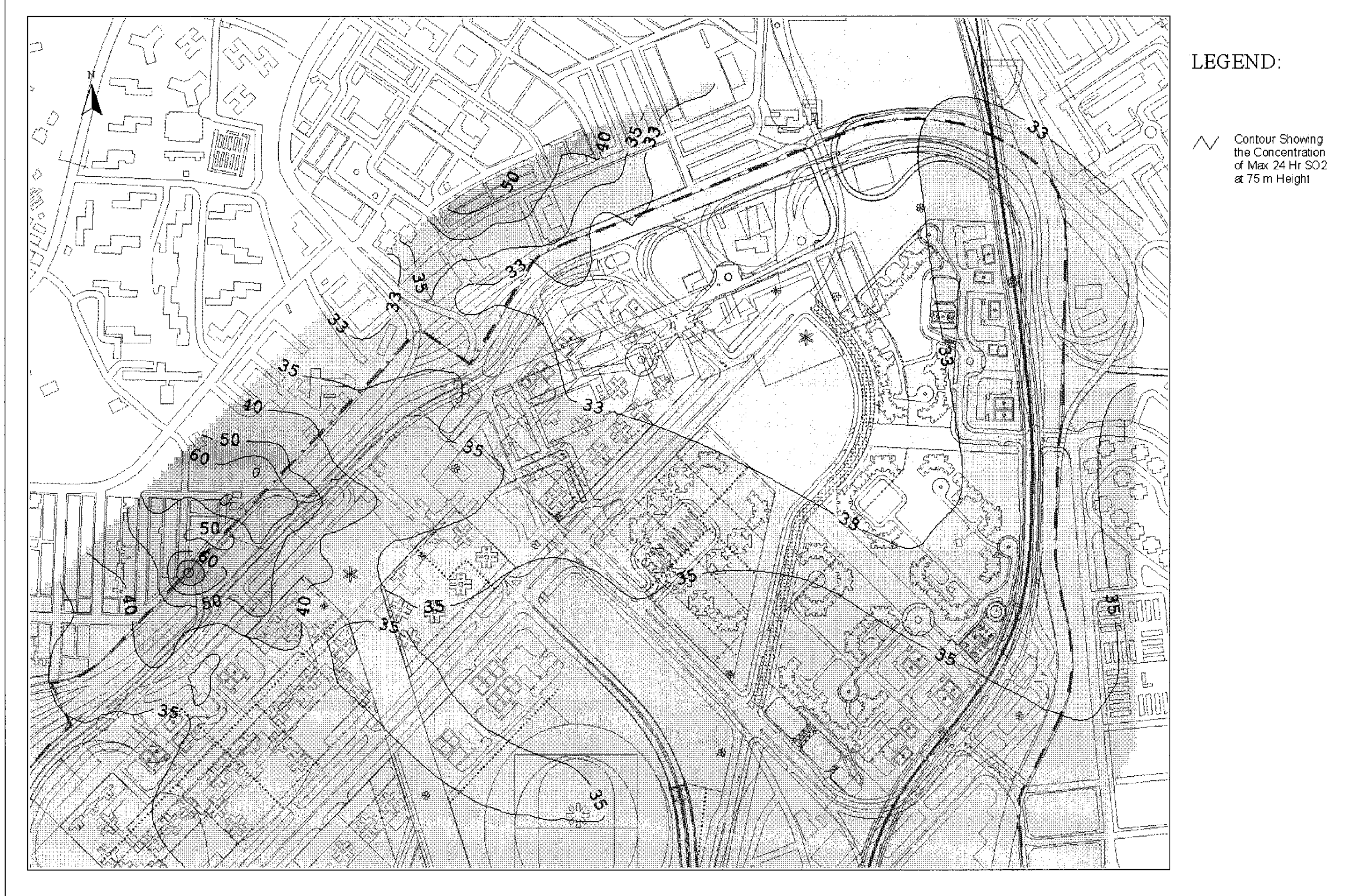
Drawing No. 22936/EN/335A Predicted Worst-case 24-hr Average SO2 Concentration Contours at 75m Above Ground
