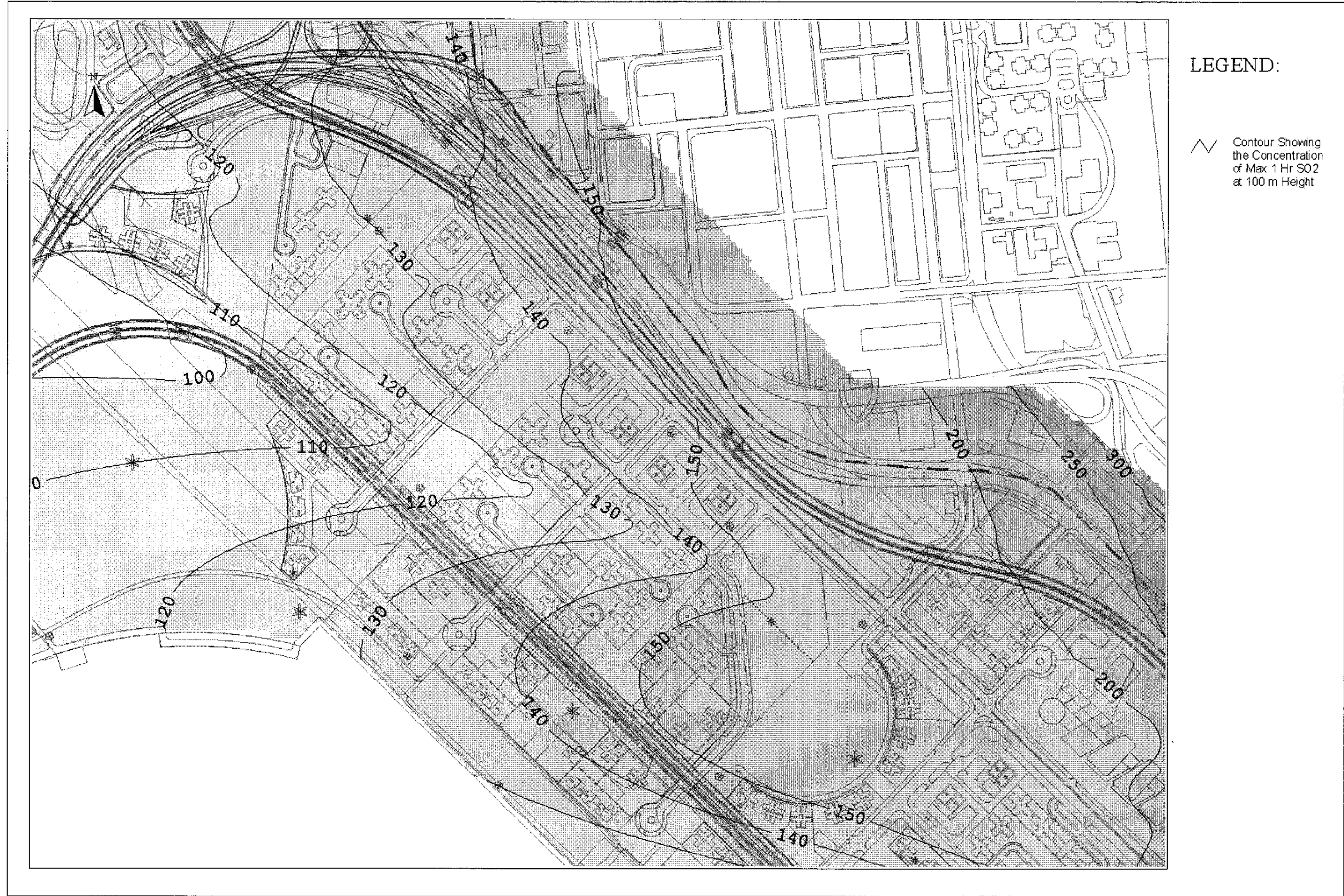
Drawing No. 22936/EN/332E Predicted Worst-case 1-hr Average SO 2 Concentration Contours at 100m Above Ground
