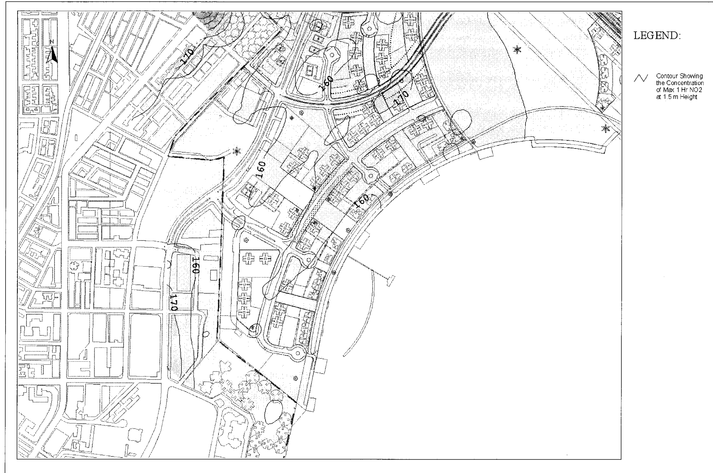
Drawing No. 22936/EN/316D Predicted Worst-case 1-hr Average NO 2 Concentration Contours at 1.5m Above Ground
