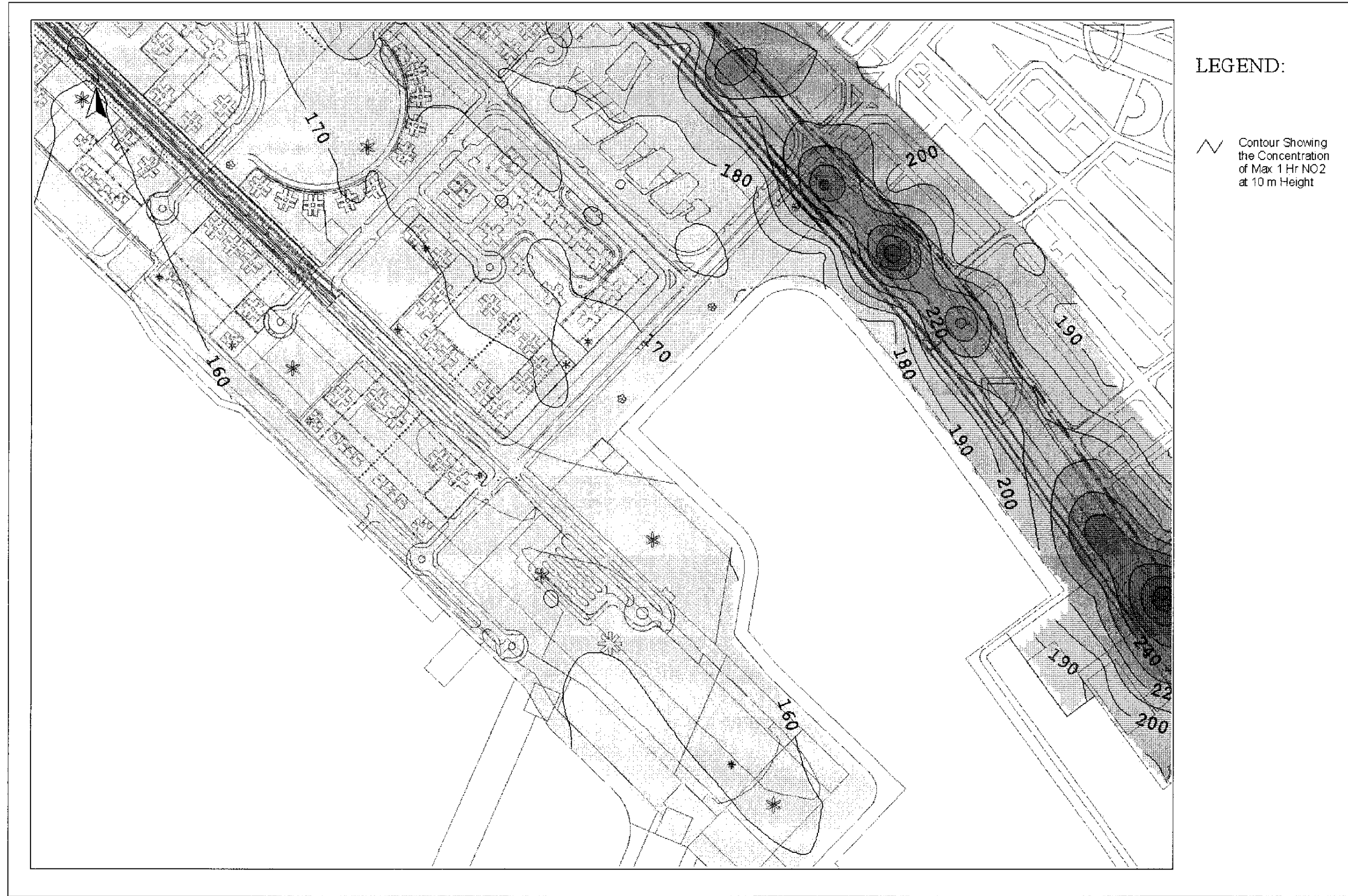
Drawing No. 22936/EN/317F Predicted Worst-case 1-hr Average NO 2 Concentration Contours at 10m Above Ground
