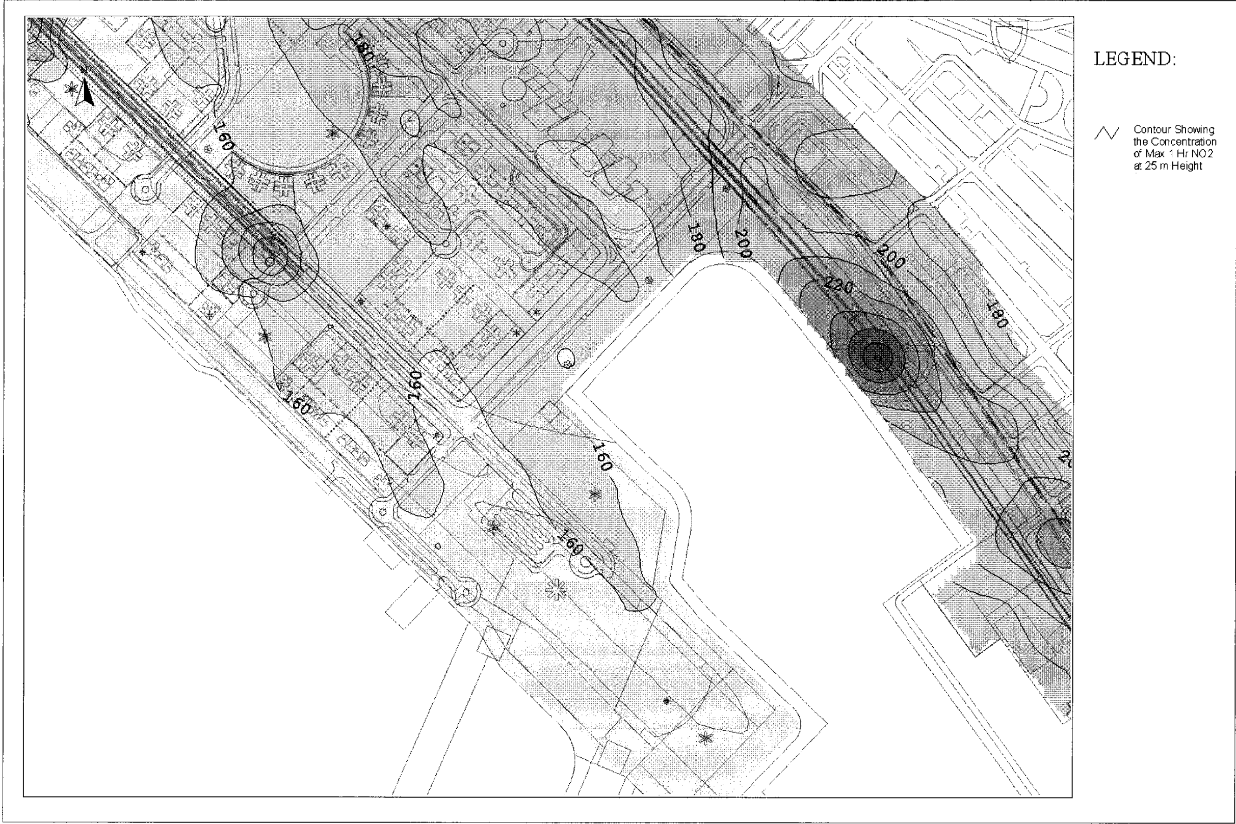
Drawing No. 22936/EN/318F Predicted Worst-case 1-hr Average NO 2 Concentration Contours at 25m Above Ground
