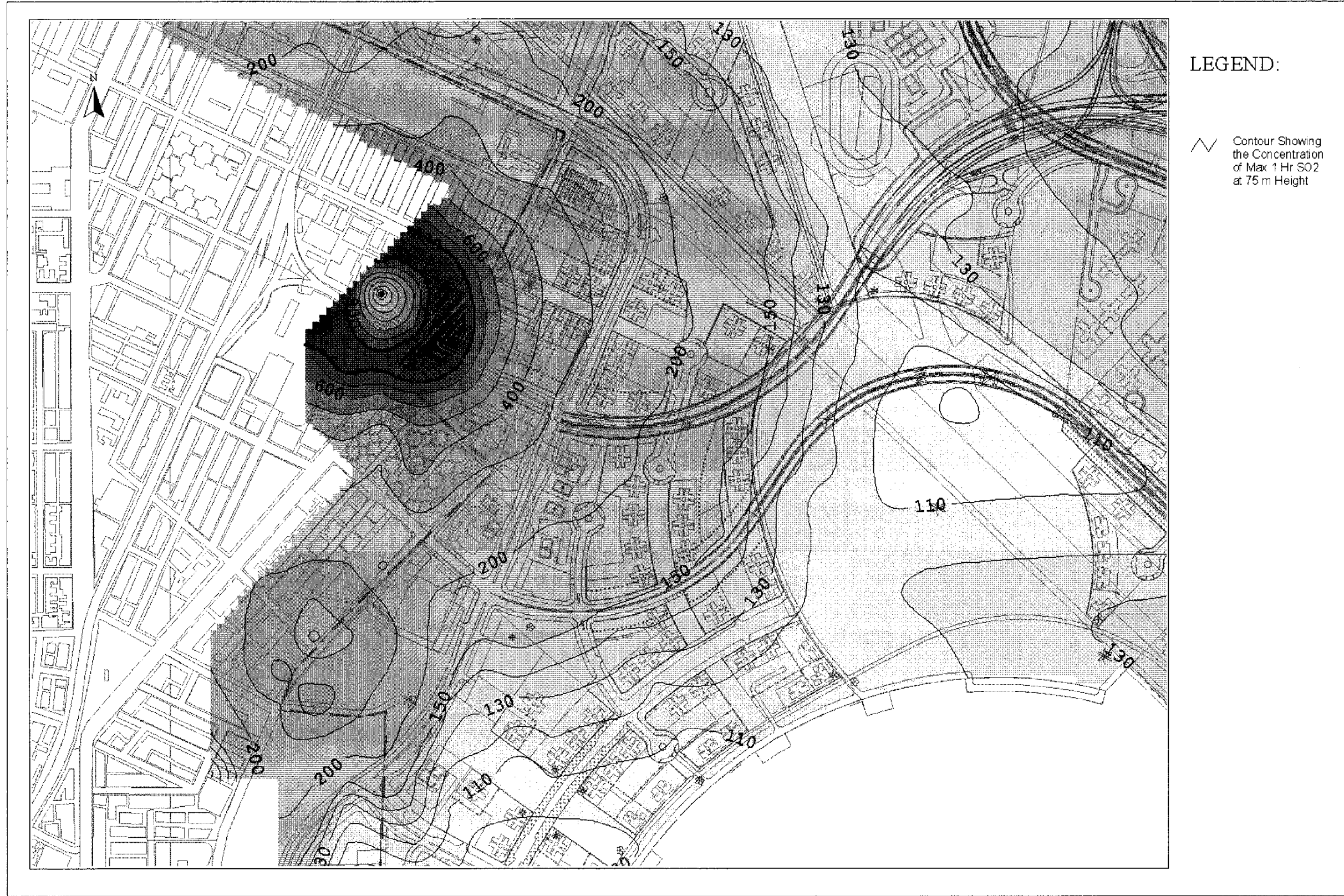
Drawing No. 22936/EN/331C Predicted Worst-case 1-hr Average SO 2 Concentration Contours at 75m Above Ground
