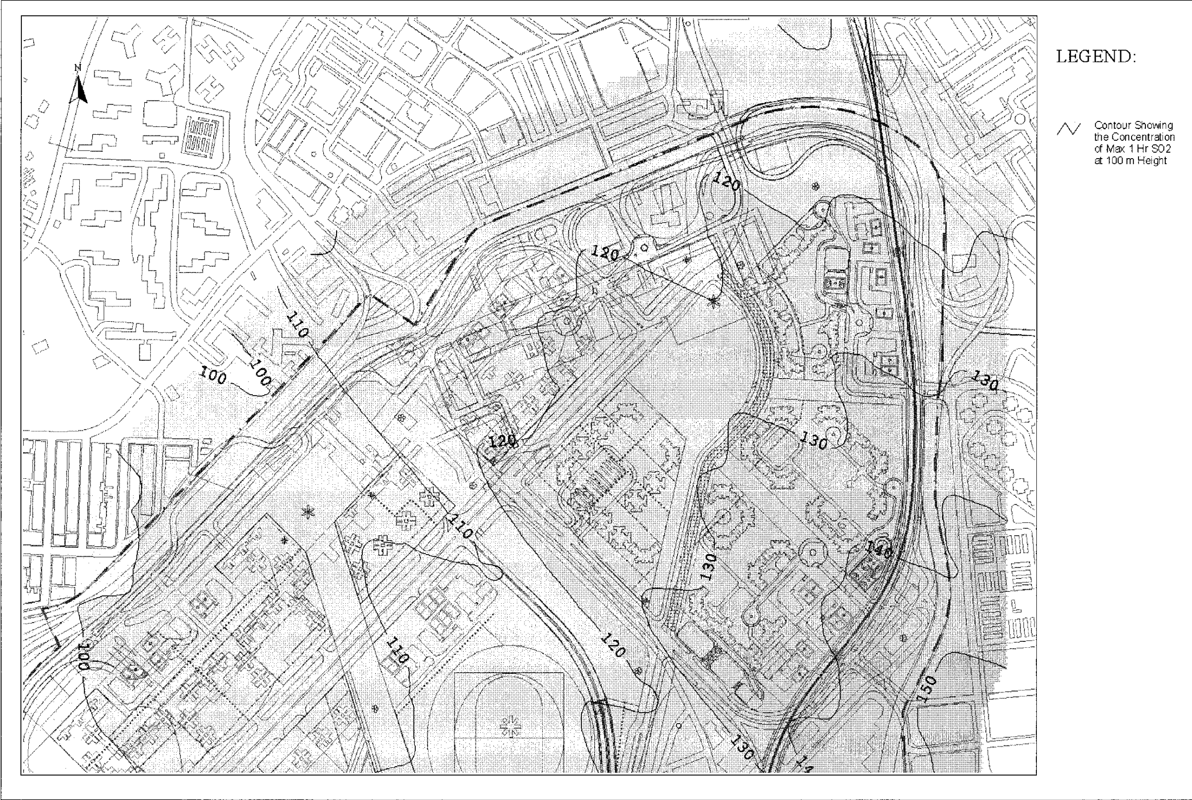
Drawing No. 22936/EN/332A Predicted Worst-case 1-hr Average SO 2 Concentration Contours at 100m Above Ground
