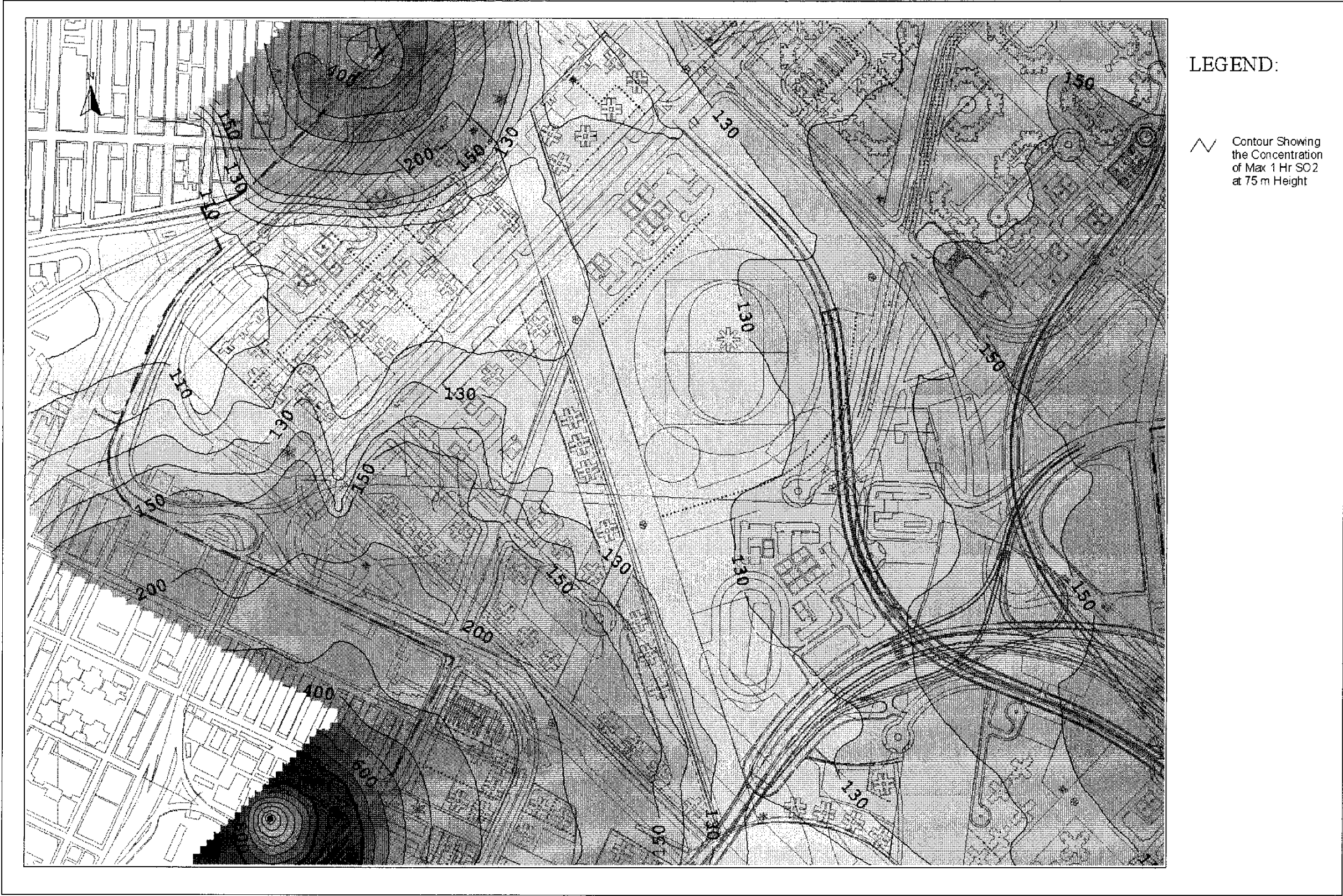
Drawing No. 22936/EN/331B Predicted Worst-case 1-hr Average SO 2 Concentration Contours at 75m Above Ground
