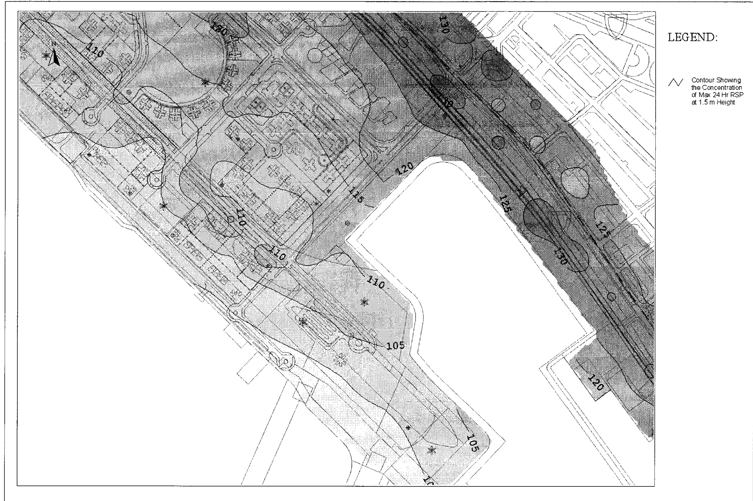
Drawing No. 22936/EN/328F Predicted Worst-case 24-hr Average RSP Concentration Contours at 1.5m Above Ground
