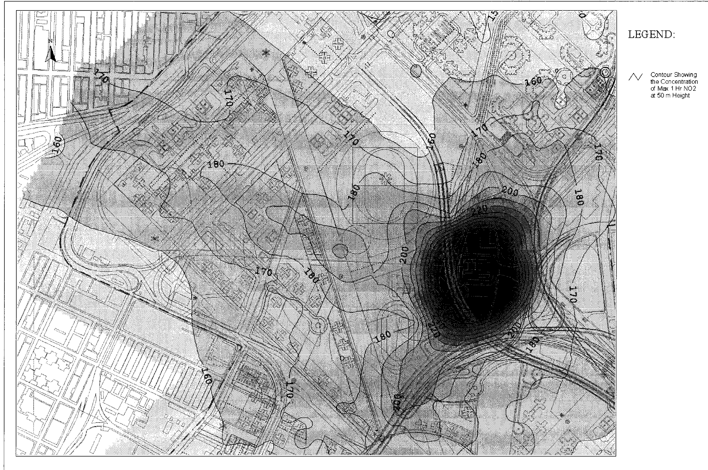
Drawing No. 22936/EN/319B Predicted Worst-case 1-hr Average NO 2 Concentration Contours at 50m Above Ground
