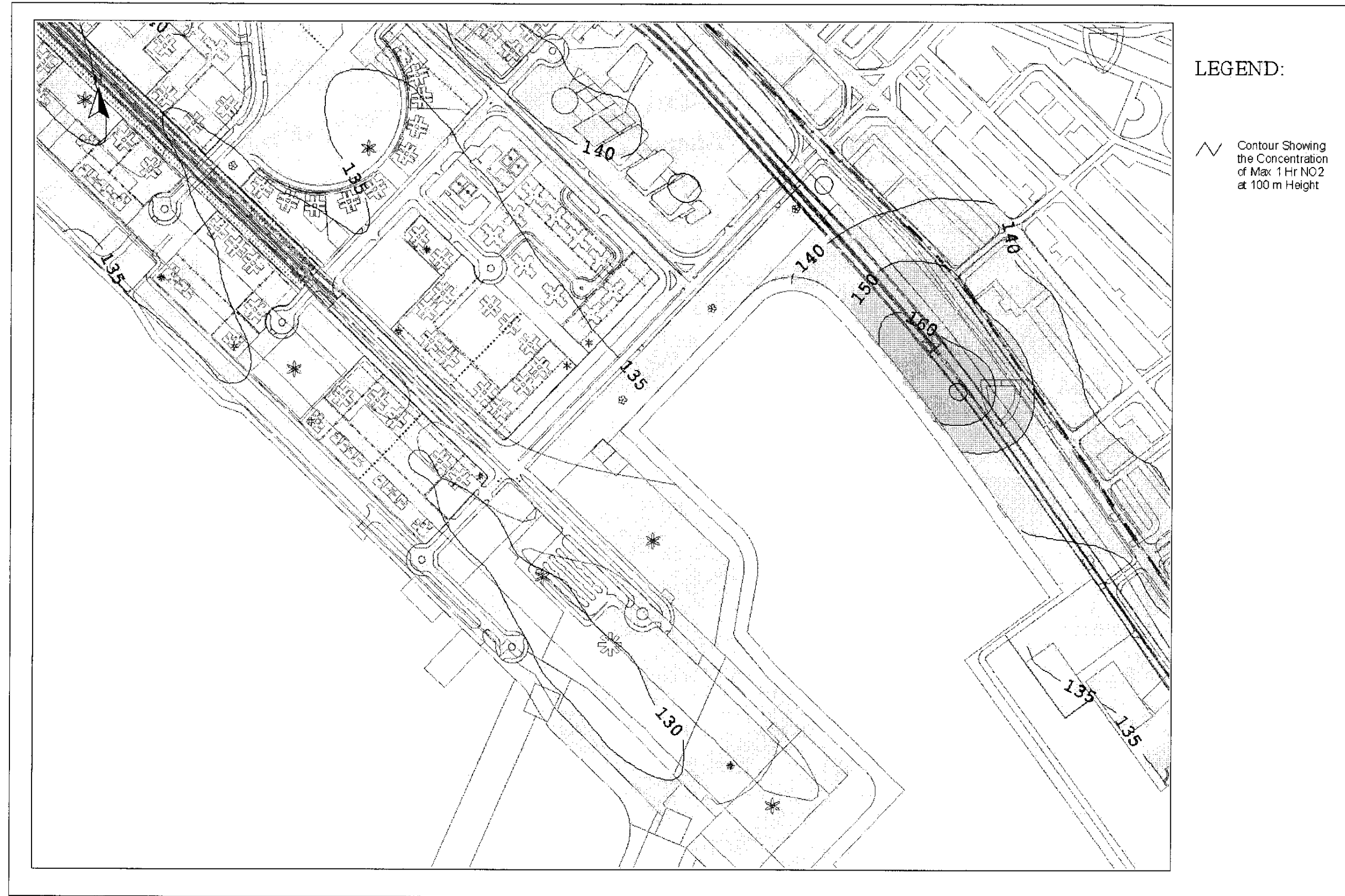
Drawing No. 22936/EN/321F Predicted Worst-case 1-hr Average NO 2 Concentration Contours at 100m Above Ground
