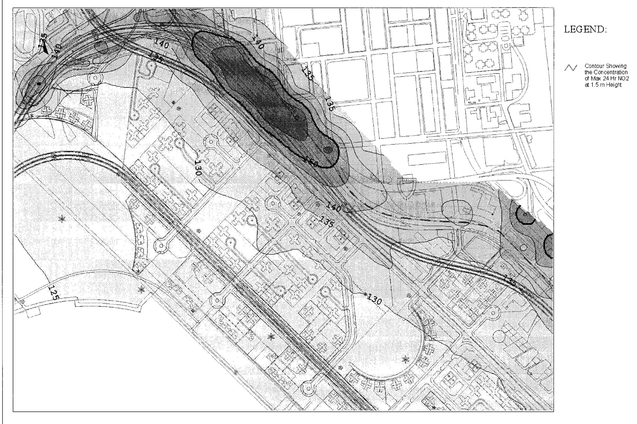
Drawing No. 22936/EN/322E Predicted Worst-case 24-hr Average NO 2 Concentration Contours at 1.5m Above Ground
