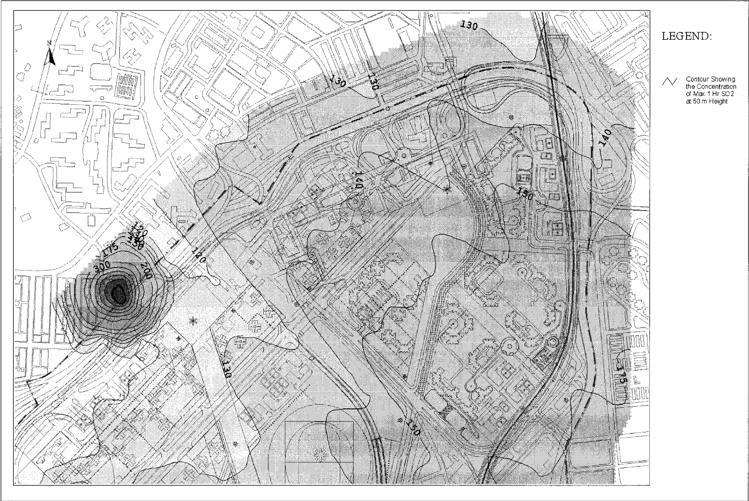
Drawing No. 22936/EN/330A Predicted Worst-case 1-hr Average SO 2 Concentration Contours at 50m Above Ground
