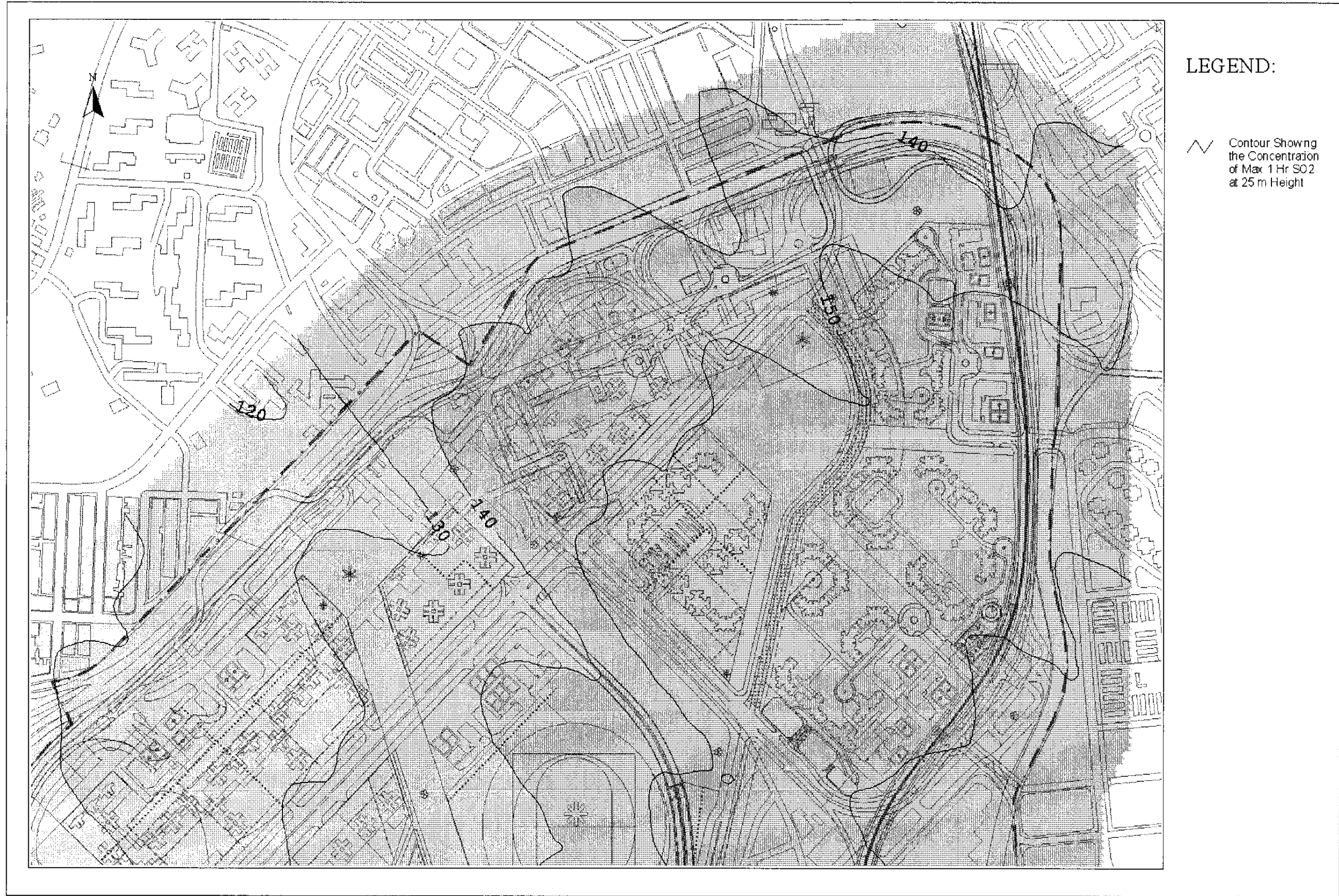
Drawing No. 22936/EN/329A Predicted Worst-case 1-hr Average SO 2 Concentration Contours at 25m Above Ground
