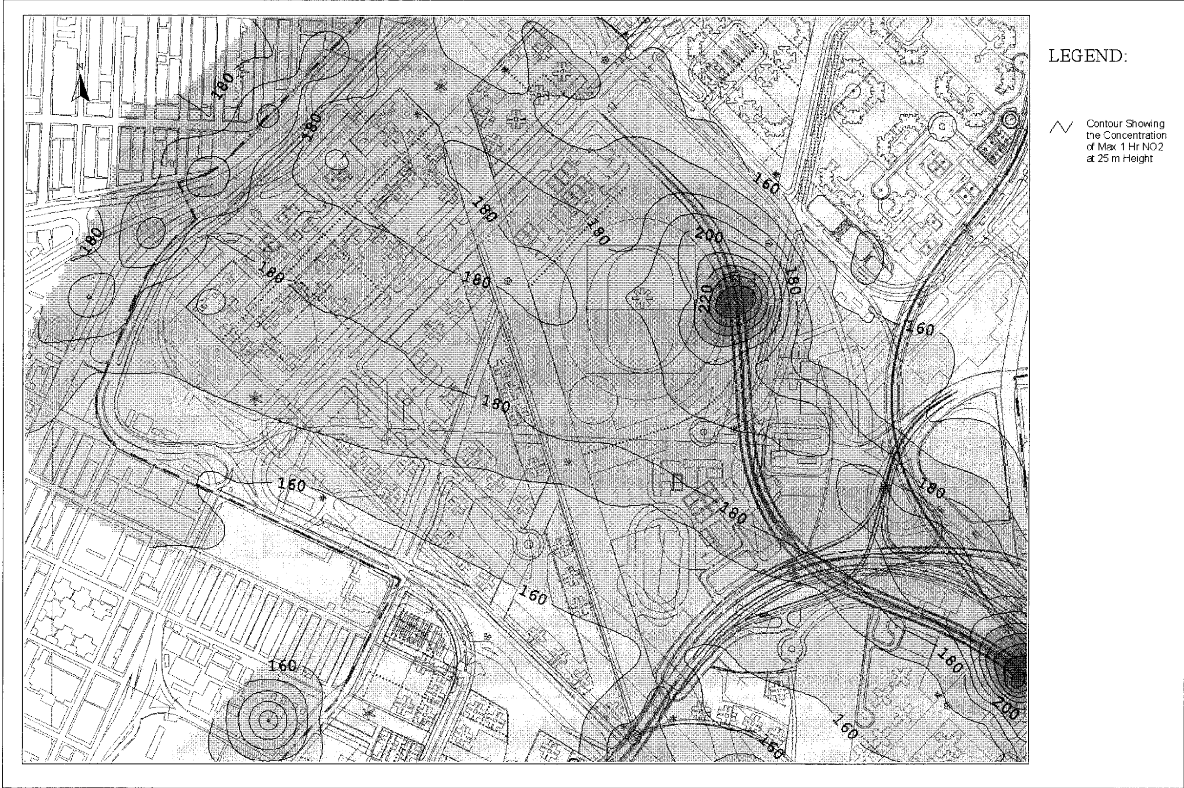
Drawing No. 22936/EN/318B Predicted Worst-case 1-hr Average NO 2 Concentration Contours at 25m Above Ground
