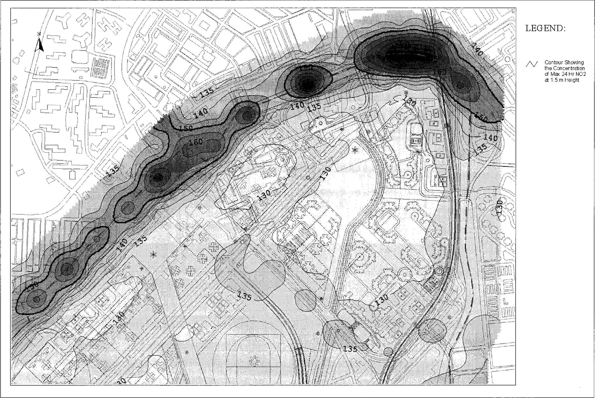
Drawing No. 22936/EN/322A Predicted Worst-case 24-hr Average NO 2 Concentration Contours at 1.5m Above Ground
