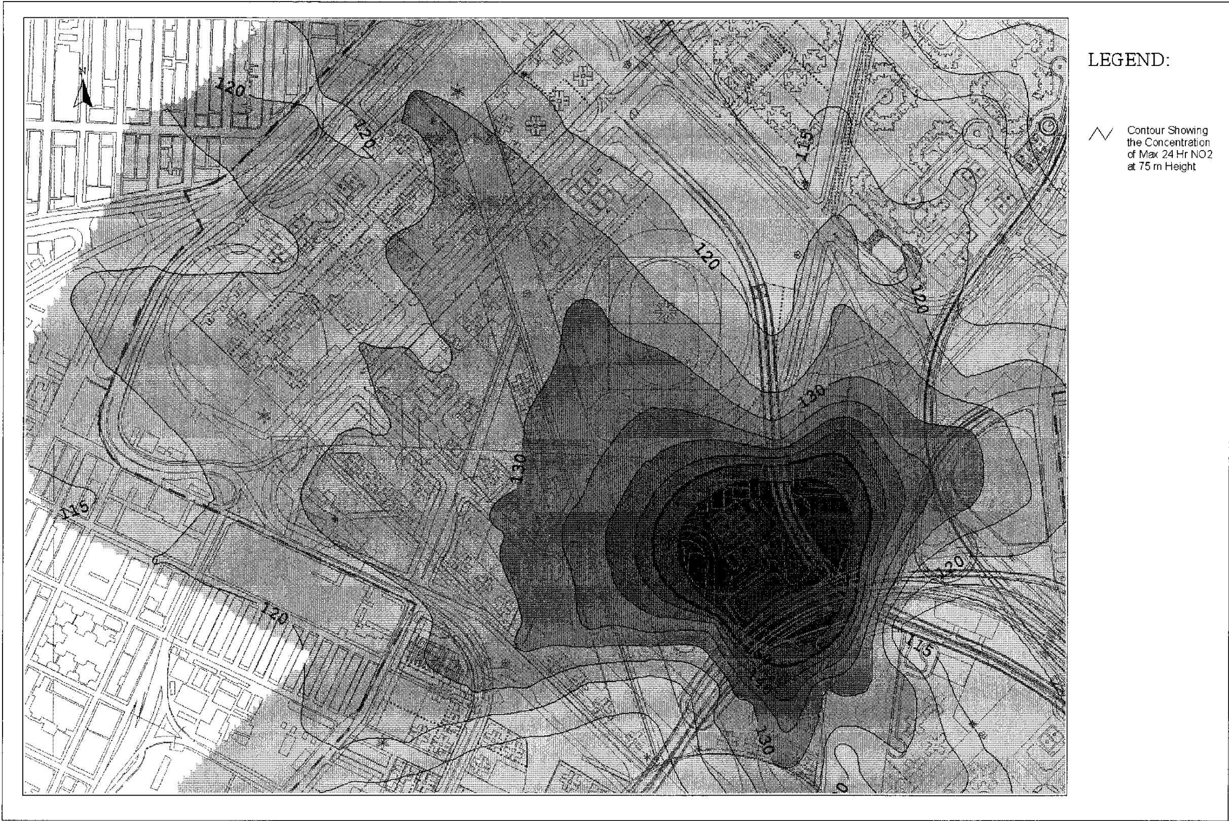
Drawing No. 22936/EN/326B Predicted Worst-case 24-hr Average NO 2 Concentration Contours at 75m Above Ground
