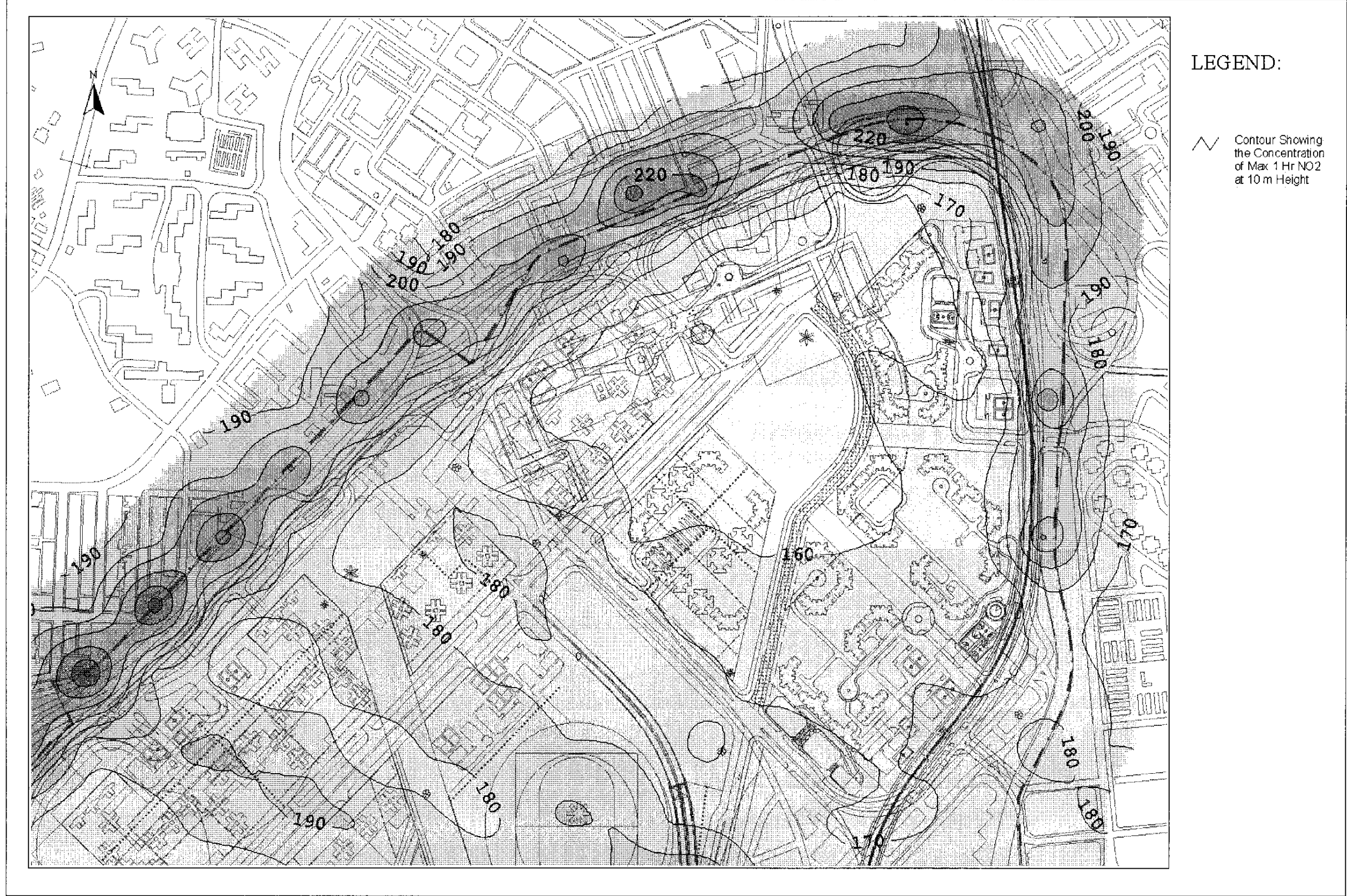
Drawing No. 22936/EN/317A Predicted Worst-case 1-hr Average NO 2 Concentration Contours at 10m Above Ground
