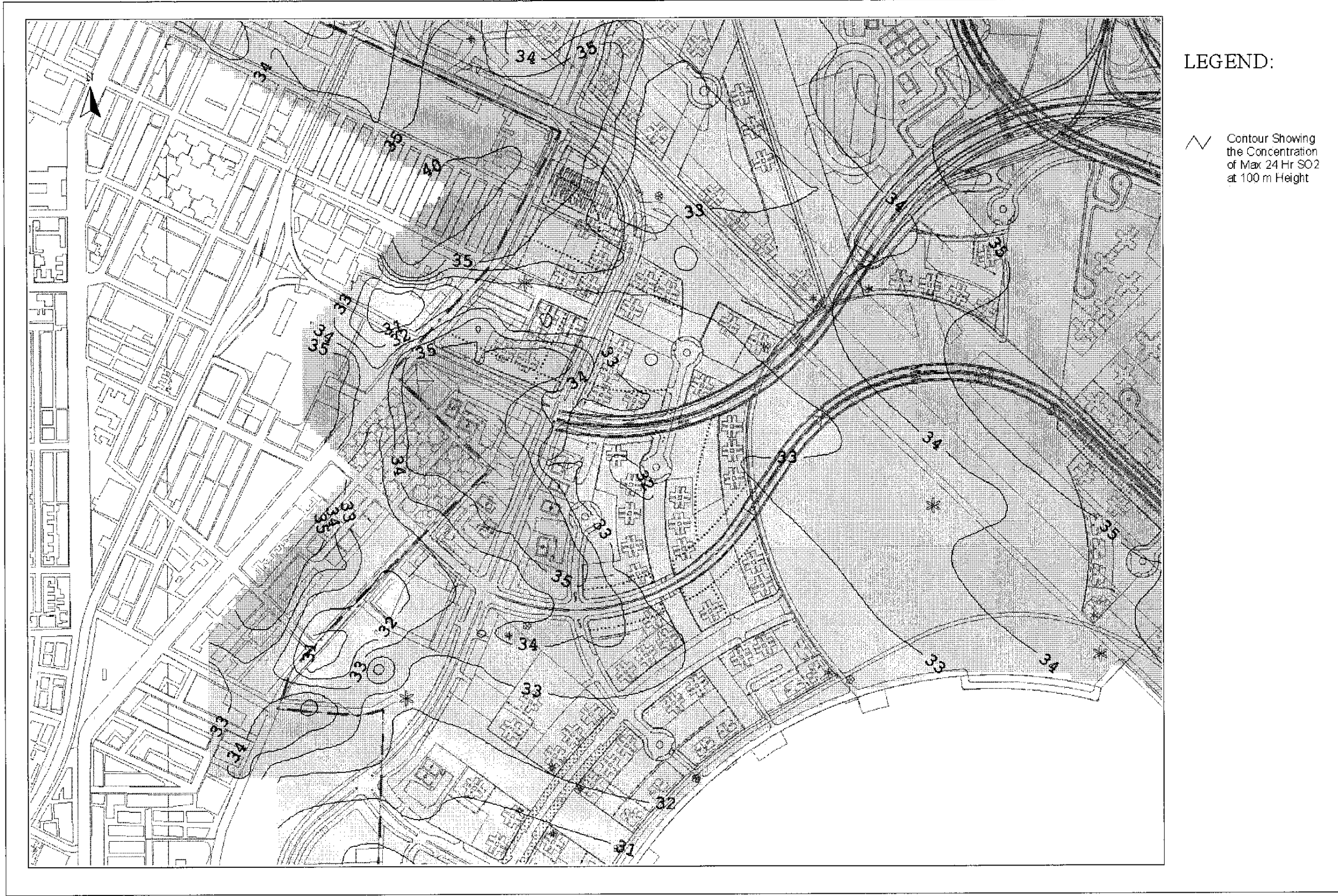
Drawing No. 22936/EN/336C Predicted Worst-case 24-hr Average SO 2 Concentration Contours at 100m Above Ground
