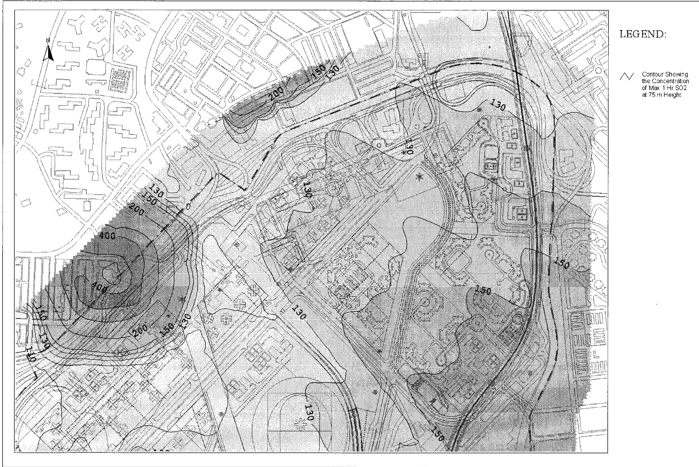
Drawing No. 22936/EN/331A Predicted Worst-case 1-hr Average SO 2 Concentration Contours at 75m Above Ground
