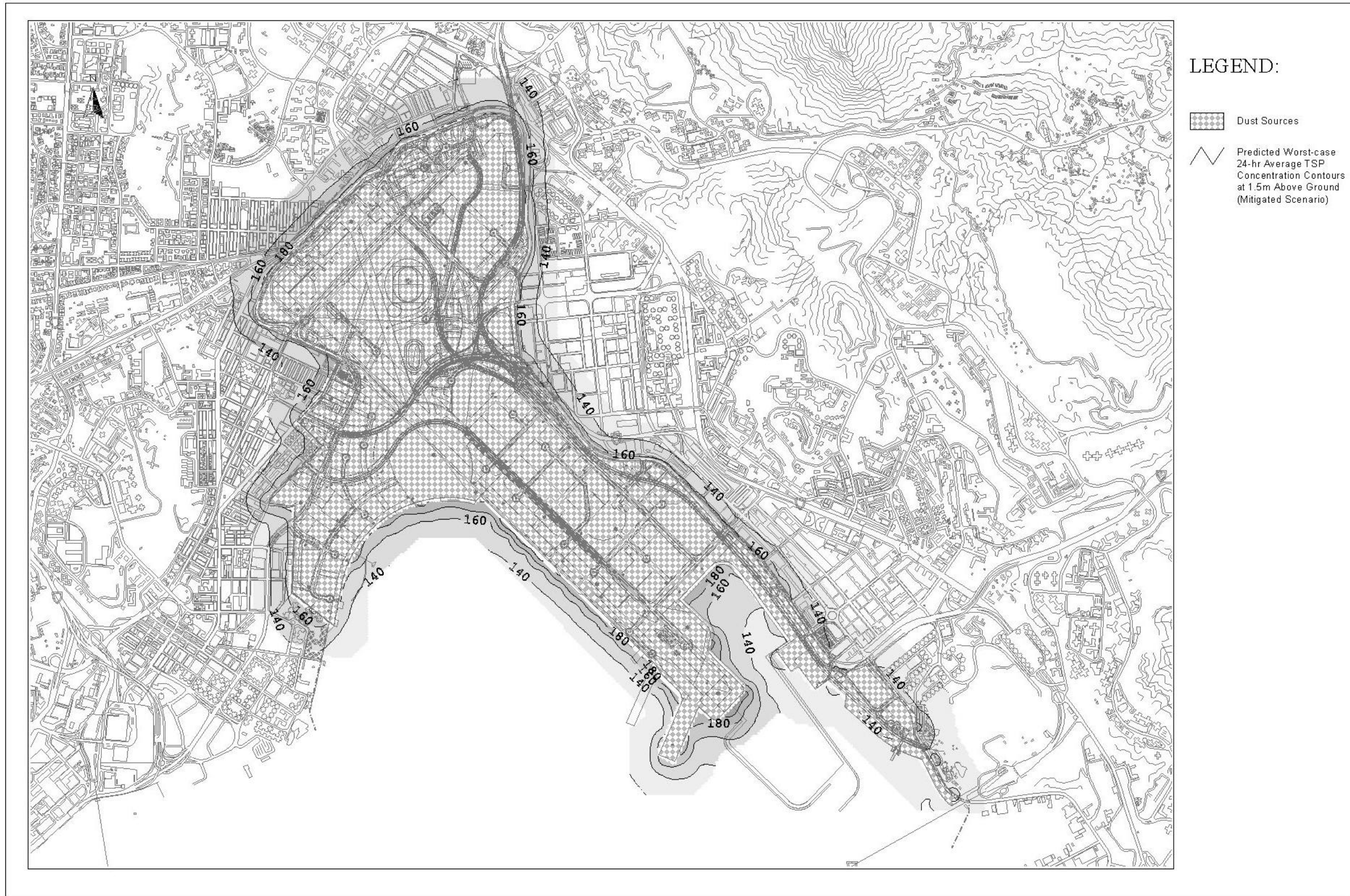
Drawing No. 22936/EN/392 Predicted Worst-case 24-hr Average TSP Concentration Contours at 1.5m Above Ground (Mitigated Scenario)
