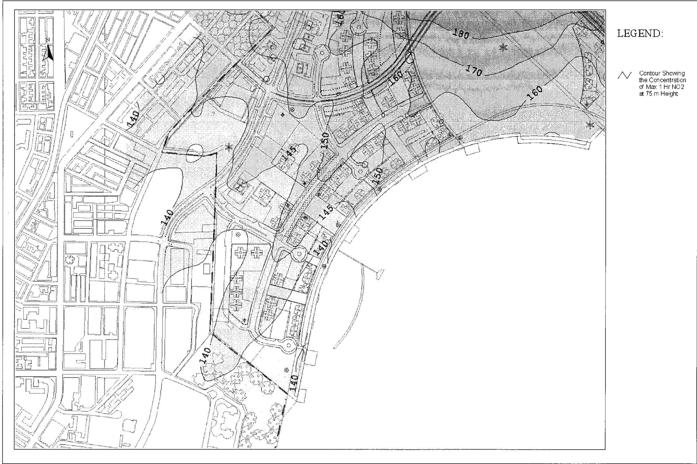
Drawing No. 22936/EN/320D Predicted Worst-case 1-hr Average NO 2 Concentration Contours at 75m Above Ground
