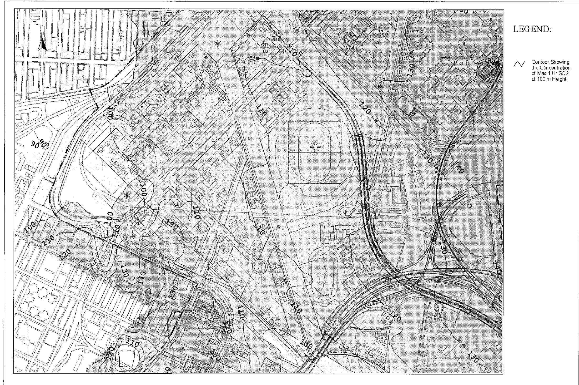
Drawing No. 22936/EN/332B Predicted Worst-case 1-hr Average SO 2 Concentration Contours at 100m Above Ground
