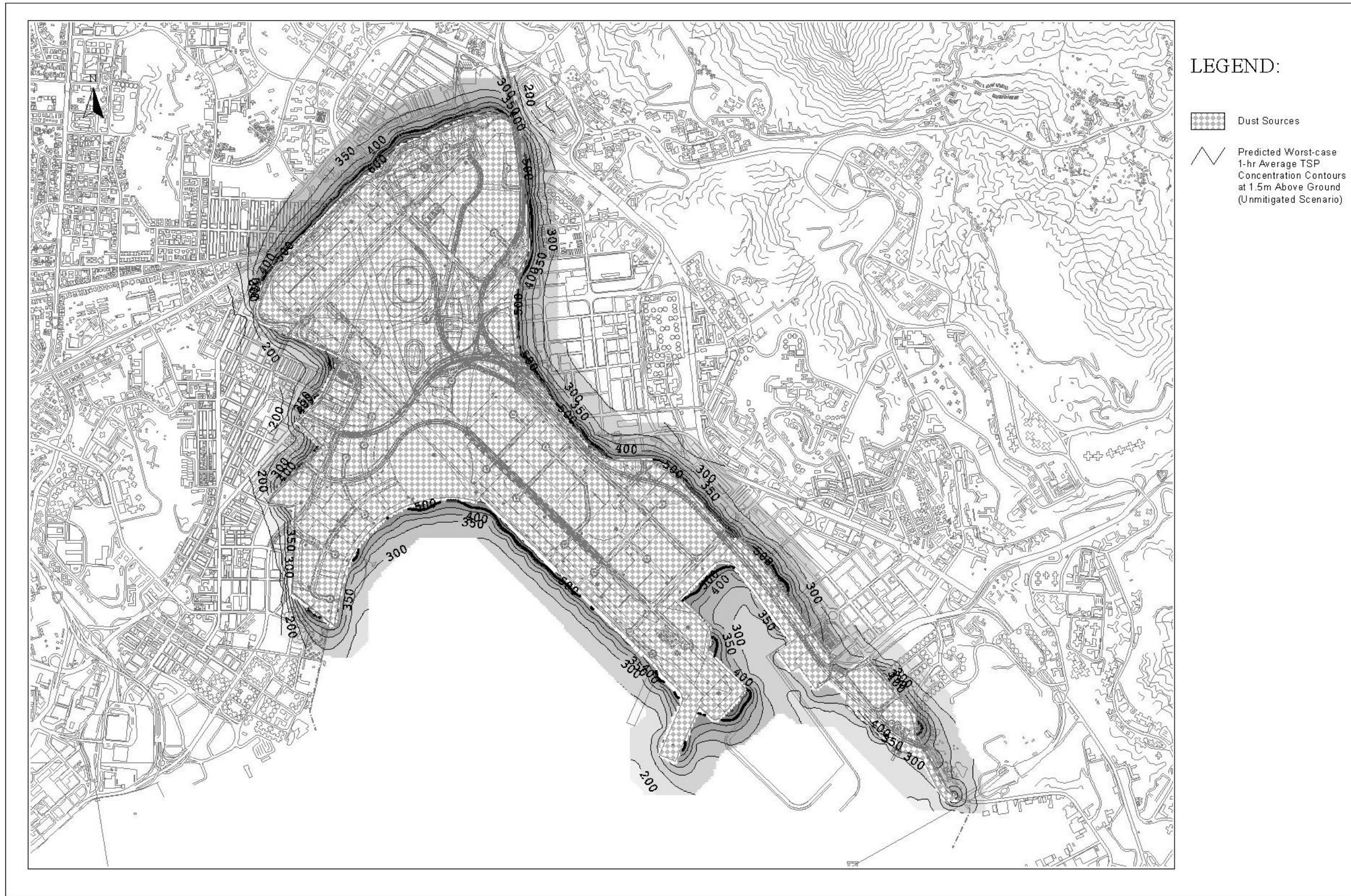
Drawing No. 22936/EN/389 Predicted Worst-case 1-hr Average TSP Concentration Contours at 1.5m Above Ground (Unmitigated Scenario)
