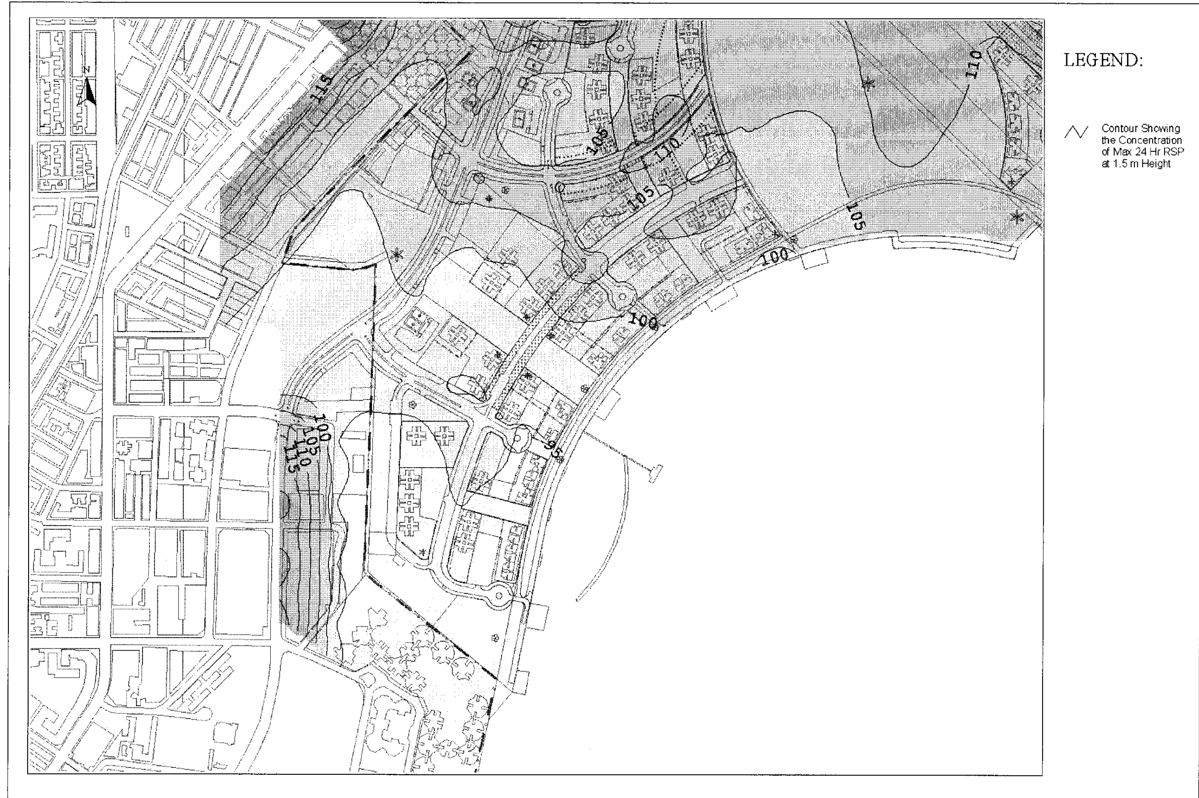
Drawing No. 22936/EN/328D Predicted Worst-case 24-hr Average RSP Concentration Contours at 1.5m Above Ground
