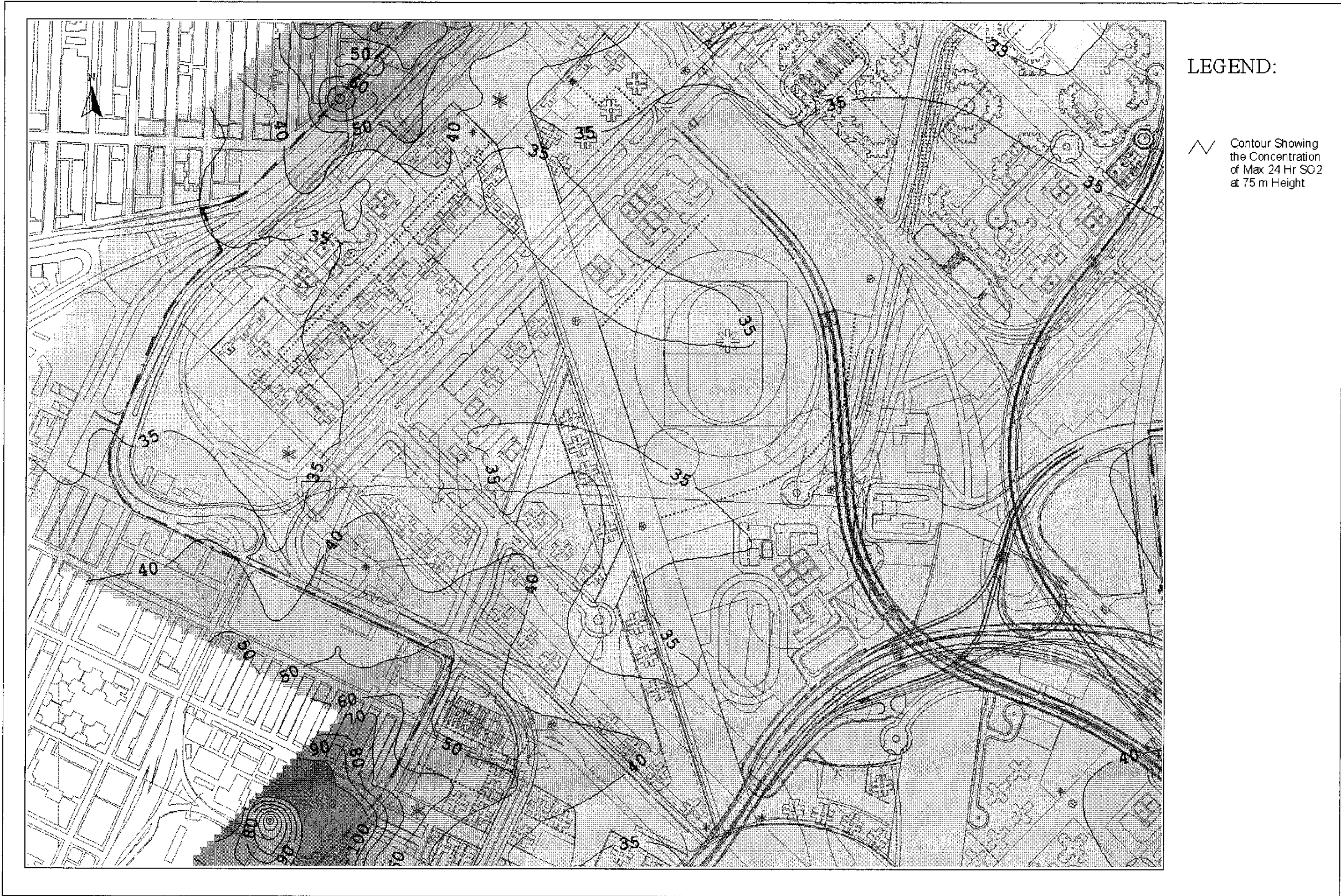
Drawing No. 22936/EN/335B Predicted Worst-case 24-hr Average SO 2 Concentration Contours at 75m Above Ground
