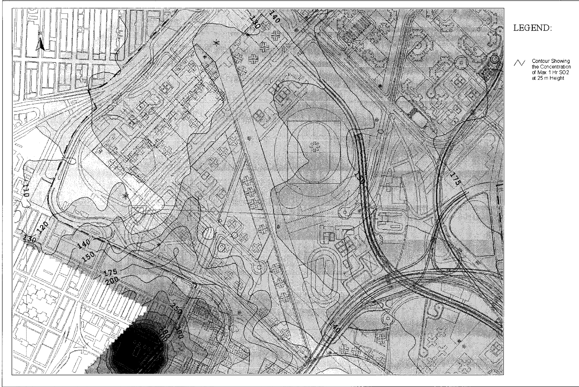
Drawing No. 22936/EN/329B Predicted Worst-case 1-hr Average SO 2 Concentration Contours at 25m Above Ground
