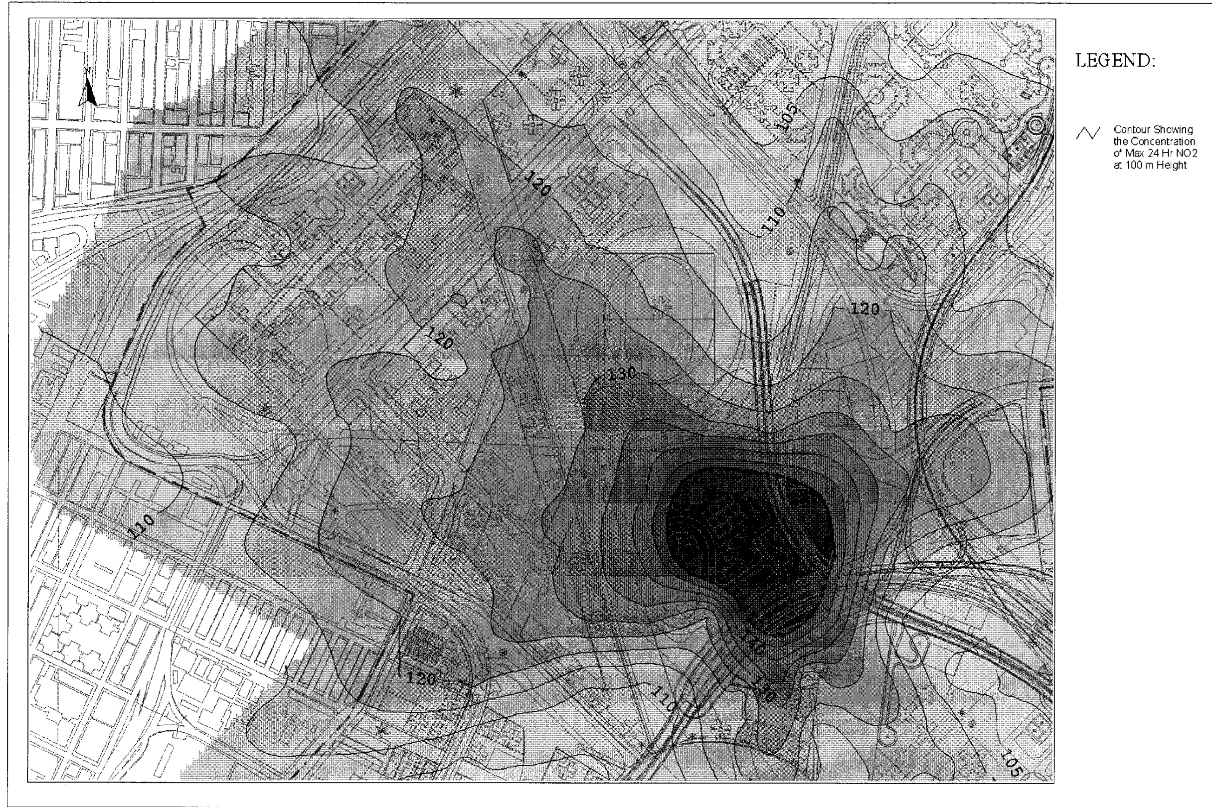
Drawing No. 22936/EN/327B Predicted Worst-case 24-hr Average NO 2 Concentration Contours at 100m Above Ground
