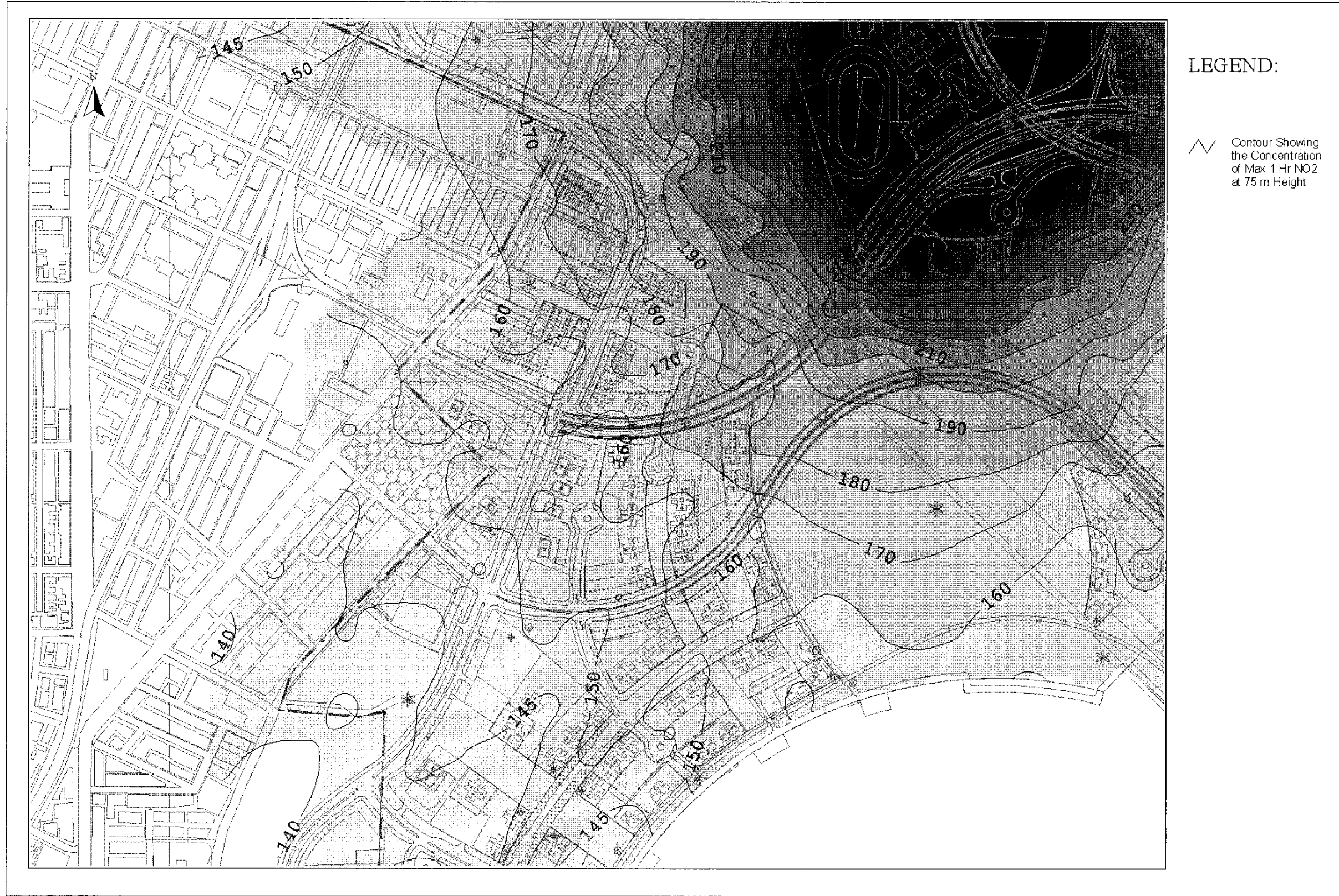
Drawing No. 22936/EN/320C Predicted Worst-case 1-hr Average NO 2 Concentration Contours at 75m Above Ground
