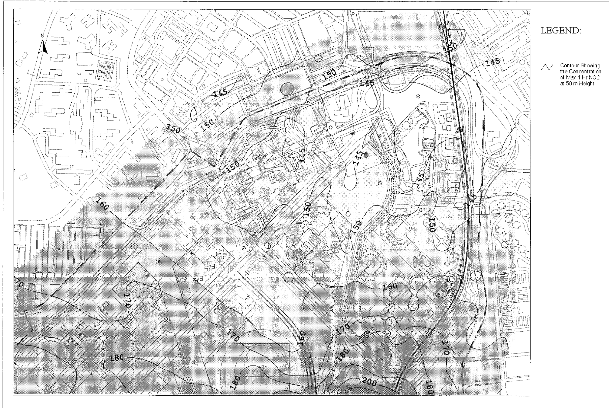
Drawing No. 22936/EN/319A Predicted Worst-case 1-hr Average NO 2 Concentration Contours at 50m Above Ground
