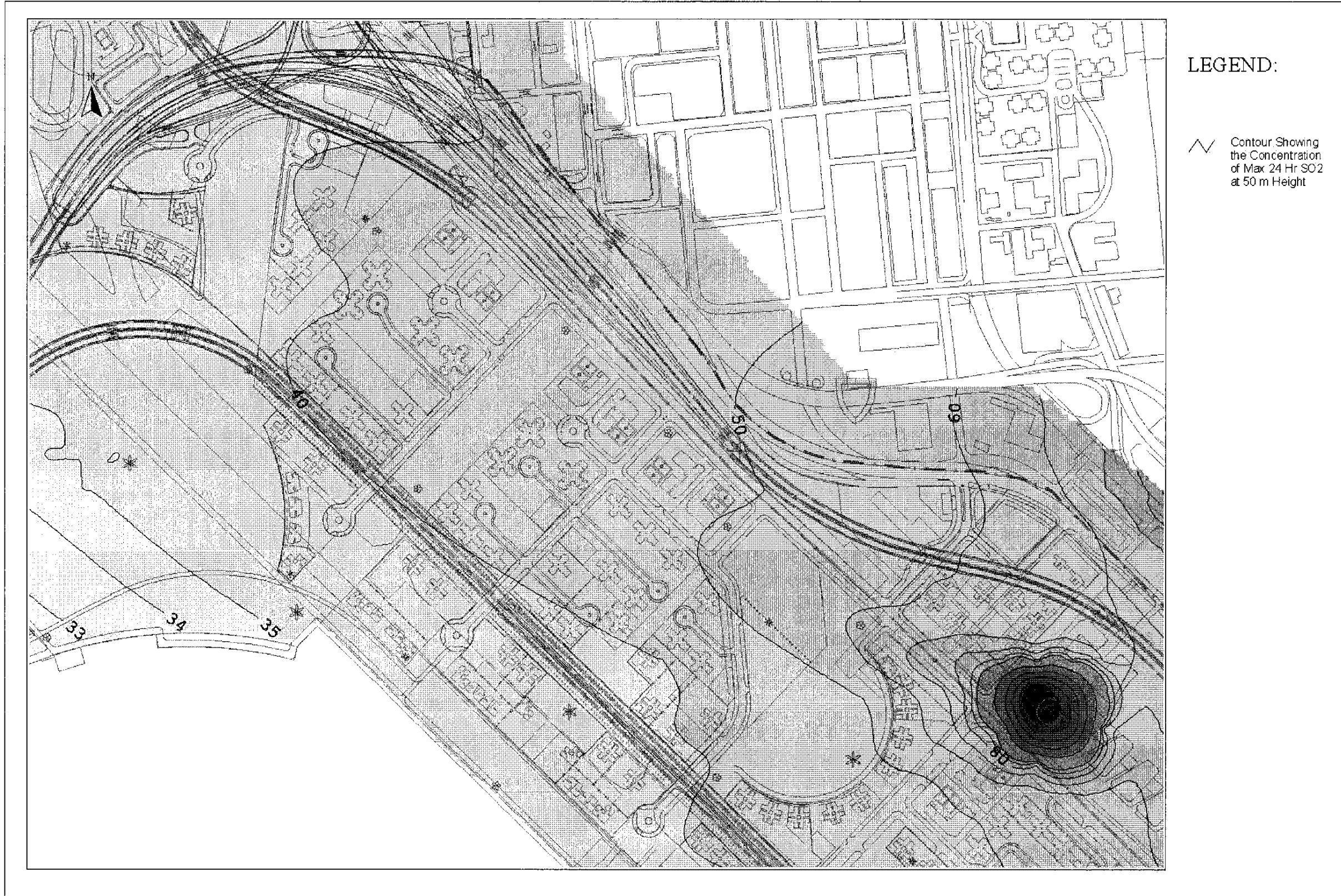
Drawing No. 22936/EN/334E Predicted Worst-case 24-hr Average SO 2 Concentration Contours at 50m Above Ground
