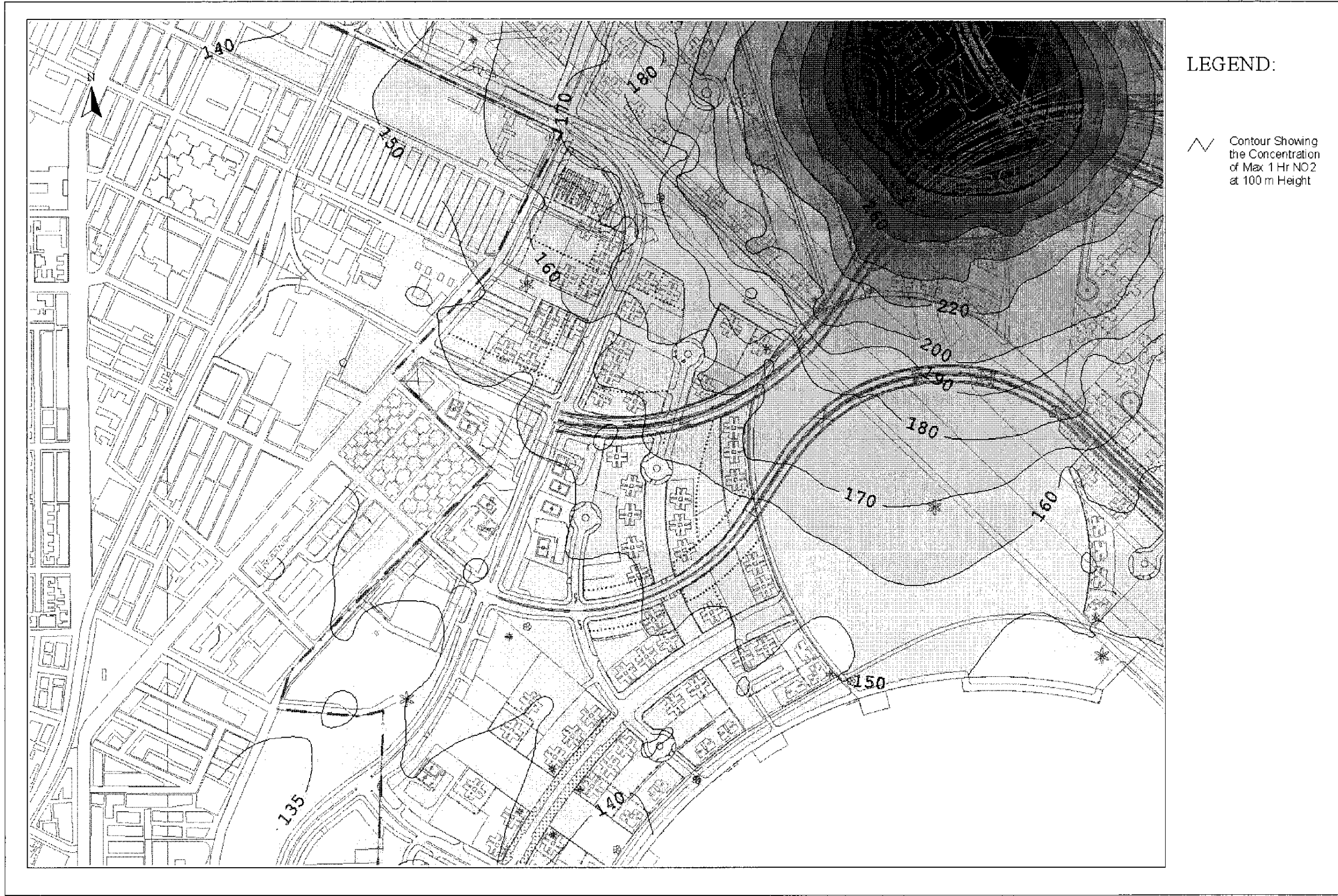
Drawing No. 22936/EN/321C Predicted Worst-case 1-hr Average NO 2 Concentration Contours at 100m Above Ground
