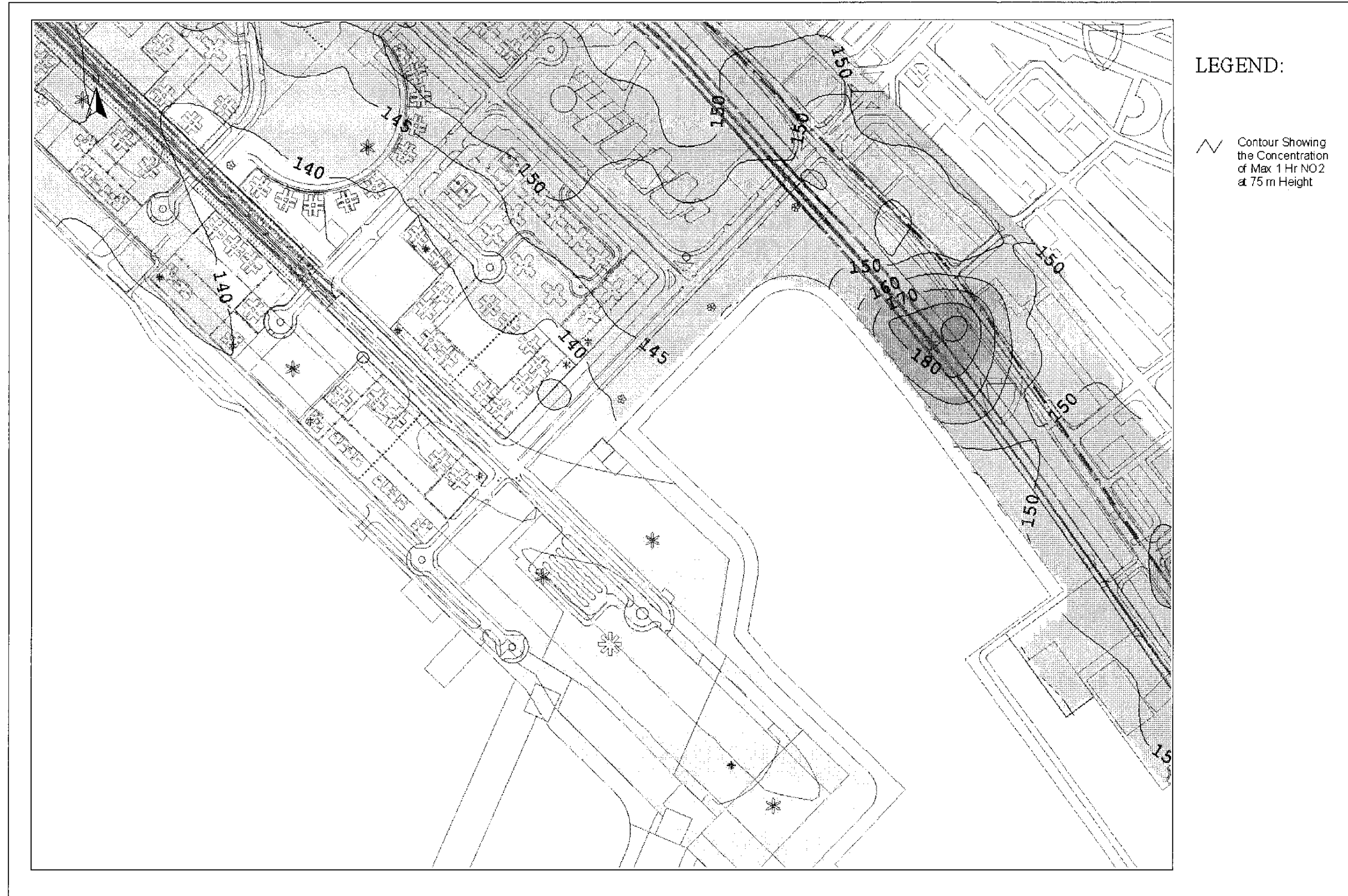
Drawing No. 22936/EN/320F Predicted Worst-case 1-hr Average NO 2 Concentration Contours at 75m Above Ground
