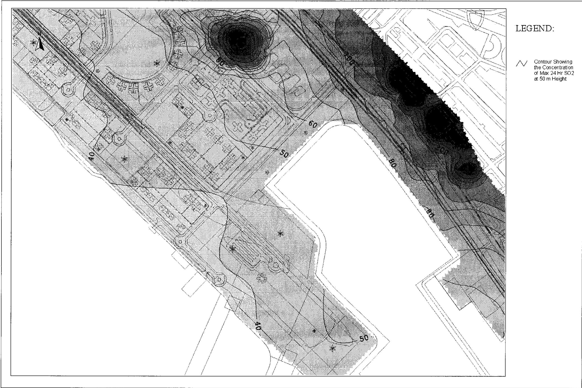
Drawing No. 22936/EN/334F Predicted Worst-case 24-hr Average SO2 Concentration Contours at 50m Above Ground
