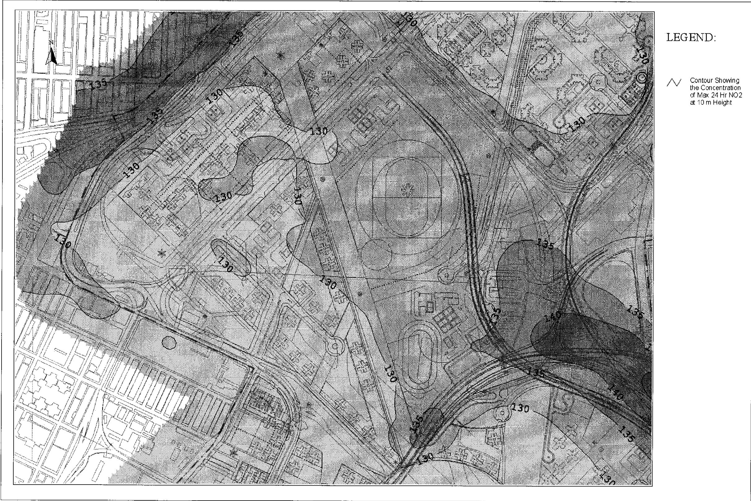
Drawing No. 22936/EN/323B Predicted Worst-case 24-hr Average NO 2 Concentration Contours at 10m Above Ground
