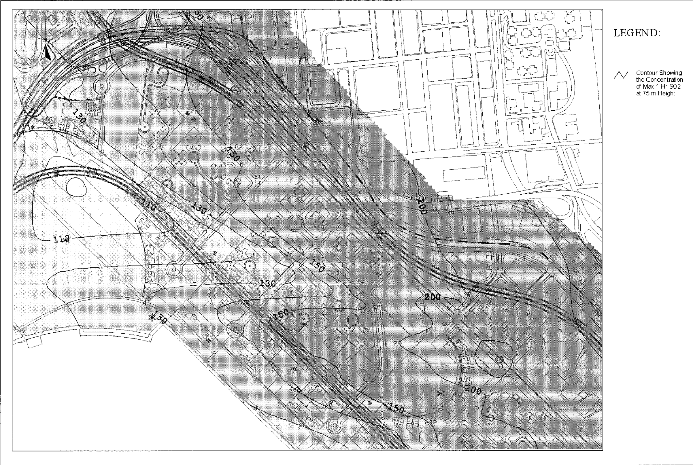
Drawing No. 22936/EN/331E Predicted Worst-case 1-hr Average SO2 Concentration Contours at 75m Above Ground
