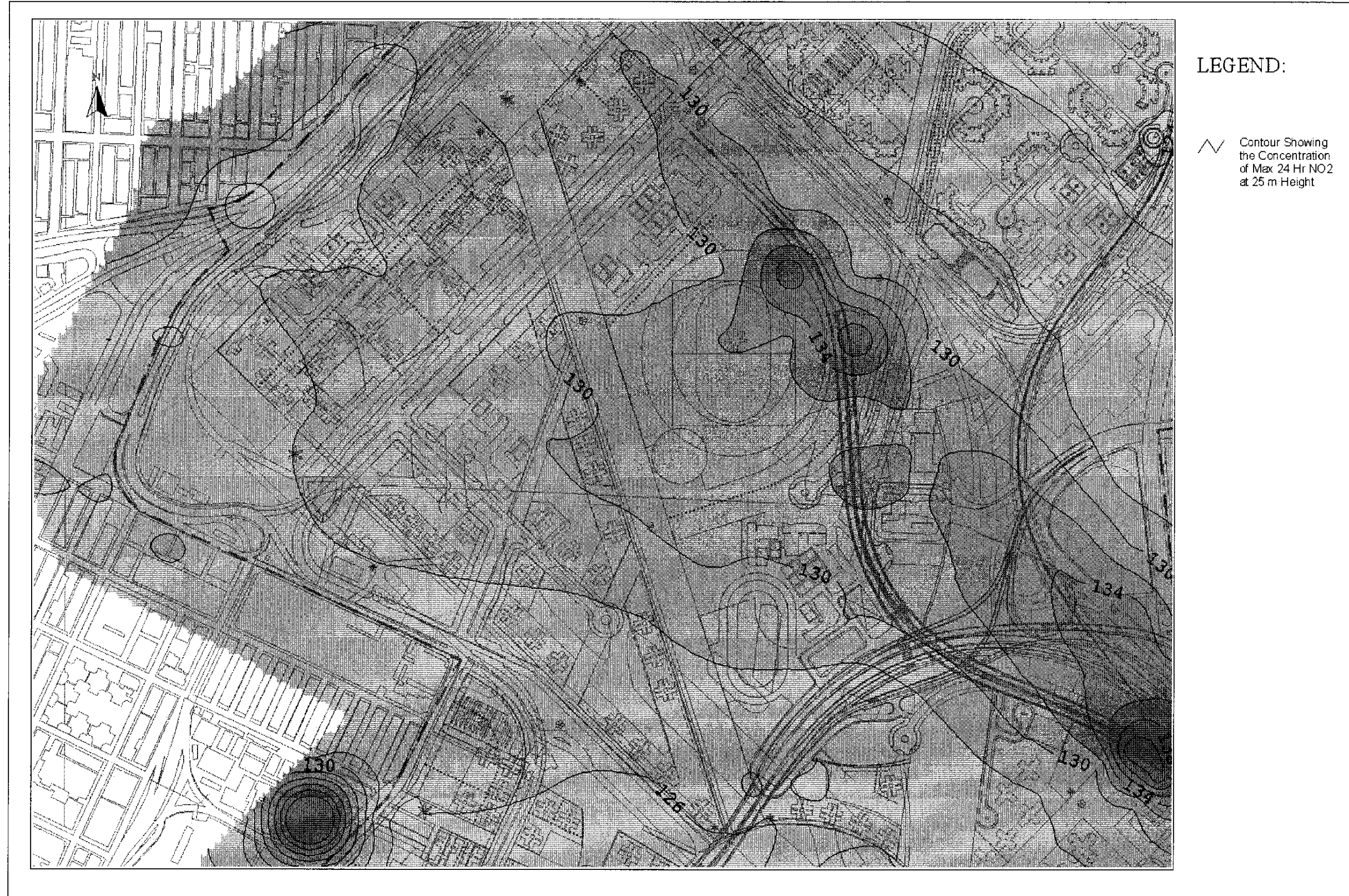
Drawing No. 22936/EN/324B Predicted Worst-case 24-hr Average NO 2 Concentration Contours at 25m Above Ground
