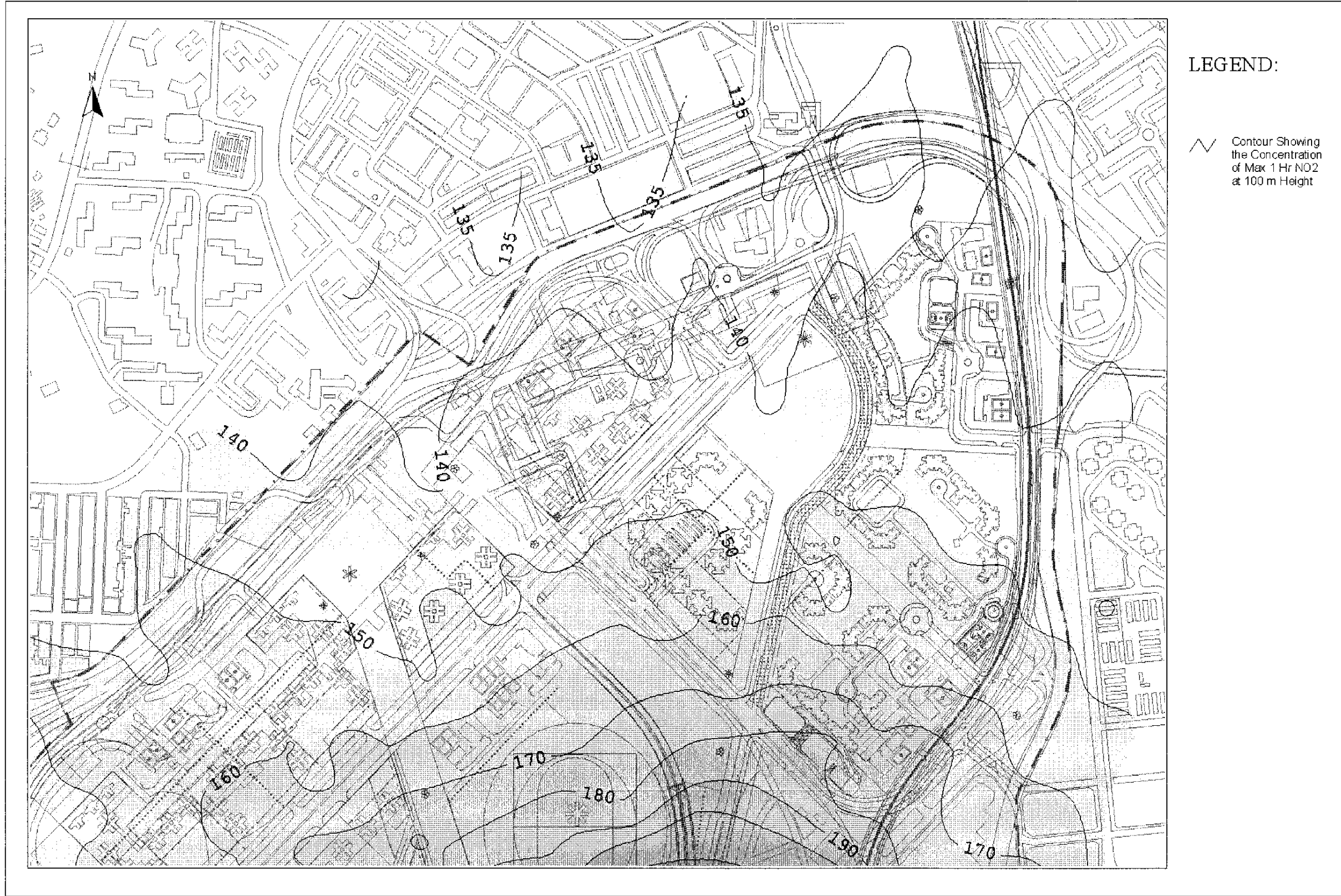
Drawing No. 22936/EN/321A Predicted Worst-case 1-hr Average NO 2 Concentration Contours at 100m Above Ground
