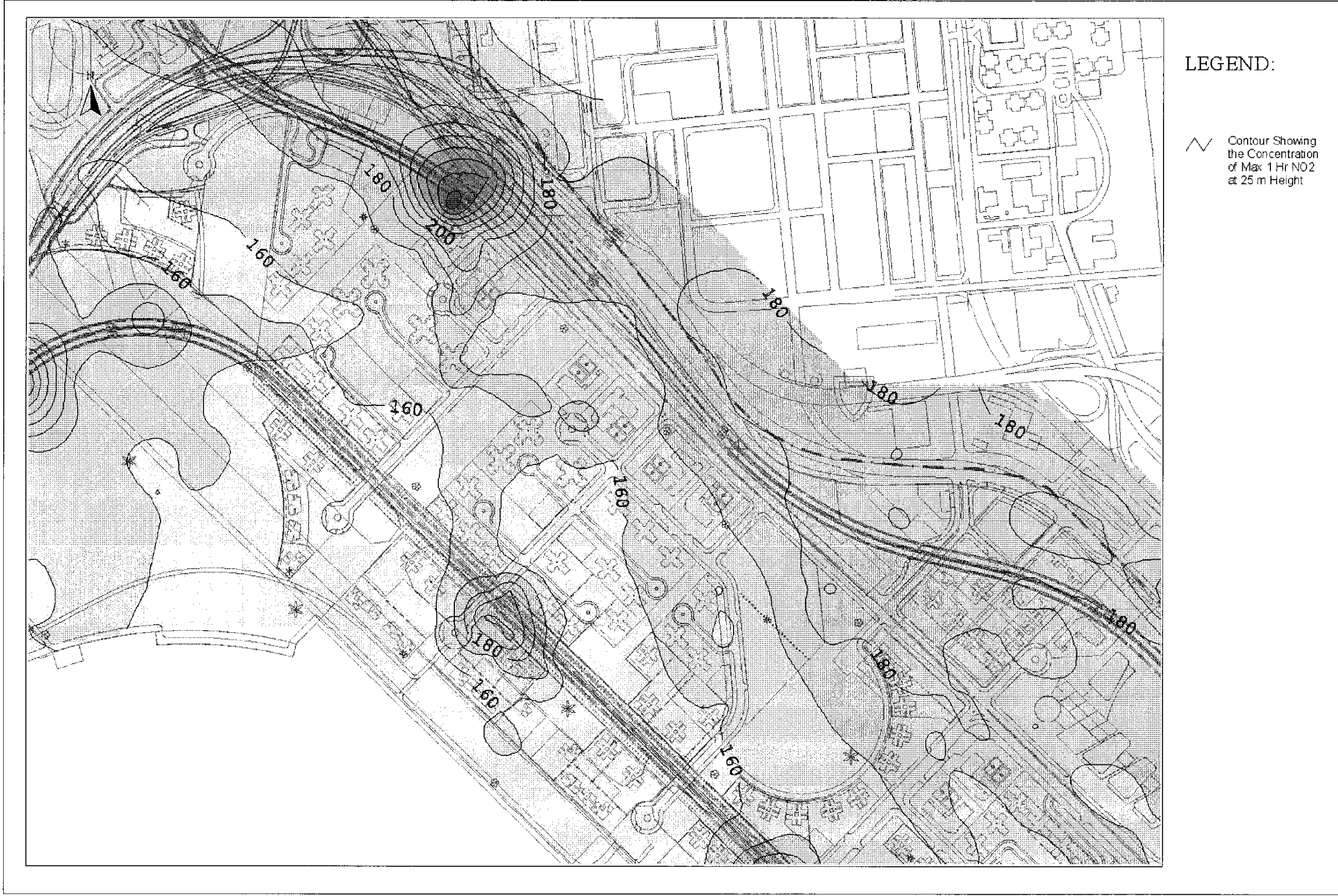
Drawing No. 22936/EN/318E Predicted Worst-case 1-hr Average NO 2 Concentration Contours at 25m Above Ground
