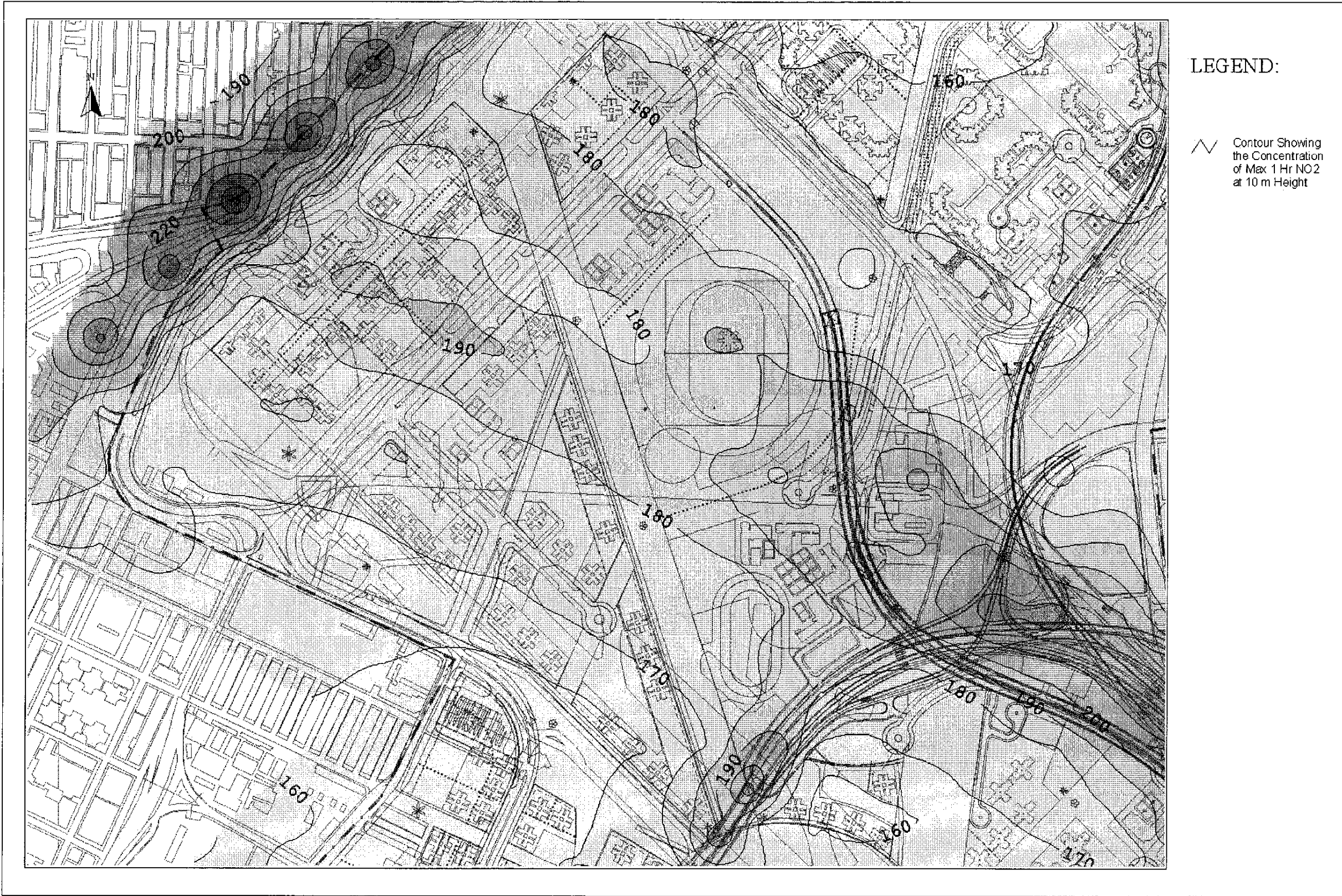
Drawing No. 22936/EN/317B Predicted Worst-case 1-hr Average NO 2 Concentration Contours at 10m Above Ground
