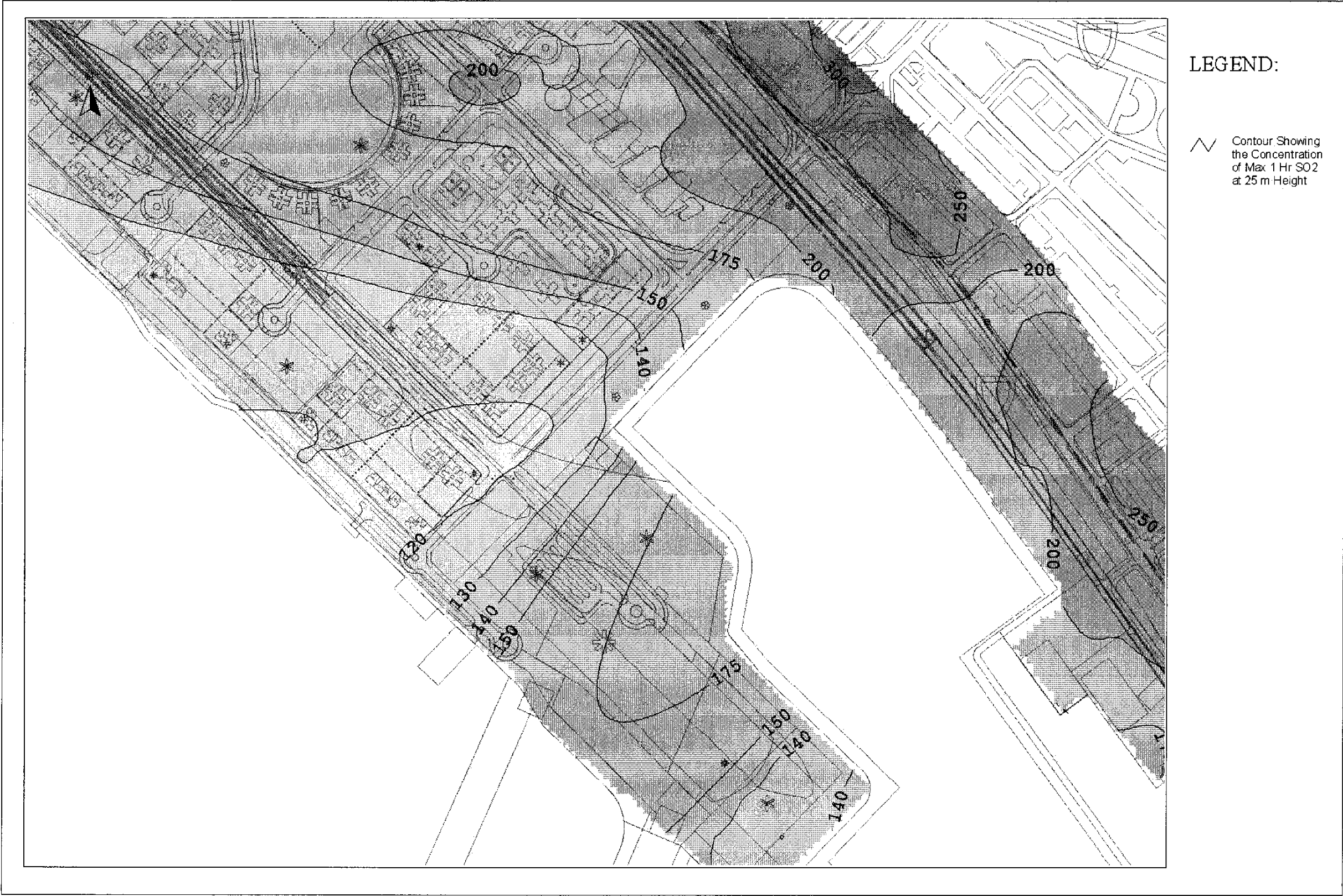
Drawing No. 22936/EN/329F Predicted Worst-case 1-hr Average SO 2 Concentration Contours at 25m Above Ground
