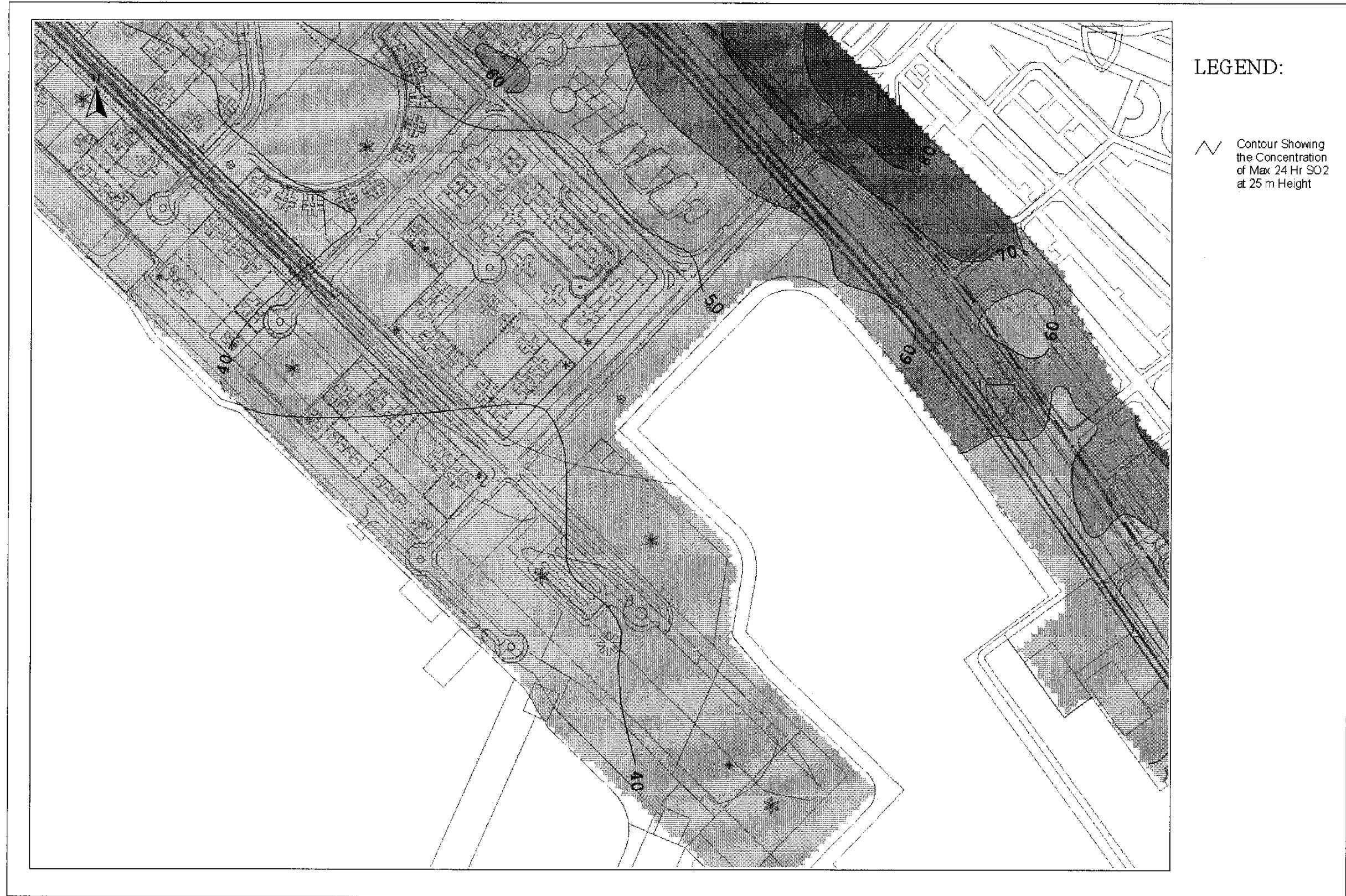
Drawing No. 22936/EN/333F Predicted Worst-case 24-hr Average SO 2 Concentration Contours at 25m Above Ground
