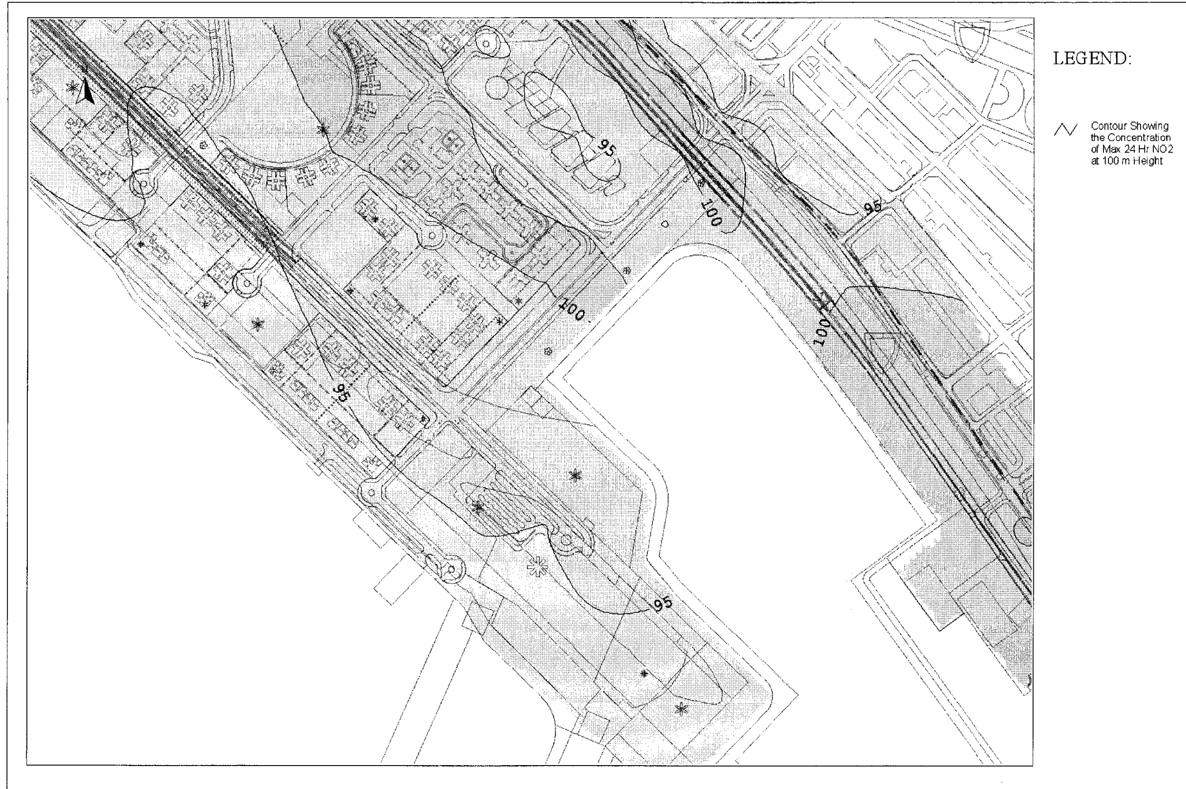
Drawing No. 22936/EN/327F Predicted Worst-case 24-hr Average NO 2 Concentration Contours at 100m Above Ground
