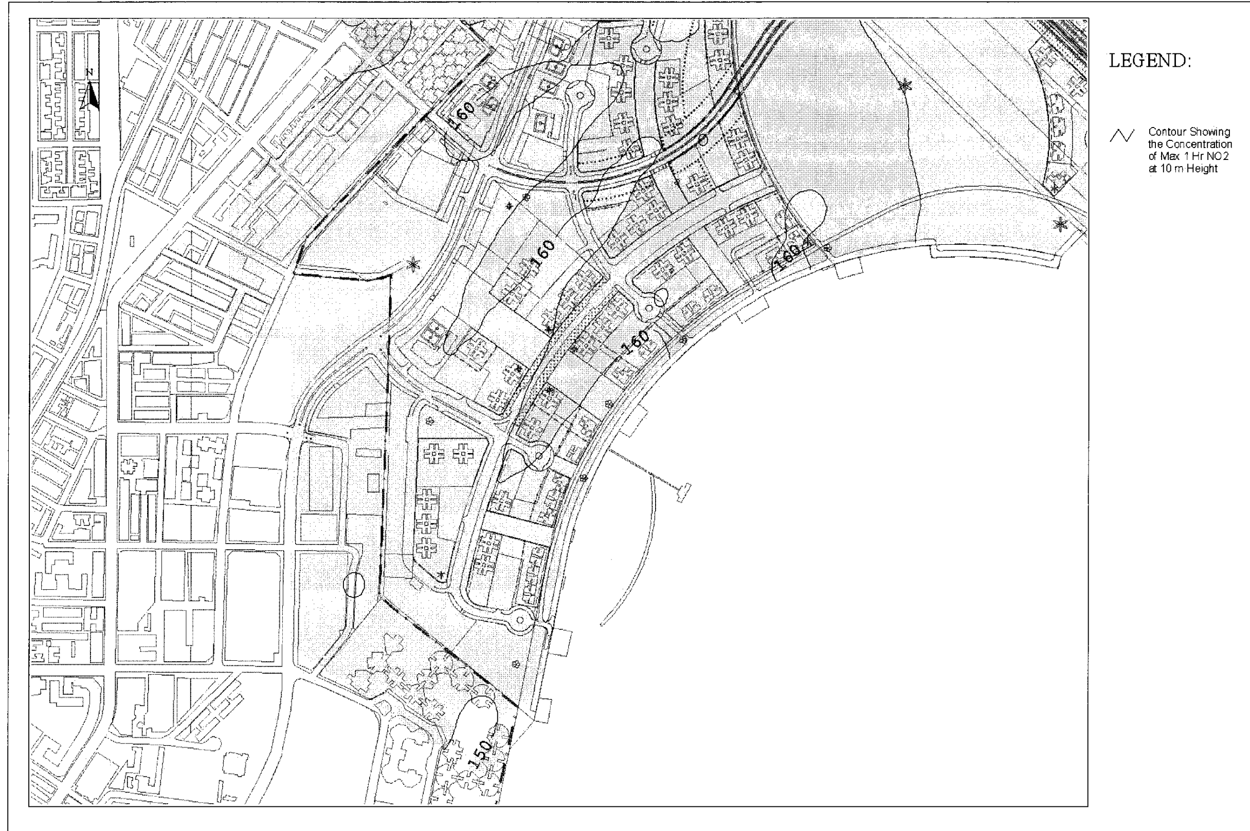
Drawing No. 22936/EN/317D Predicted Worst-case 1-hr Average NO 2 Concentration Contours at 10m Above Ground
