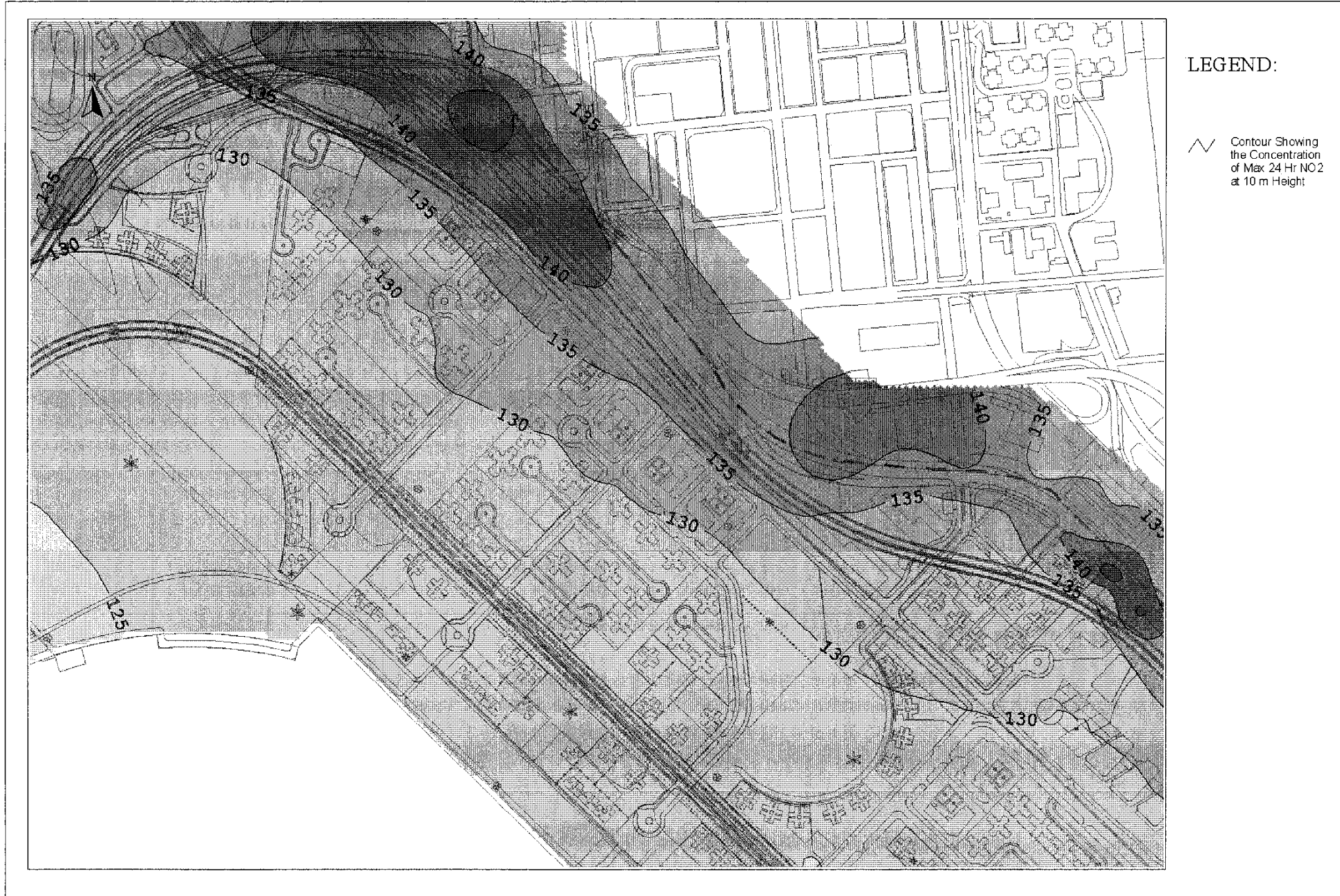
Drawing No. 22936/EN/323E Predicted Worst-case 24-hr Average NO 2 Concentration Contours at 10m Above Ground
