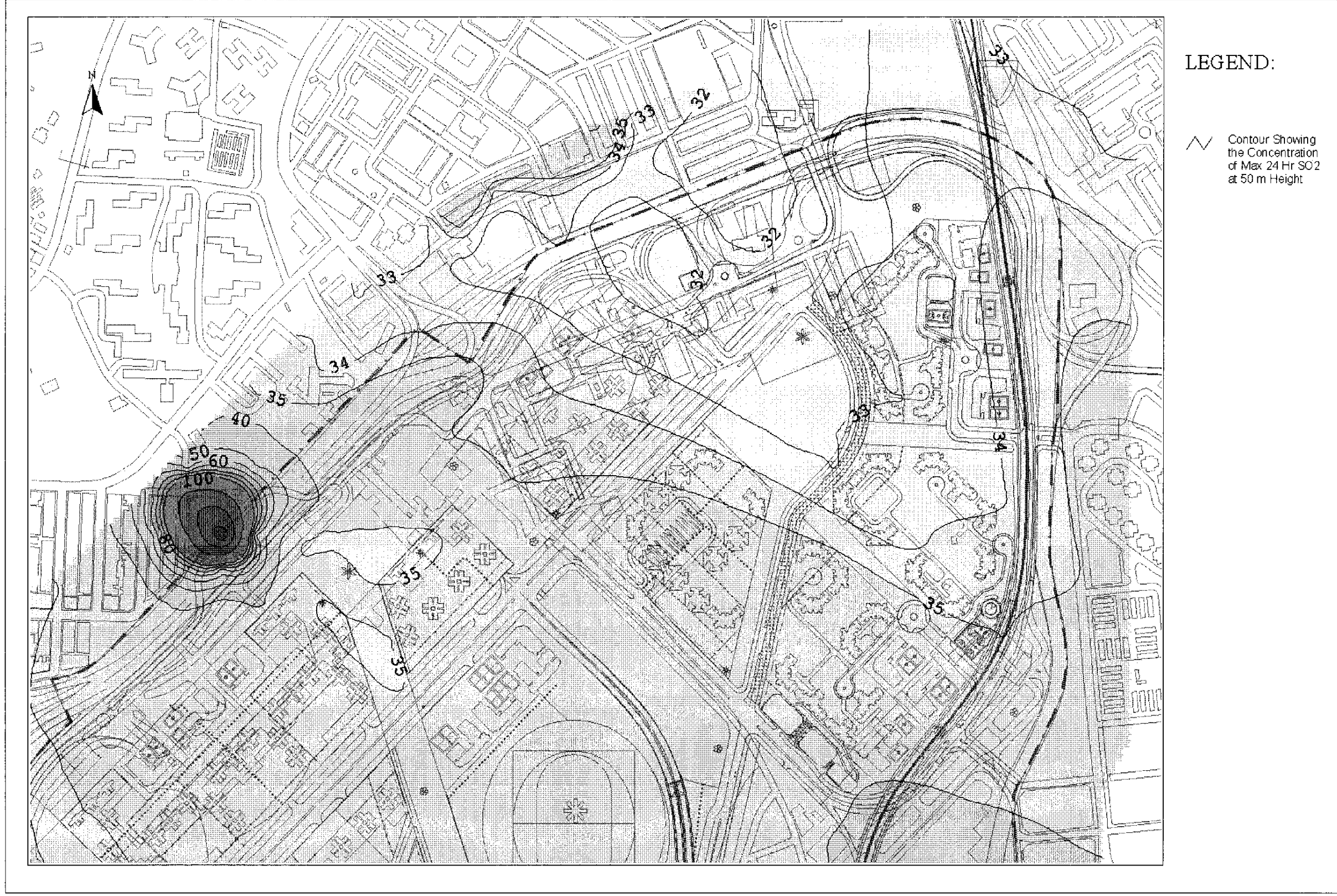
Drawing No. 22936/EN/334A Predicted Worst-case 24-hr Average SO 2 Concentration Contours at 50m Above Ground
