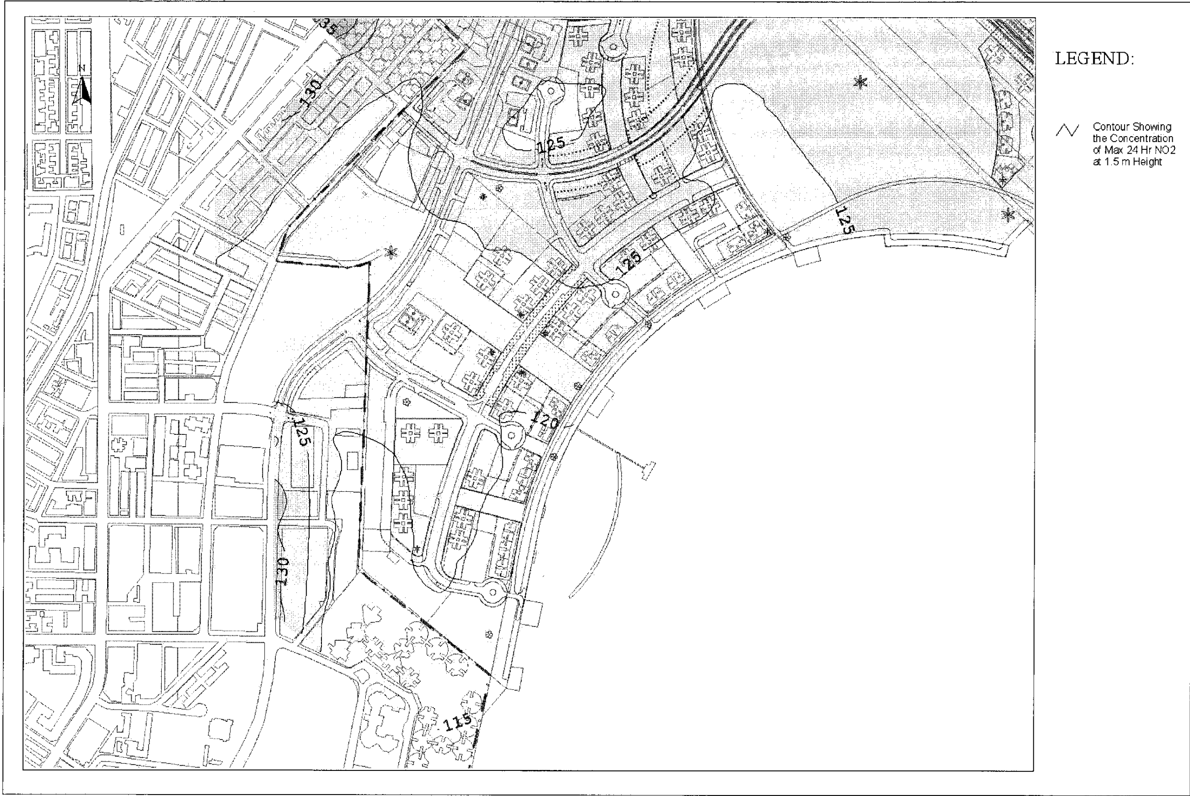
Drawing No. 22936/EN/322D Predicted Worst-case 24-hr Average NO 2 Concentration Contours at 1.5m Above Ground
