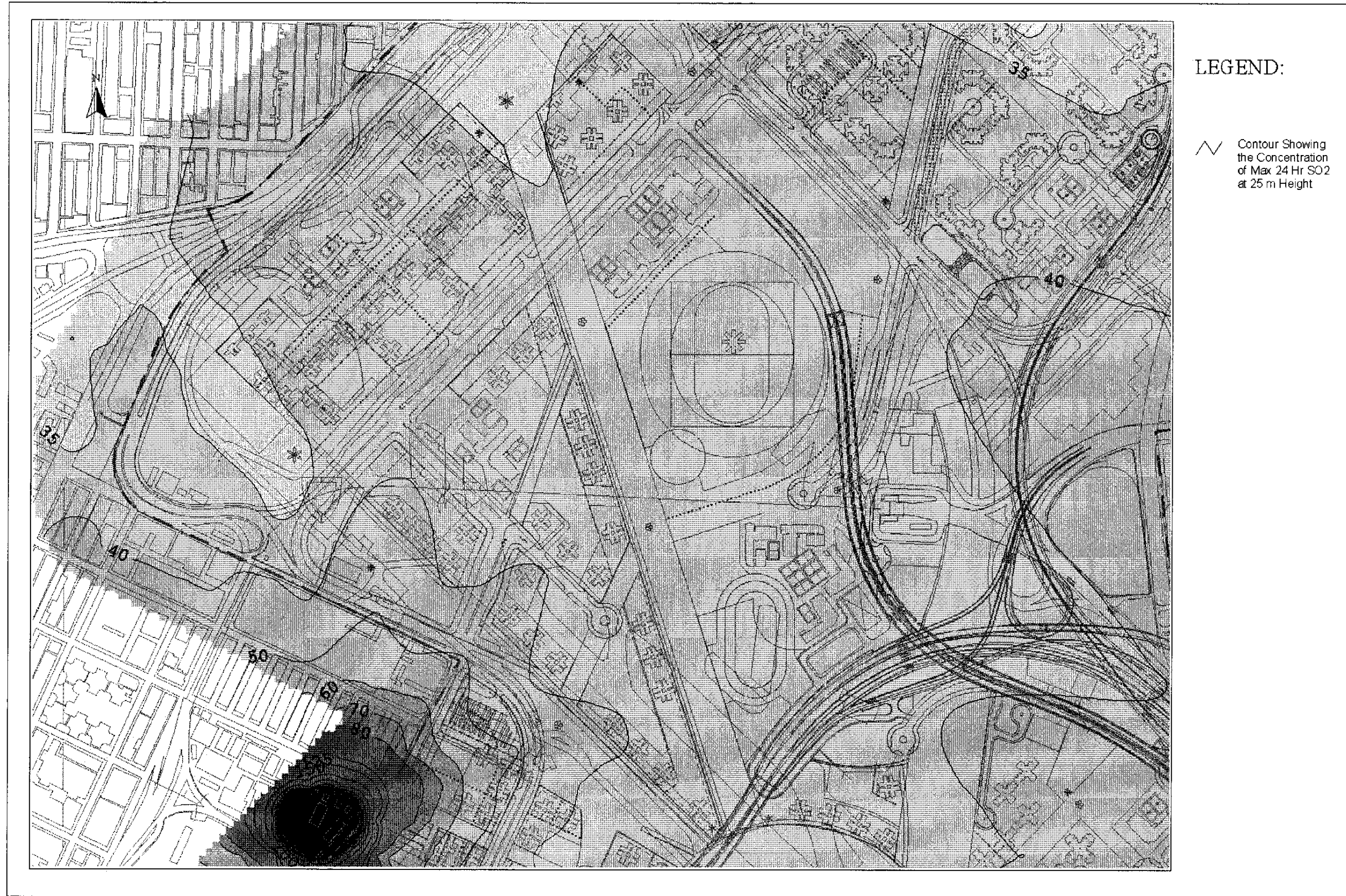
Drawing No. 22936/EN/333B Predicted Worst-case 24-hr Average SO2 Concentration Contours at 25m Above Ground
