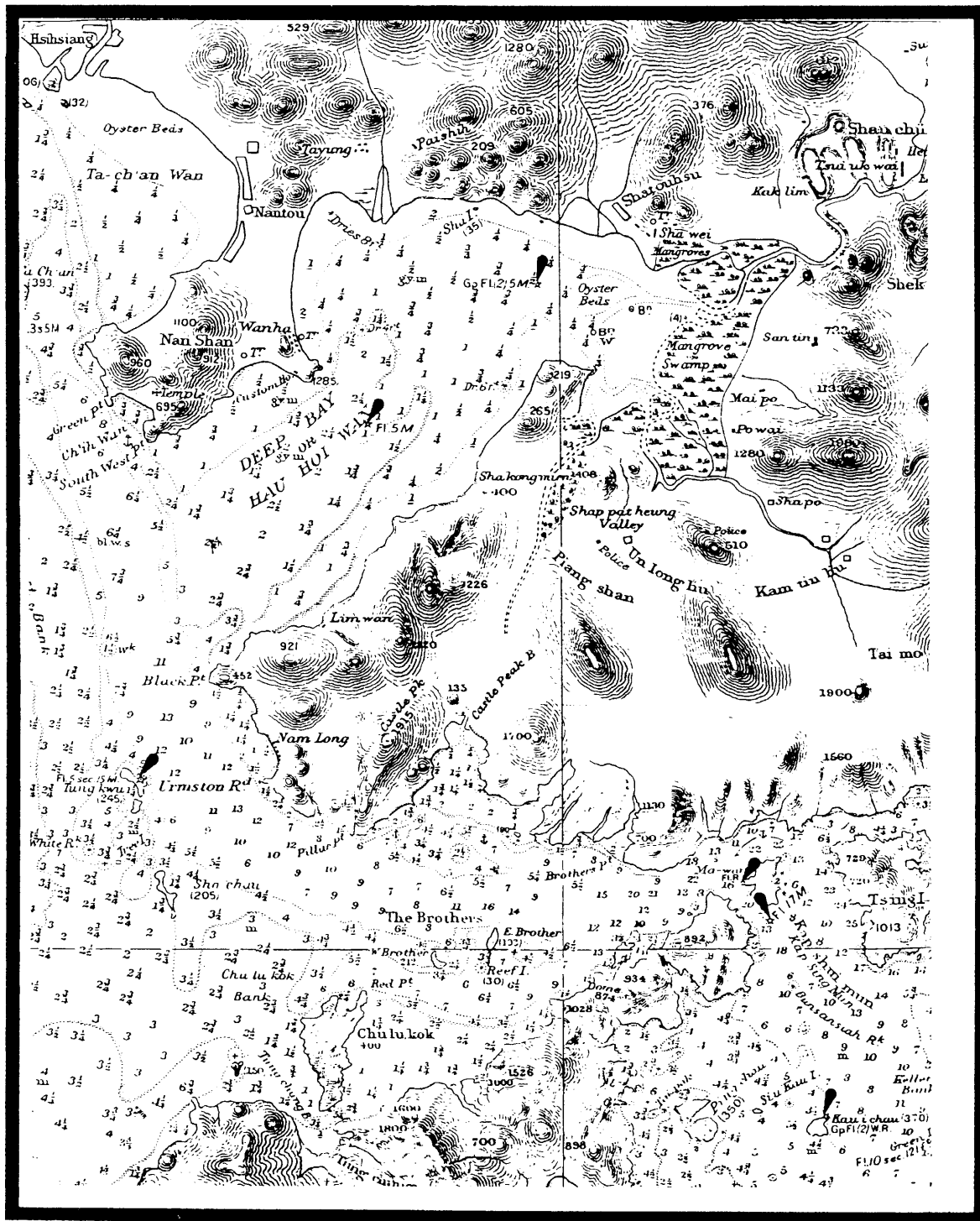
Figure 12.10 British Admiralty Chart 1966
