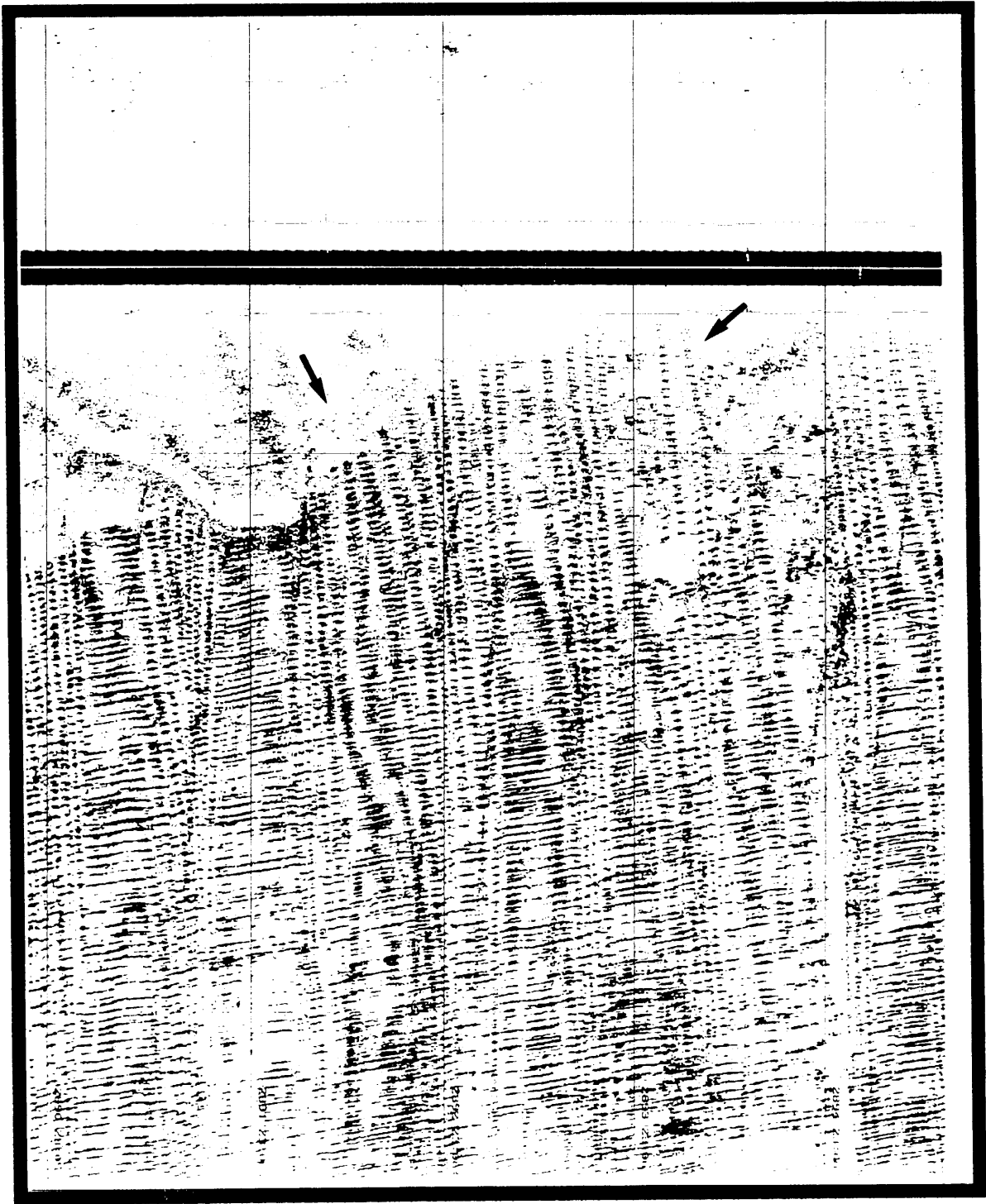
Figure 12.12 Side Scan Sonar Data Showing Oyster Beds on the Seabed
