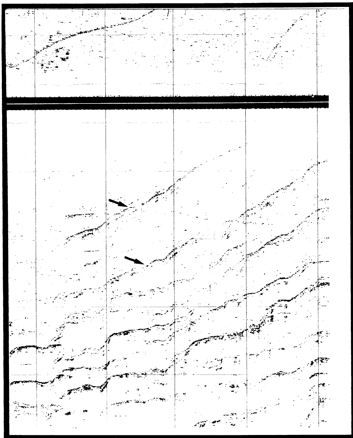
Figure 12.13 Side Scan Sonar Data Showing Deeply Incised Trawl Scars
