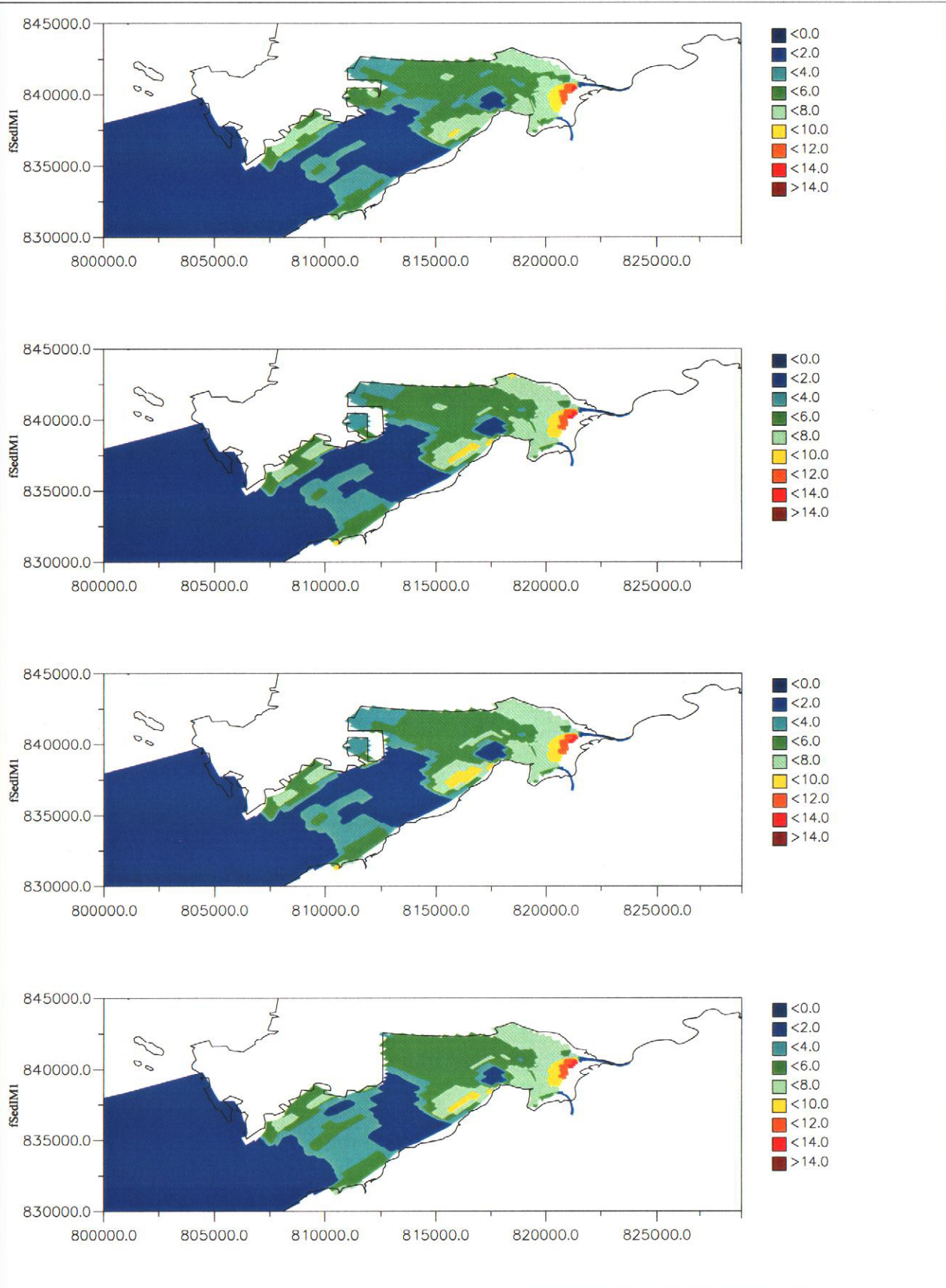
Shenzhen Western Corridor Sedimentation Flux (g/sq. m/d); Dry Season Spring Tide;Mid Ebb Top: Scenario 1; Upper: Scenario 2; Lower: Scenario 3; Bottom: Scenario 4
