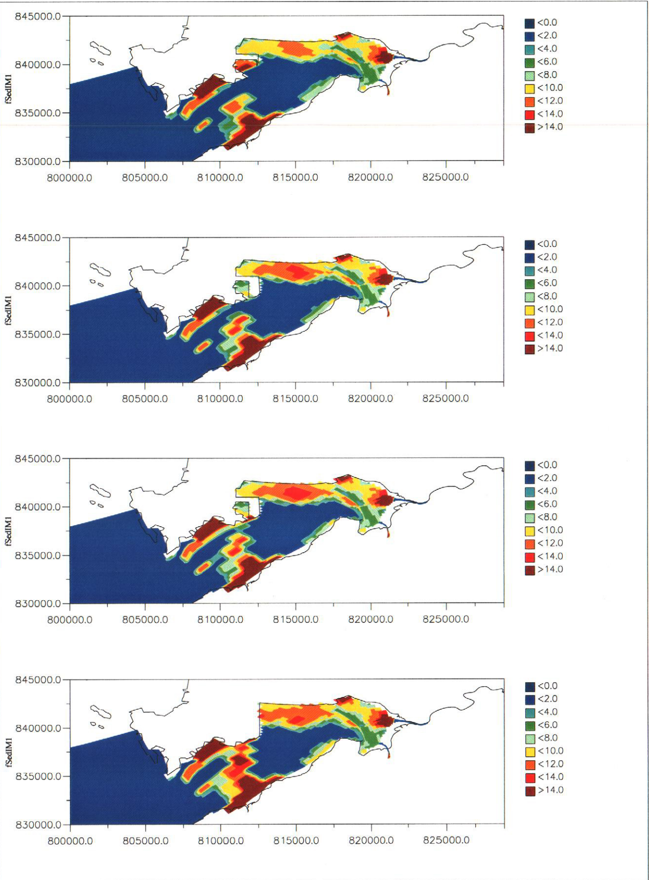
Shenzhen Western Corridor Sedimentation Flux (g/sq. m/d); Wet Season Spring Tide;Mid Ebb Top: Scenario 1; Upper: Scenario 2; Lower: Scenario 3; Bottom: Scenario 4
