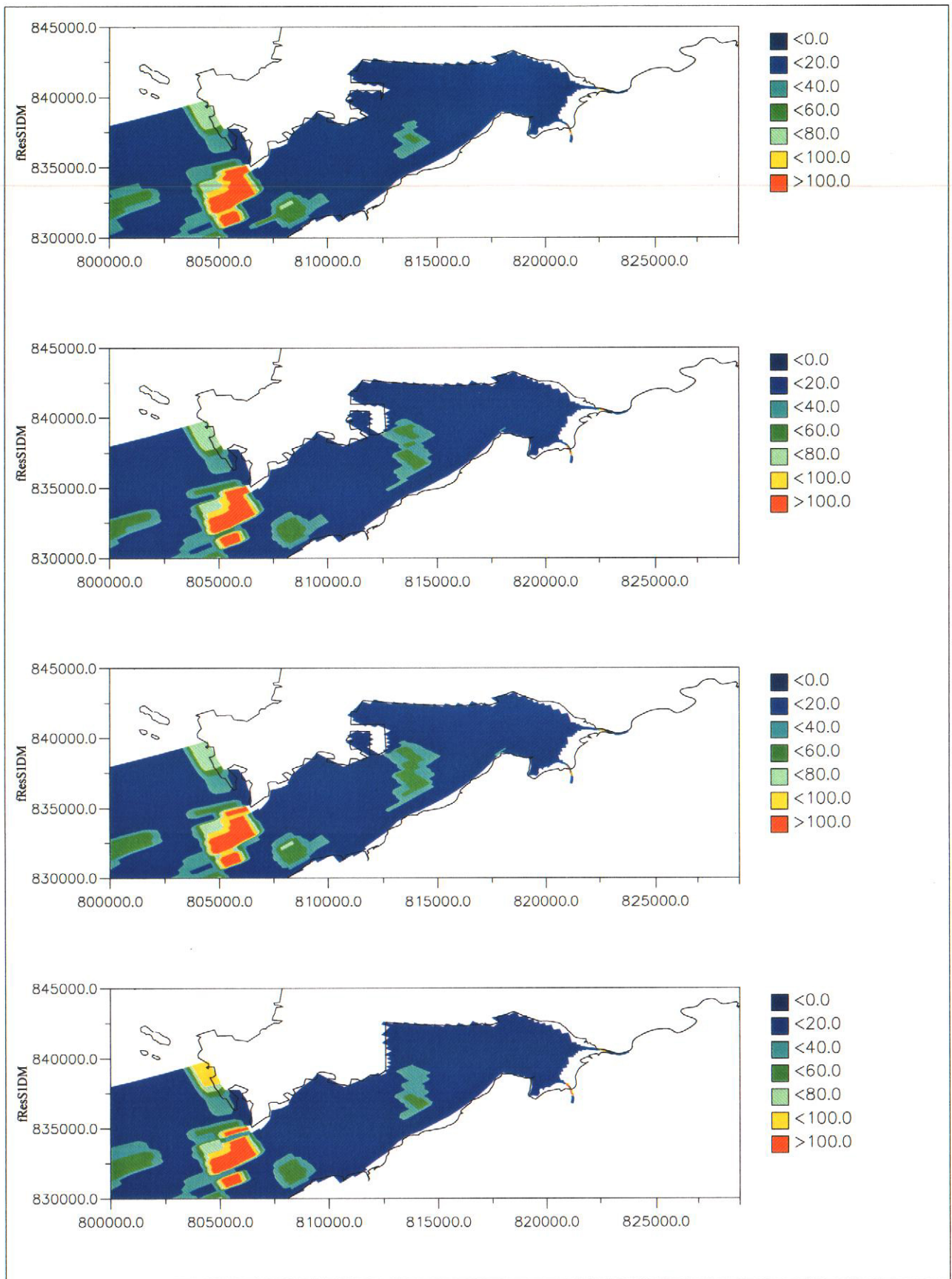
Shenzhen Western Corridor Resuspension Flux(g/sq. m/d);Wet Season Spring Tide;Mid Flood Top: Scenario 1; Upper: Scenario 2; Lower: Scenario 3; Bottom: Scenario 4 Wet Season August 2002 Figure 7.111 Ove Arup & Partners Hong Kong Ltd
