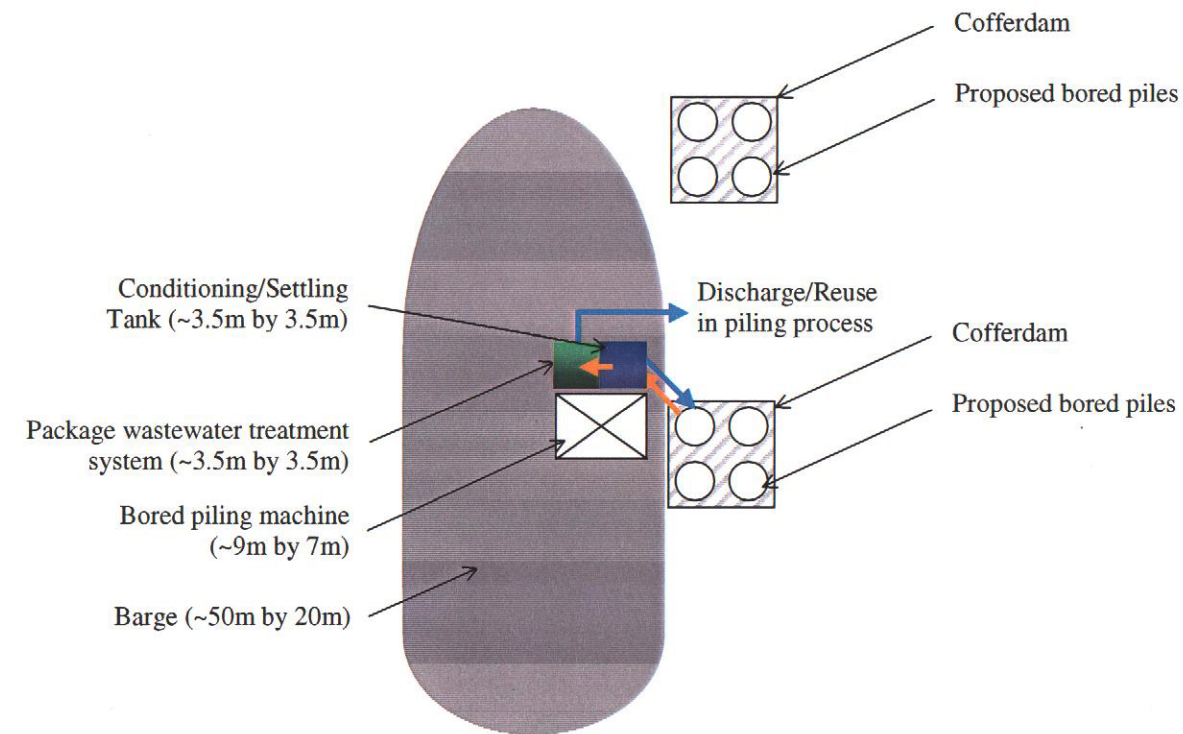
(c) Bored Piling in Deep Water Region
