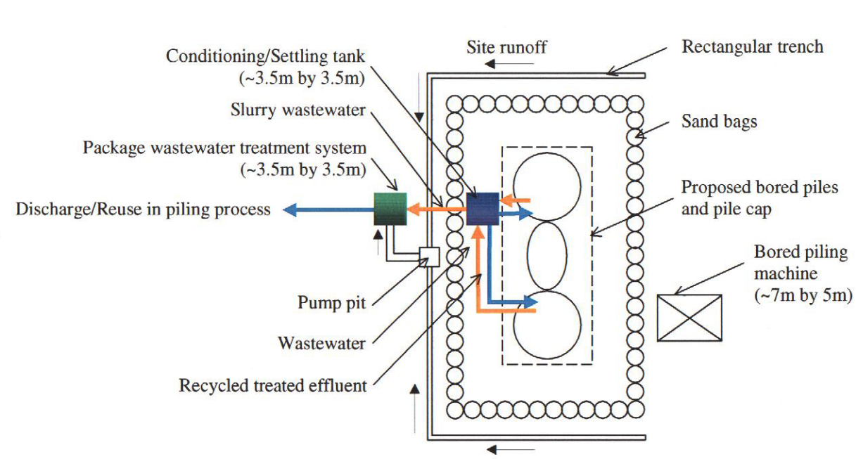
(a) Bored Piling Site near Local Stream Course within Works Area at Ngau Hom Shek (Under DBL Project)
