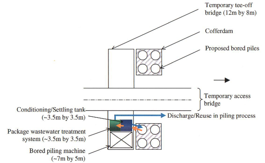
(b) Bored Piling in Shallow Water Region
