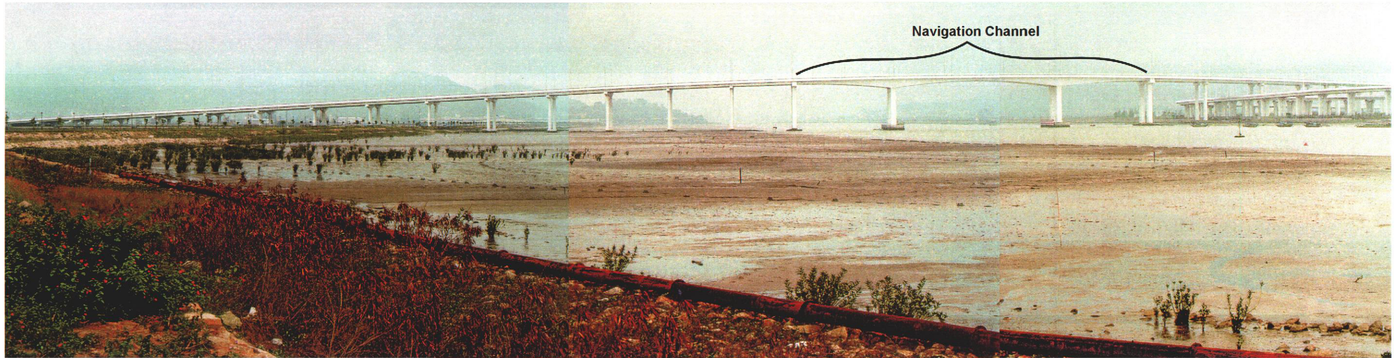
a Lotus Bridge in Macau SAR as seen in un-modified photograph taken from 600m north of the bridge on 28 March 2002. Pier spacing left (east) of the navigation channel across the mudflat is 35m, less than half of the 75m proposed for the SWC bridge.
