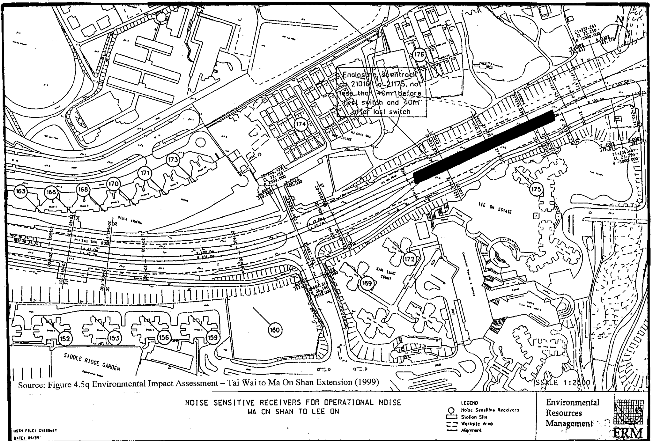
Figure 3.7.1a Mitigation Measure (Enclosure) proposed on MOS Rail Viaduct next to Lee On Estate by MOS EIA
