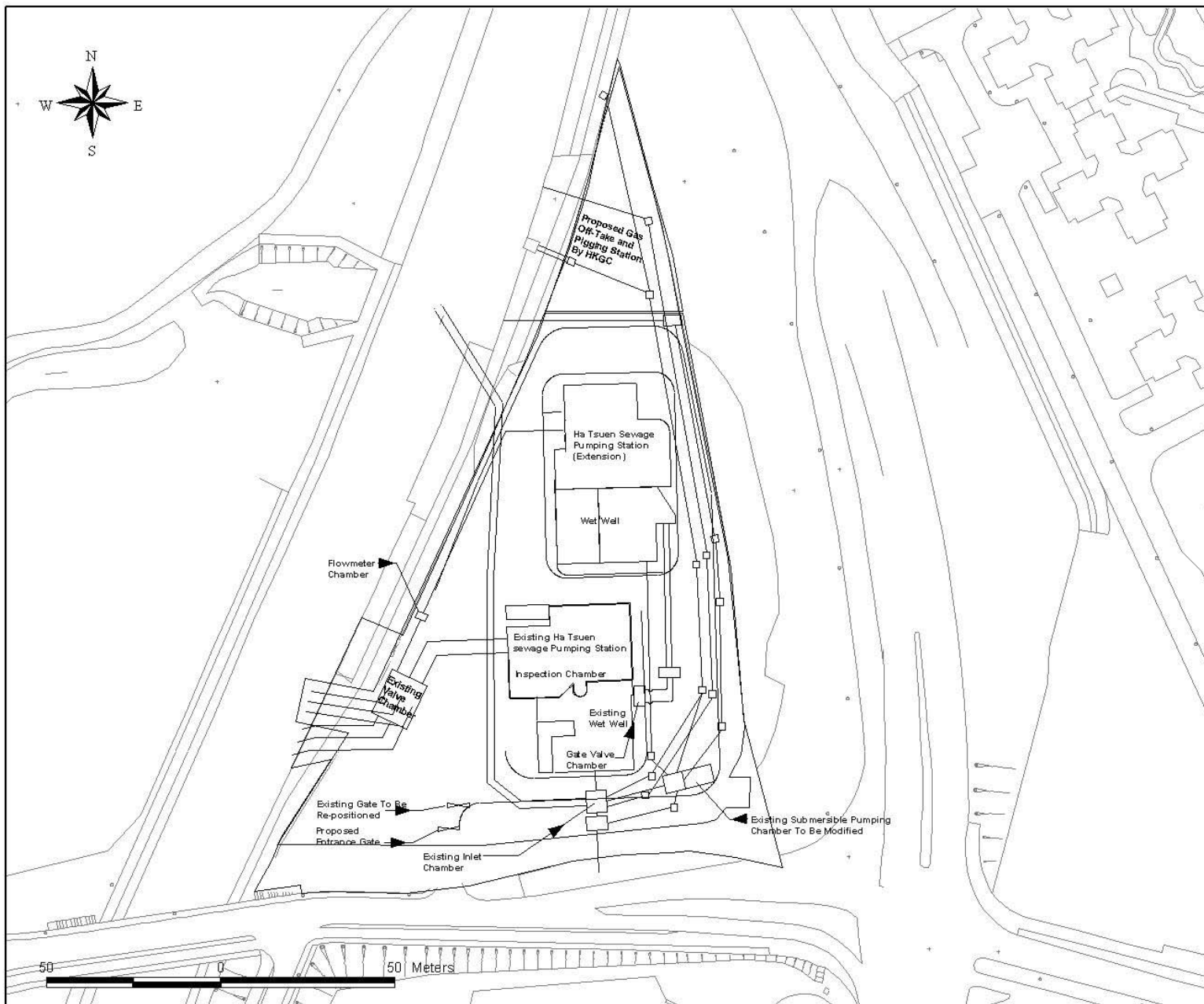
Figure 5 The Preliminary Layout Plan of the Proposed Expanded Ha Tsuen PS
