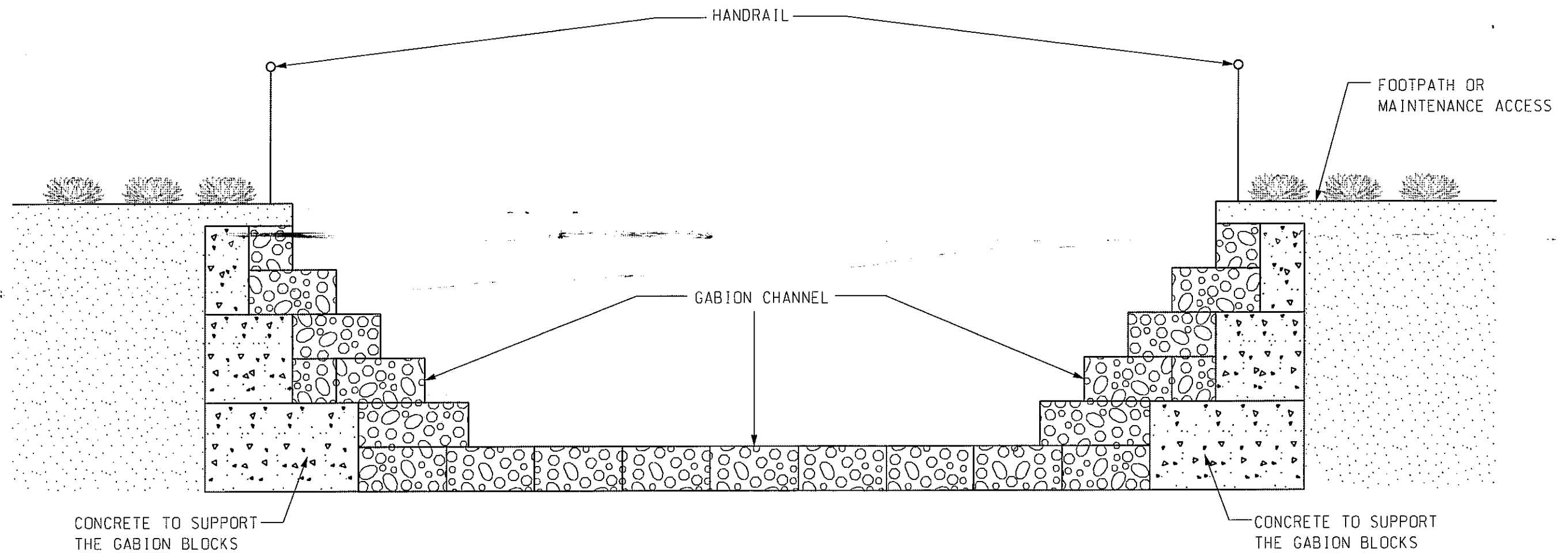
TRAPEZOIDAL CHANNEL WITH GABION BASE AND BANK N.T.S.
