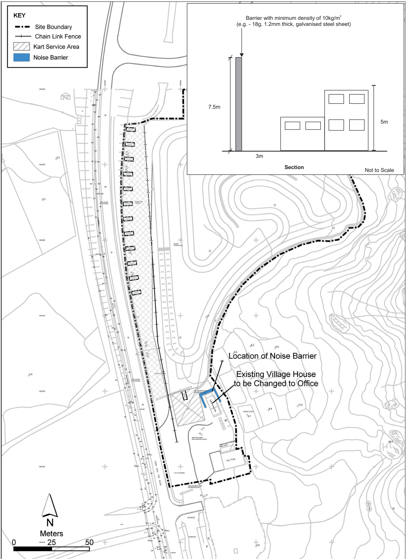
Layout Plan of Karting Track & Location of Noise Barrier
