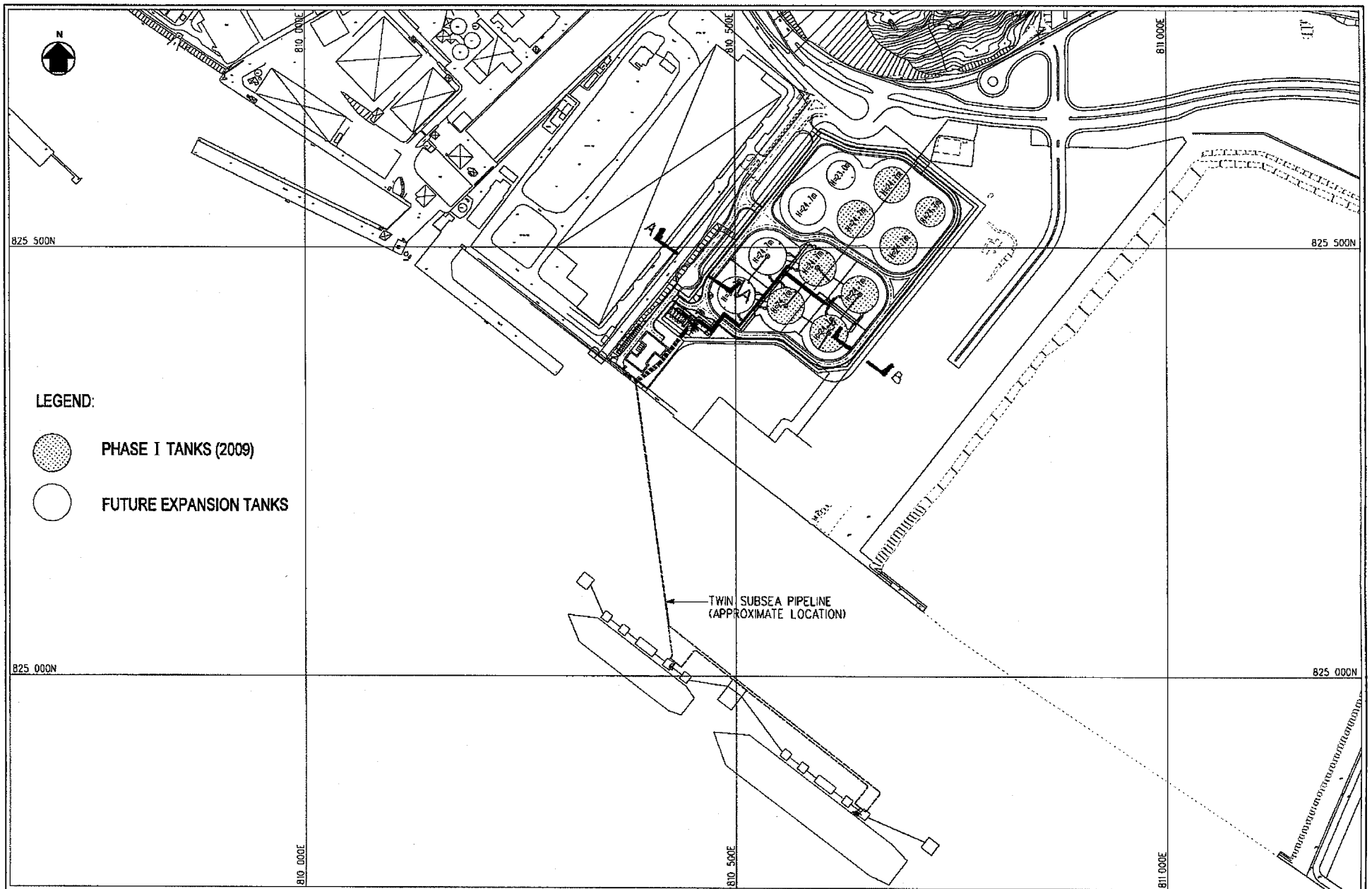
CONCEPT LAYOUT OF PERMANENT AVIATION FUEL FACILITY TANK FARM AND JETTY WITHIN TUEN MUN AREA 38
