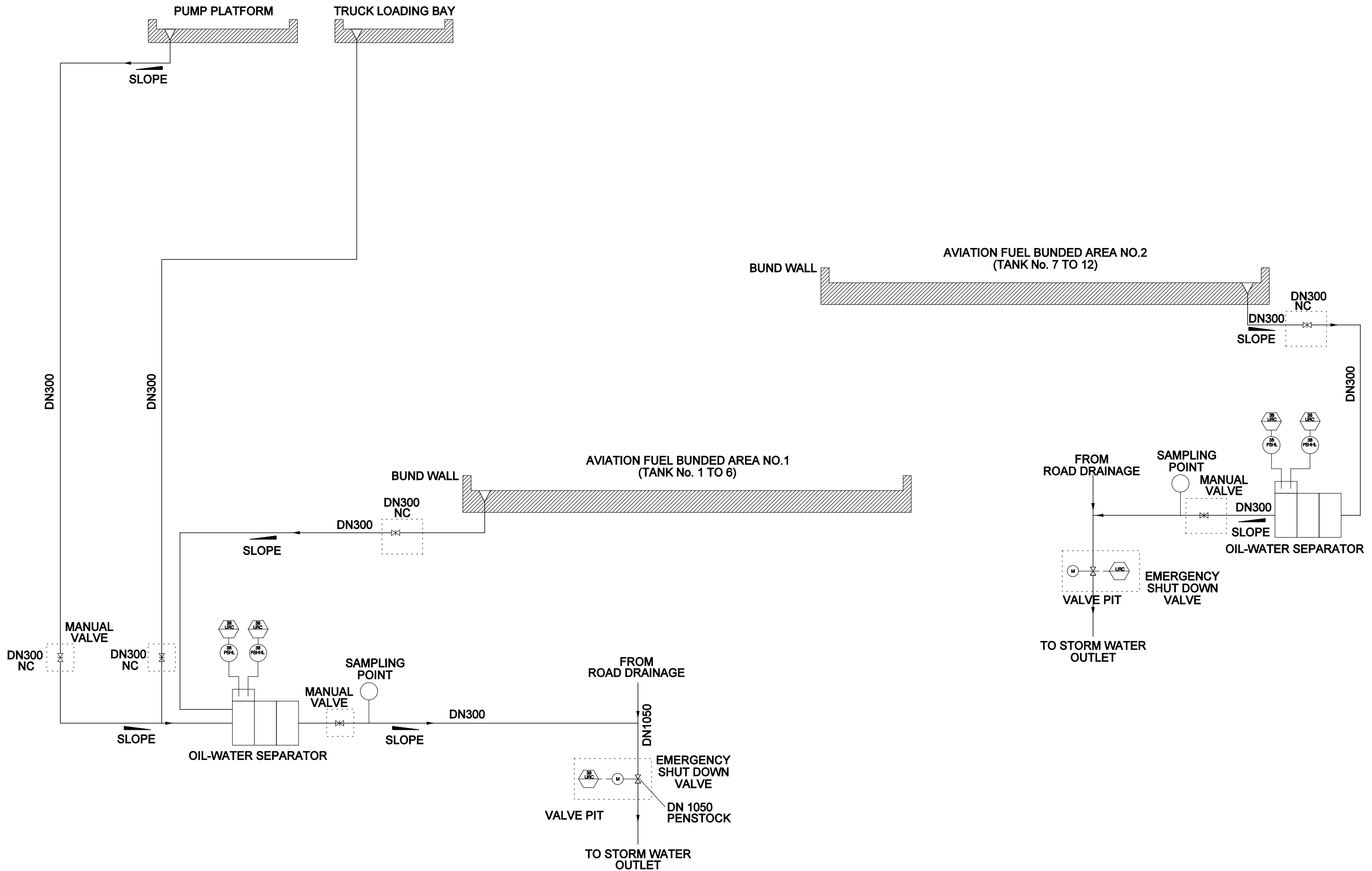
Schematic Diagram - Storm Water Drainage of Tankfarm and Tanks Banded Areas
