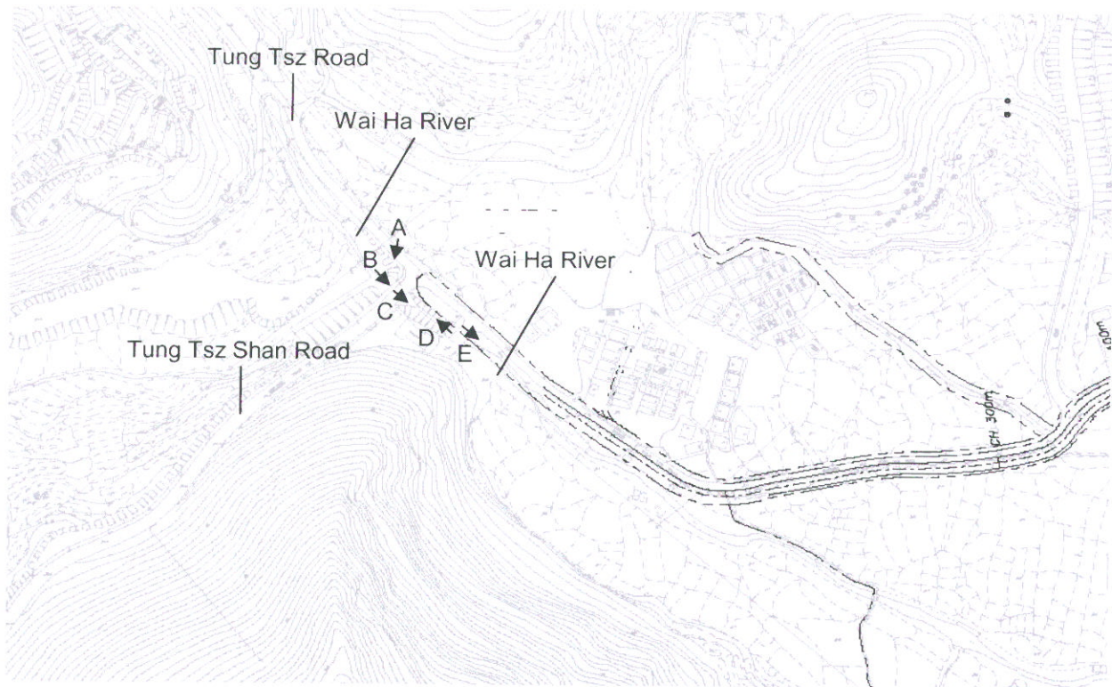
Viewing Points (A to E) along the Intercept Point of Wai Ha River and the Proposed Twin Cell Box Culvert
