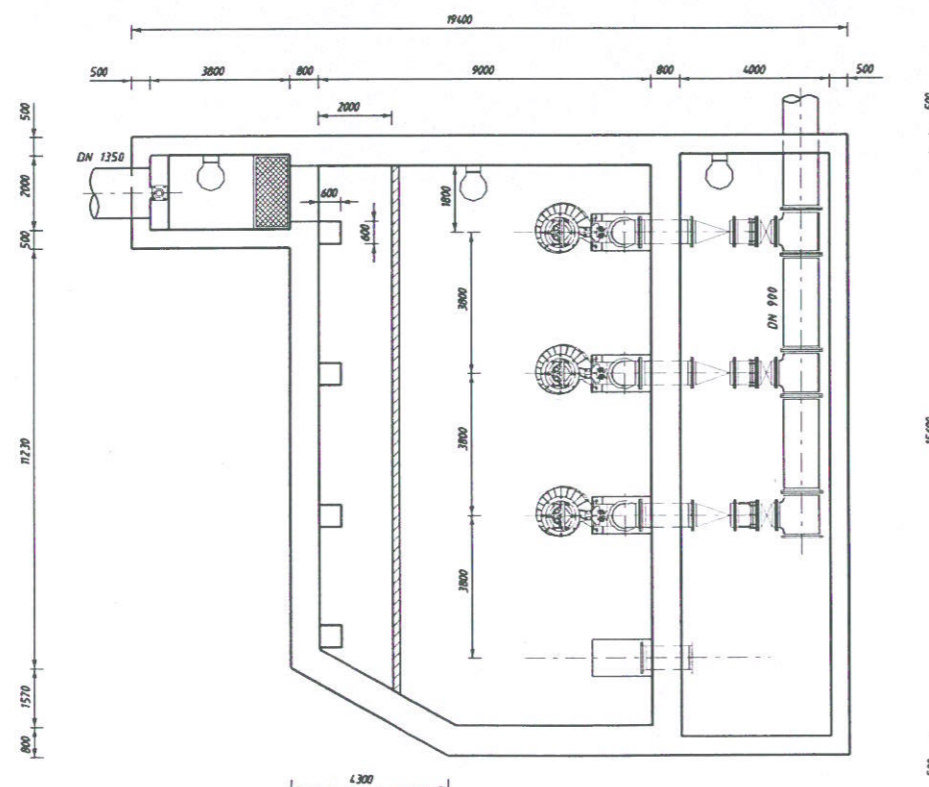
BASEMENT PLAN
