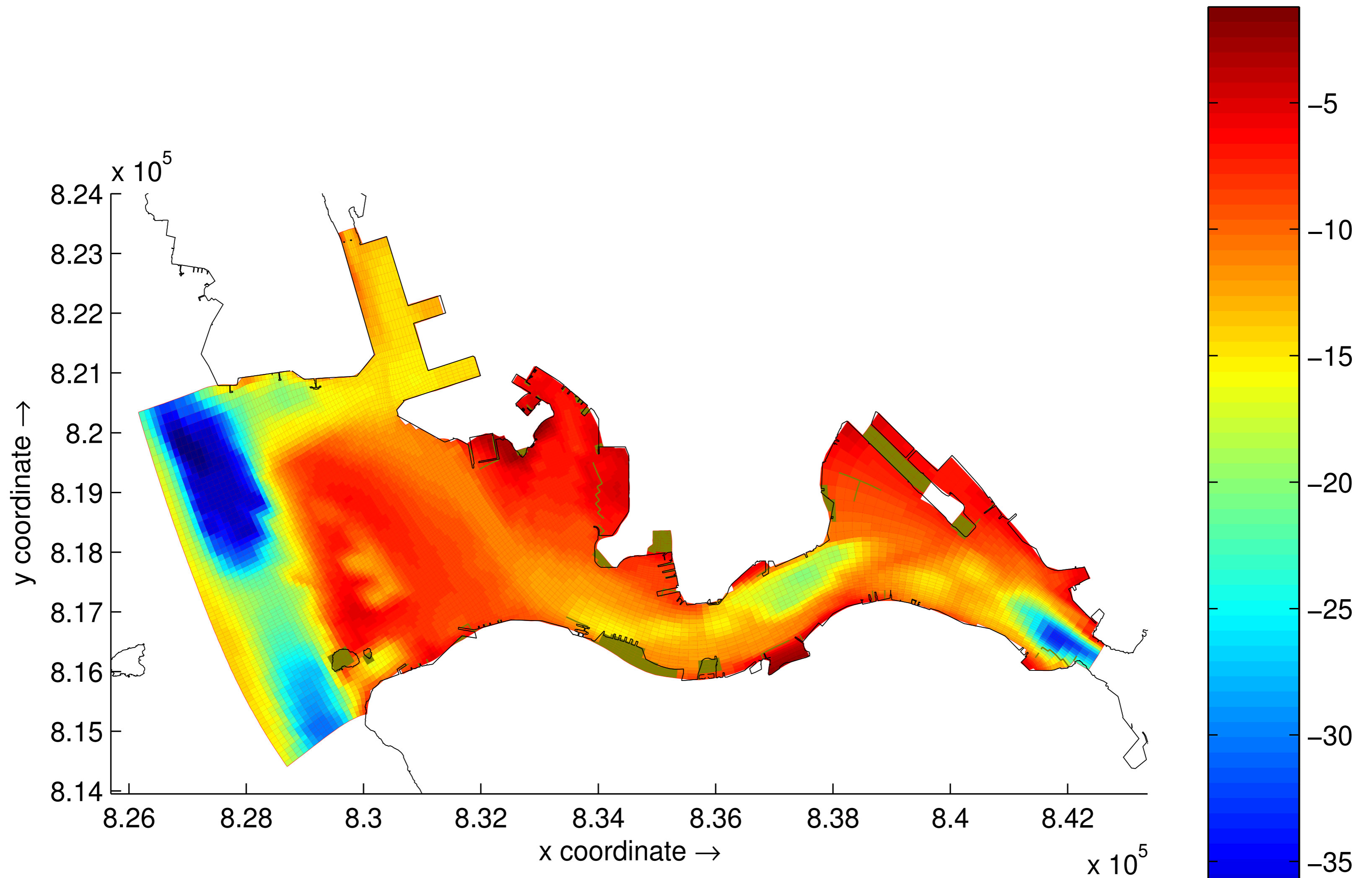
Figure 3.8b Bathymetry in the Victoria Harbour
