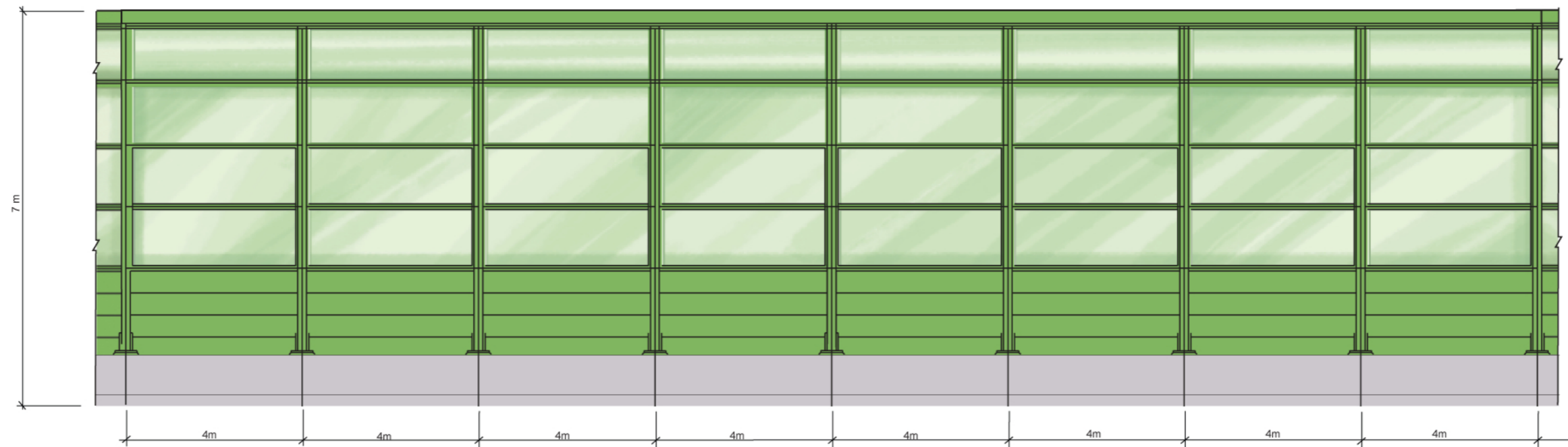
Facade Design Option 7 Reflective and Absorptive Panels
