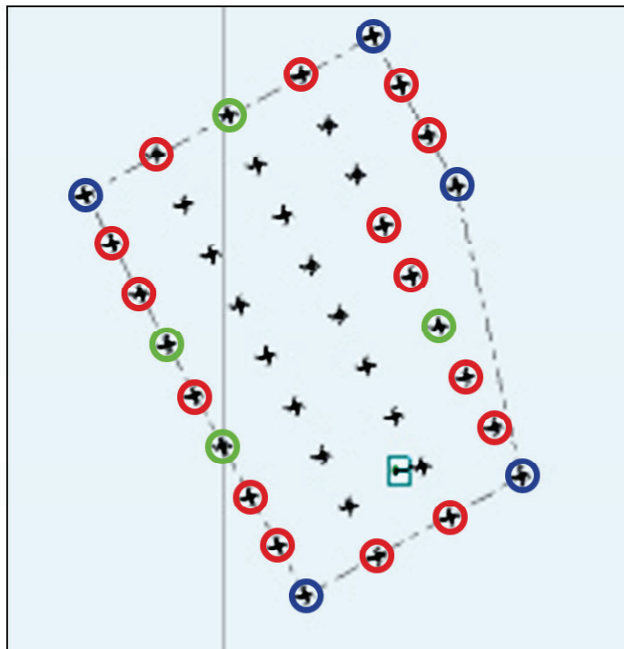
5MW LAYOUT
