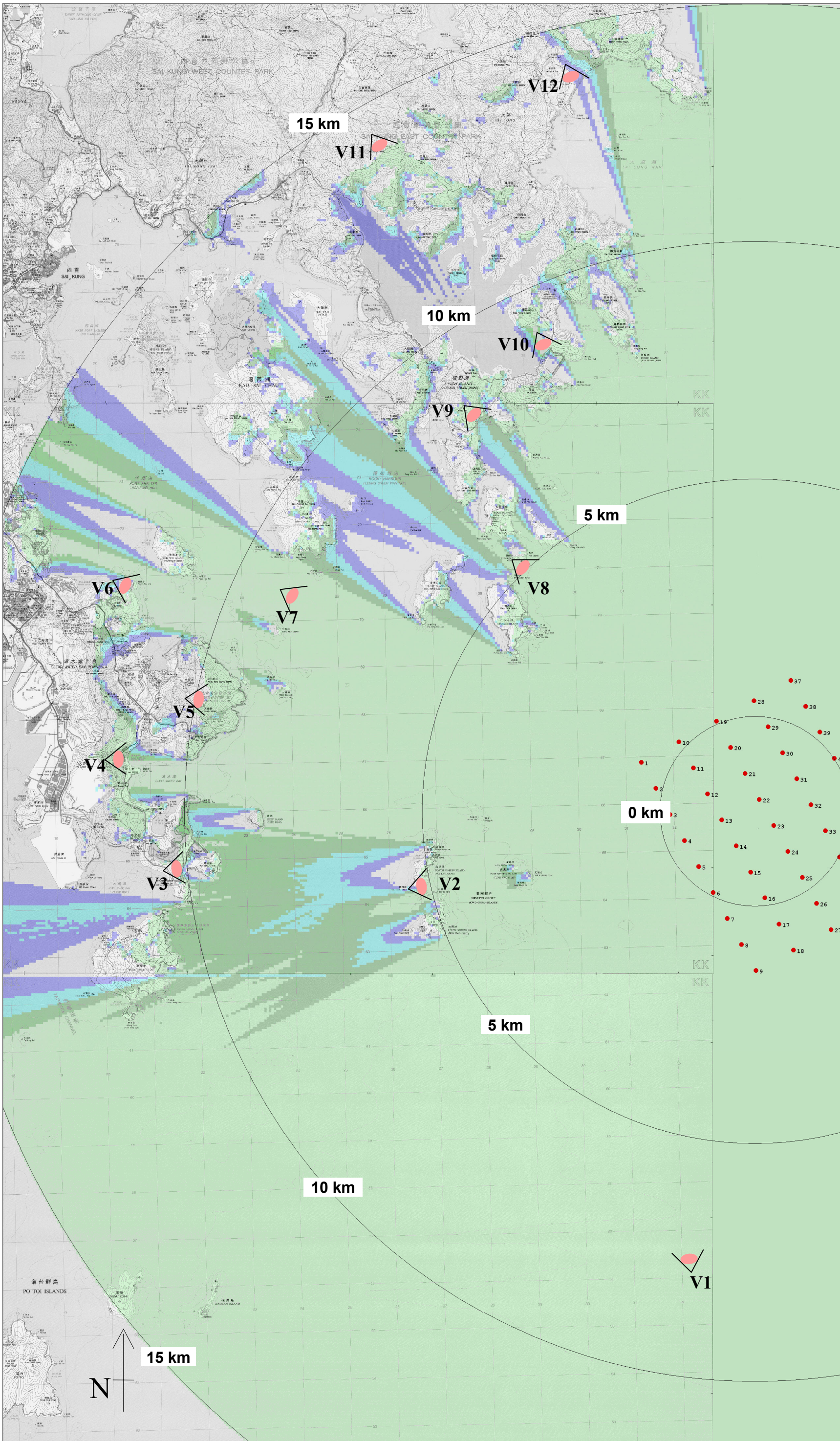
Figure 10.7b 5MW Option Viewpoints and ZVI to Blade Tip
