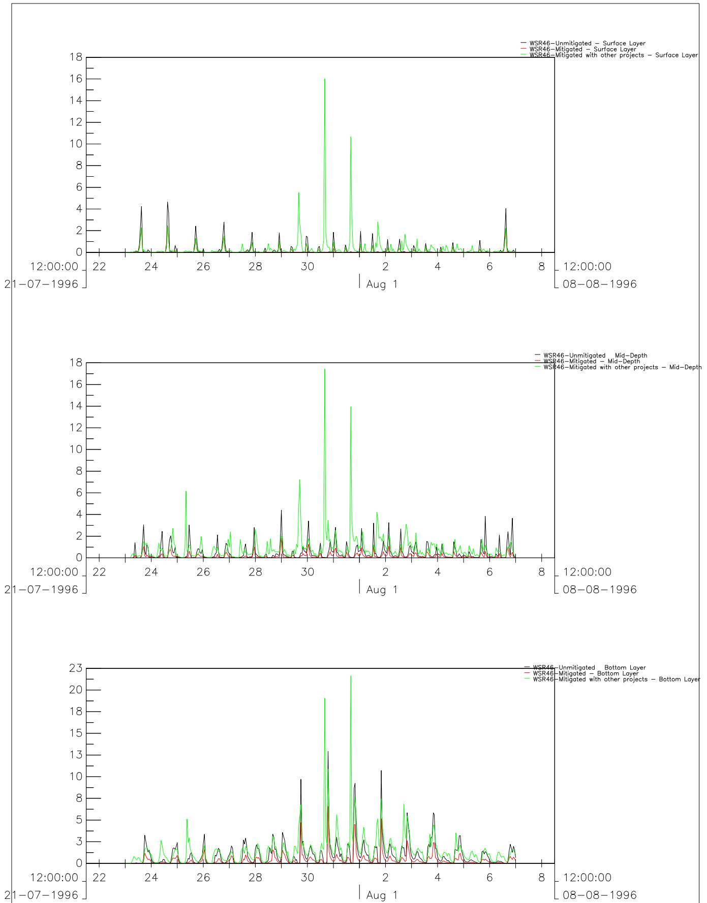
Year 2011 Time History Plots of the SS (mg/L) at WSR46, Wet Season (Top: Surface Layer; Middle: Mid-Depth; Bottom: Bottom Layer)
