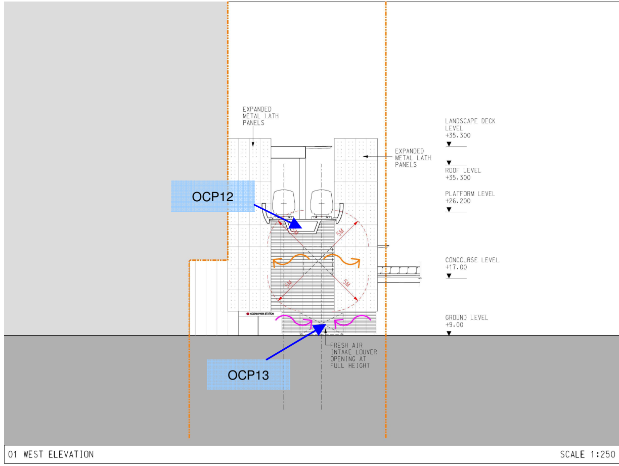
West Elevation
