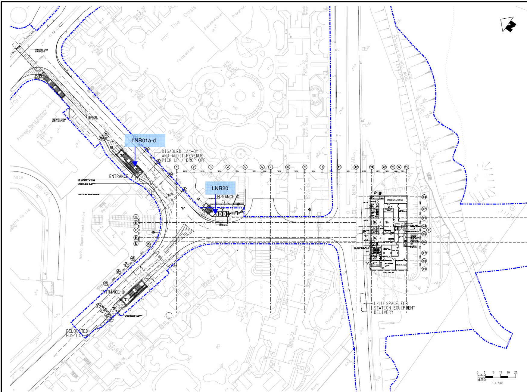
South Horizons Station Entrances A and C
