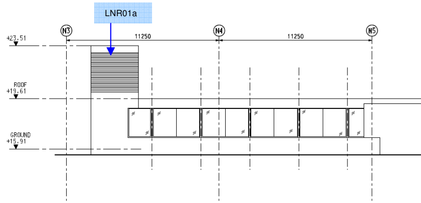
ELEVATION 2 SCALE
