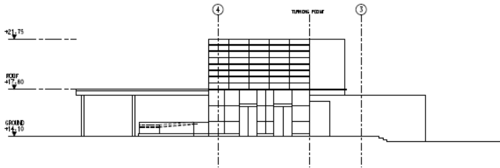
ELEVATION 9 SCALE
