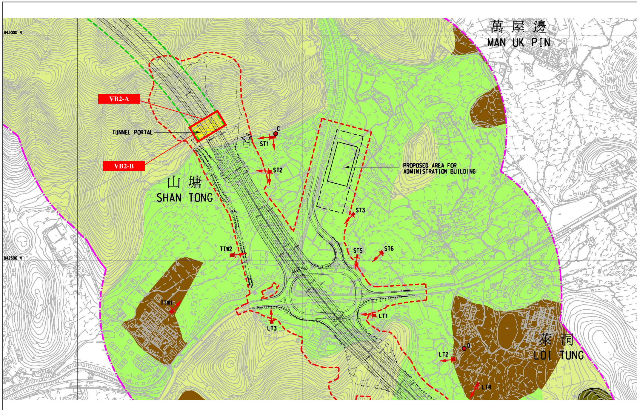
Figure 4.21.3 Fixed Plant of North Tunnel South Portal
