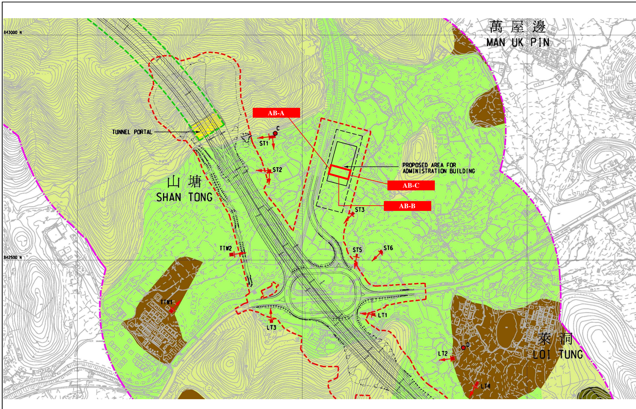
Figure 4.21.4 Fixed Plant of Administration Building
