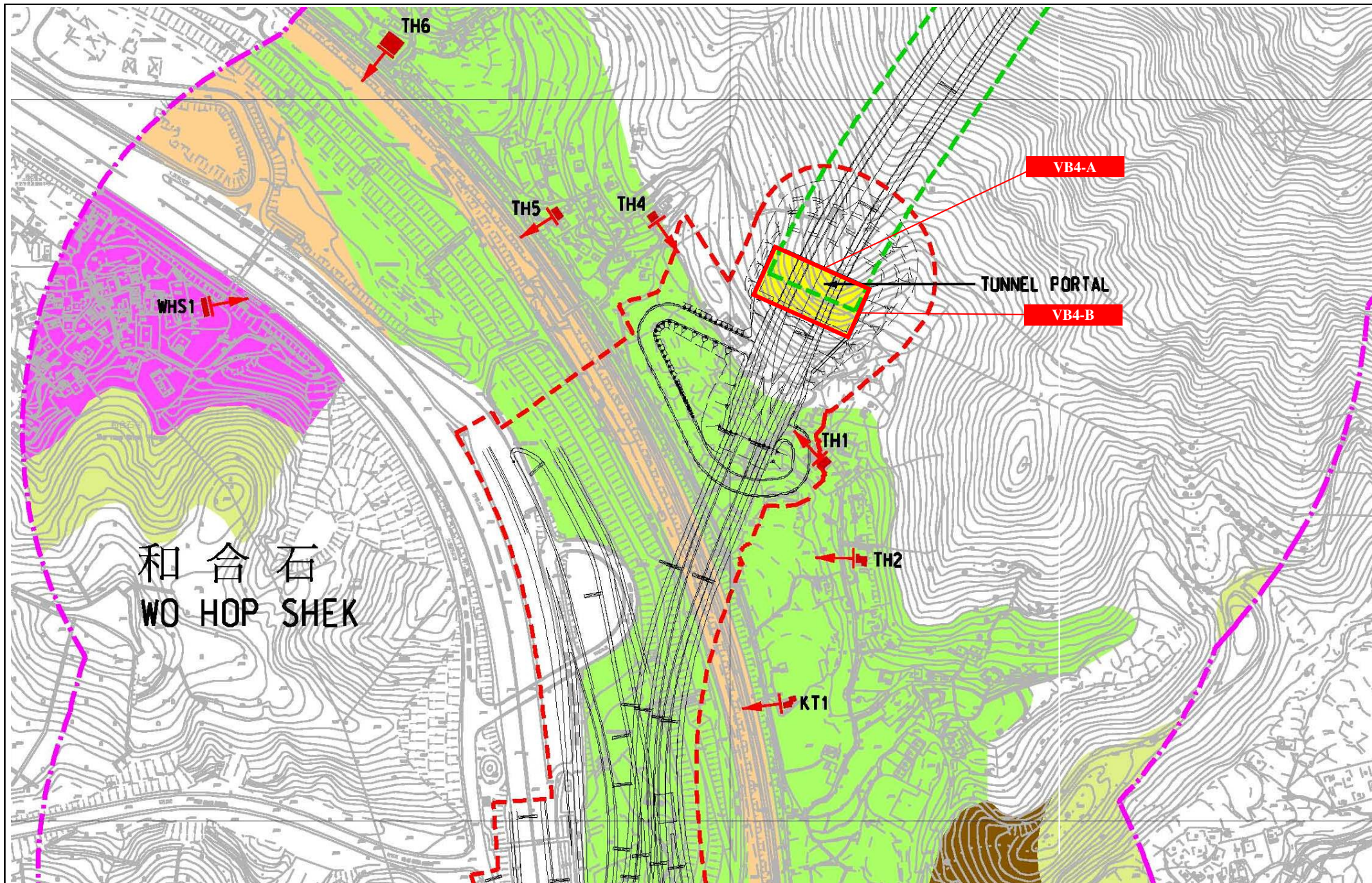
Figure 4.21.7 Fixed Plant of South Tunnel South Portal
